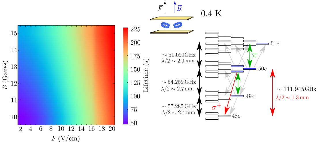
FIGURE II.12 The lifetime per atom is calculated inside an ideal inhibiting capacitor at 0.4 K. The plot is done for a pair of |50c\rangle atoms at a 5\text{ }\mu\text{m} distance as a function of the electric and magnetic fields. The individual atom populations is schematically represented by the opacity in the level drawn in the diagram on the right. The colored arrows depict the main transition limiting the lifetime in the capacitor. The light gray arrows show some relevant \sigma transitions that are suppressed by the capacitor. Absorption of photons with \Delta n = 2 are negligible at low temperatures.
