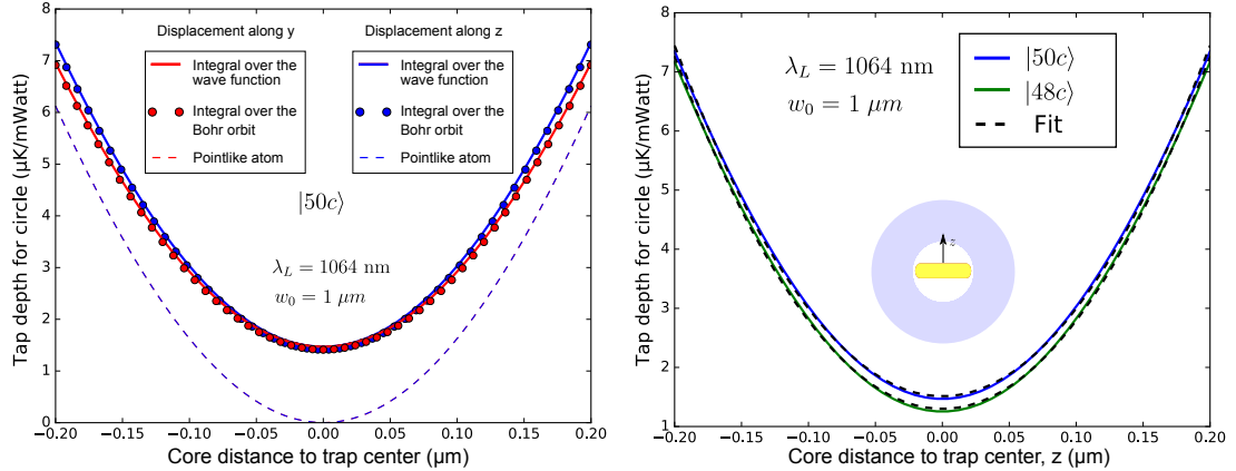
FIGURE C.2 Strongly focused LG beam ( w_0 = 1 \text{ } \mu\text{m} ). (a) Quasi-harmonic potentials along the y (red) and z (blue) directions for state |50c\rangle . The solid lines correspond to the full wavefunction average of the potential. The dots correspond to the Bohr orbit approximation and the dashed lines correspond to the point-like atom picture. (b) Potential along the z direction for states |48c\rangle and |50c\rangle . The blue ring represents the LG profile.
