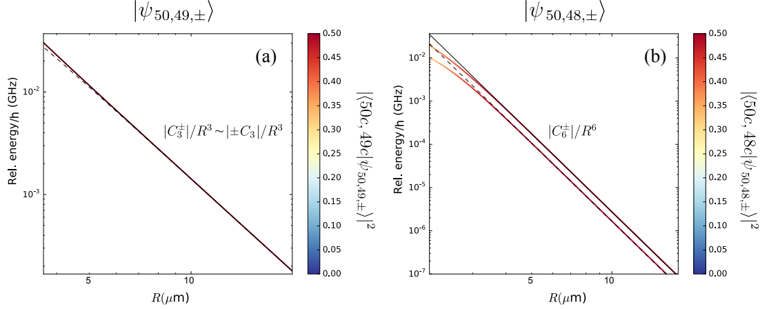
FIGURE I.6 Absolute value of the interaction energy as a function of position for interacting circular atoms. We show the energy dependence of the pair |\psi_{50,49,\pm}\rangle (a) and |\psi_{50,48,\pm}\rangle (b) with the interatomic distance R . The color bar represents the proportion of the product states to the eigenstate. For the pair of levels 50c - 49c ( \Delta n = 1 ) the direct dipole term dominates the interaction ( 1/R^3 ). For the pair 50c - 48c ( \Delta n = 2 ) the van der Waals ( 1/R^6 ) interaction dominates. In both plots (a) and (b), the solid black line fits the energy for the anti-symmetric superposition and the dashed line fits that of the symmetric superposition for R > 5 \mu\text{m} .
