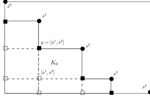
Figure 2.3.3: Knee points are the maximal elements obtained by the meet of d unsat points. The meet [s^1, s^2] is maximal and therefore defines a knee point g , whereas [s^1, s^3] does not. Dimension two is a degenerate case, since knee points are easily computable by taking the meet of any two unsat successors: in our example knee points correspond to [s^0, s^1] , [s^1, s^2] , [s^2, s^3] , and [s^3, s^4] . In arbitrary dimension generating knee points is not trivial.
