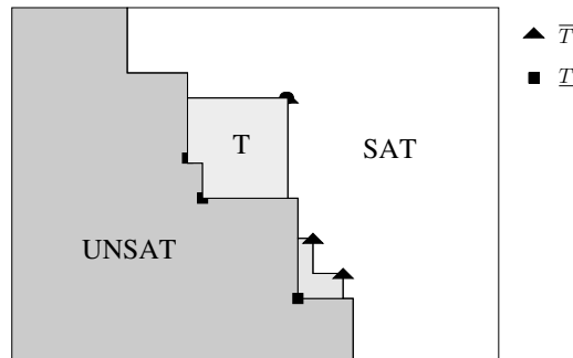
Figure 2.6.1: A partition between the sat , unsat and timeout parts of the cost space respecting property 2.6E.
