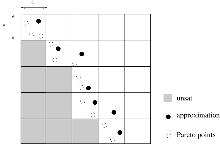
Figure 2.2.3: \epsilon -approximation with the grid.
