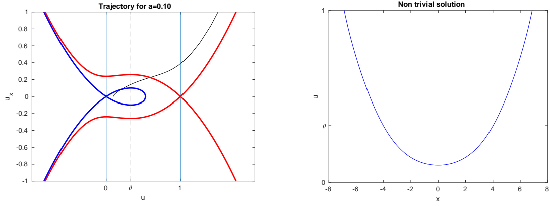
Figure 5.4 – \sigma = 40 and f(s) = s(1-s)(s-\theta) , \theta = 0.33 . Phase portrait (Left): the trajectory corresponding to the nontrivial solution is in black, the energy set \{\mathcal{E} = F(1)\} in red, the energy set \{\mathcal{E} = F(0)\} in blue. Nontrivial solution of (5.11) (Right).
