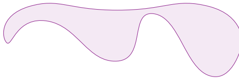
Figure 5.3 – A domain with a large eigenvalue, for which constrained boundary control enables us to control the population to an intermediate trait.
