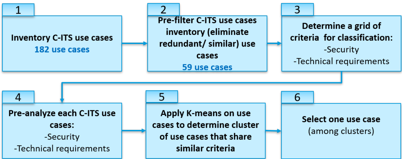
Figure 4.5: Classification methodology
