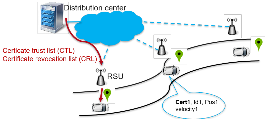
Figure 4.4: CRL/CTL reloading
