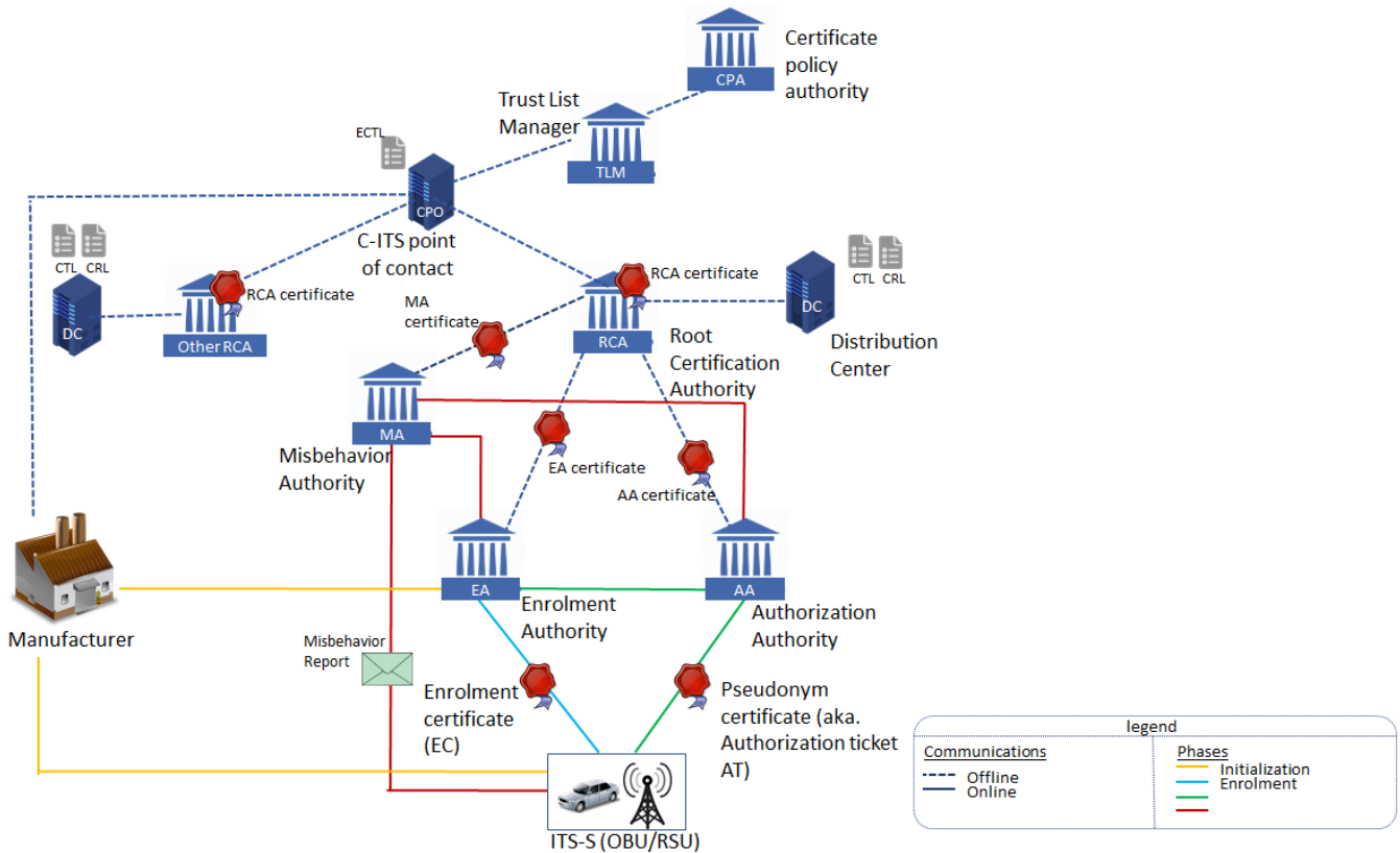
Figure 3.4: ETSI PKI Architecture
