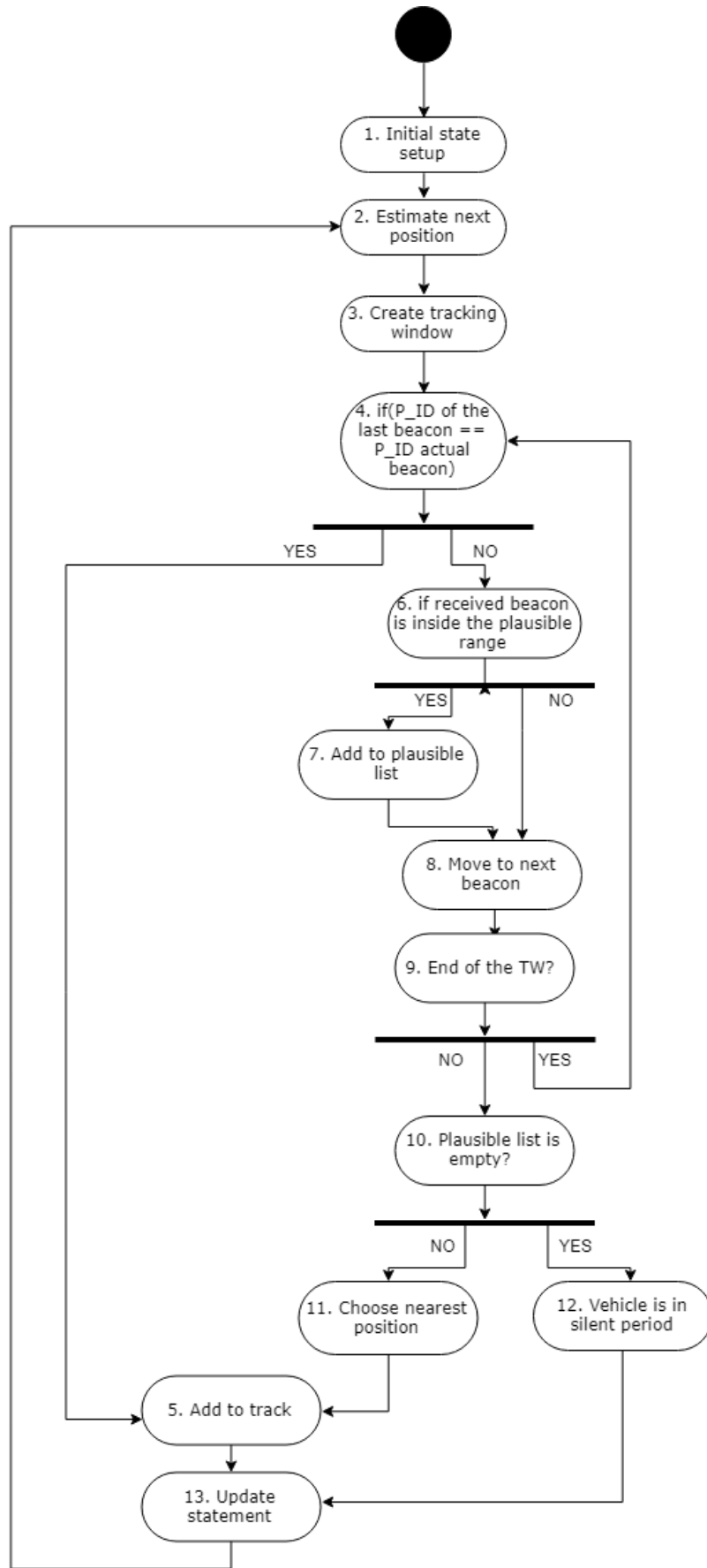
Figure 6.22: Tracking algorithm
