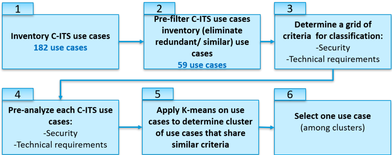
Figure 4.5: Classification methodology
