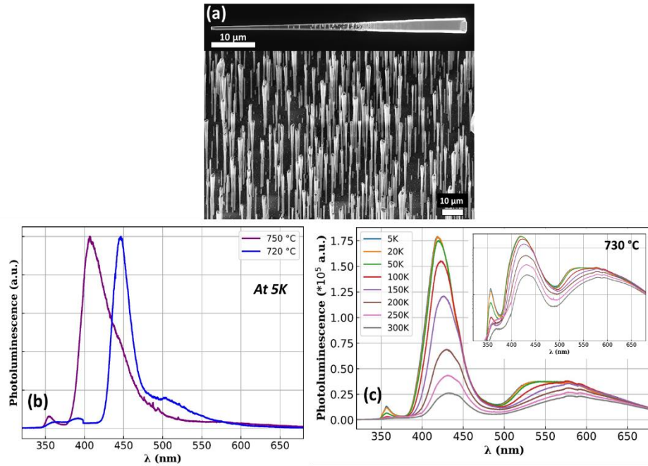
Figure 3.2: (a) SEM image of as-grown wires for sample with InGaN QWs grown at 720 °C with single wire SEM image at the top-inset (#T2610), (b) Low temperature photoluminescence (PL) spectra for samples with QWs grown at 720 °C and 750 °C (#T2400), (c) Temperature-dependent PL for additional sample with QW grown at 730 °C (#T2548).
