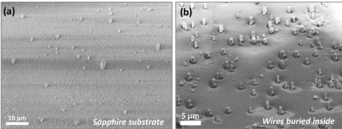
Figure 5.4: SEM images after PDMS peeling off: (a) titled at 30° showing the surface of sapphire substrate and (b) tilted at 45° showing n-GaN wire bottoms protruding out of the PDMS layer after RIE etching.
