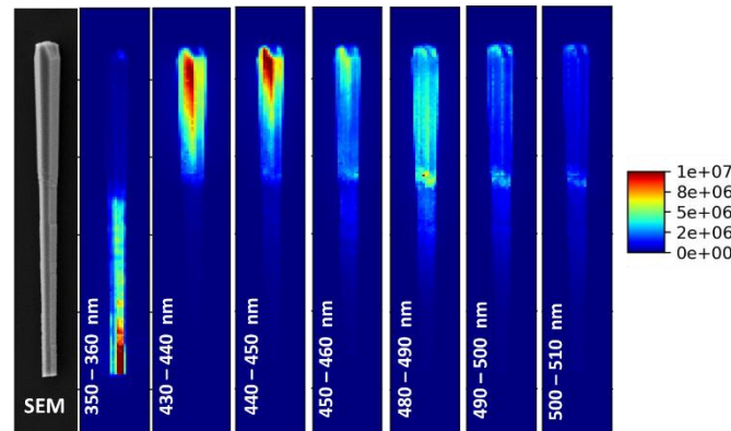
Figure 3.15: CL-mapping of single wire at 4 K for different wavelength emission with SEM image at extreme left.
