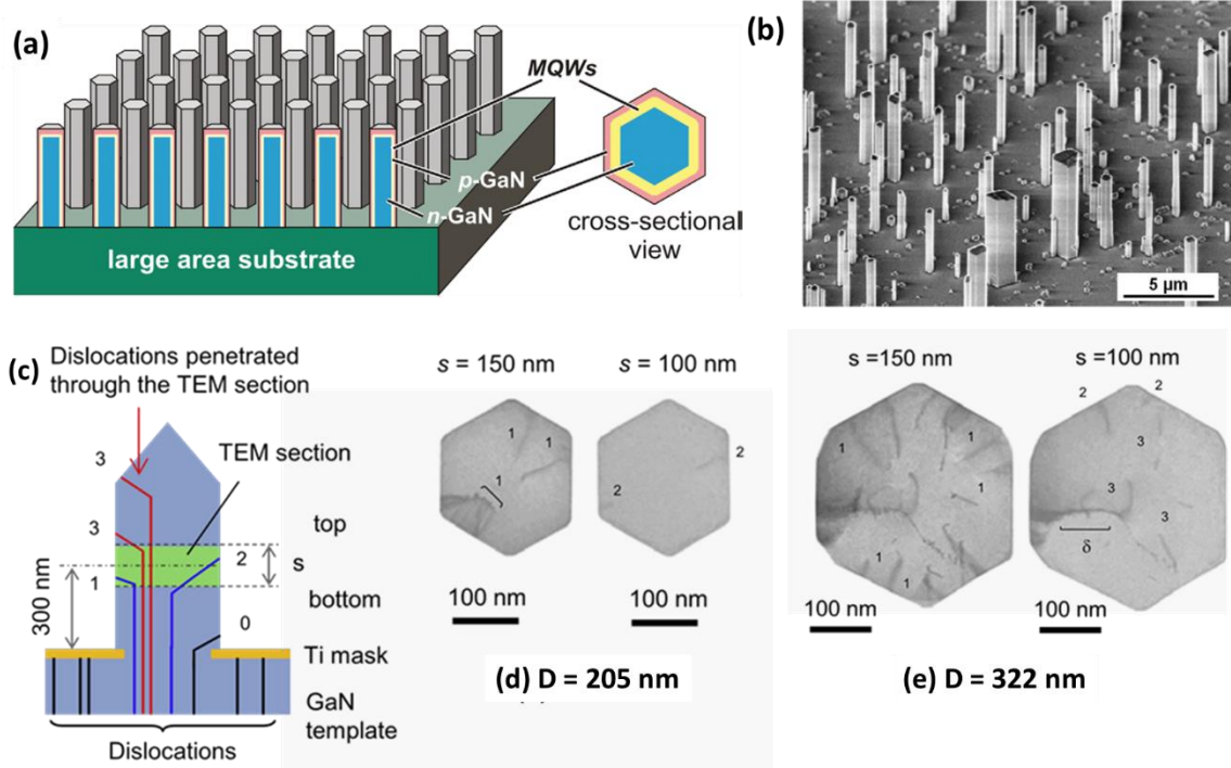
Figure 1.10: (a) Taken from Ref. 68: Schematics of core-shell geometry for InGaN/GaN based LED; (b) Adapted from Ref. 56.: SEM view of typical self-assembled GaN wires grown on c -plane sapphire substrate; (c-e) Taken from Ref. 62: Schematic diagram of dislocations propagating in a TEM section in (c), magnified plan-view TEM images of nanocolumns with diameters D = 205 nm in (d) and D = 322 nm in (e). Note the nanocolumns are sliced horizontally to a thickness of s at a height of \sim 300 nm above their bottoms.
