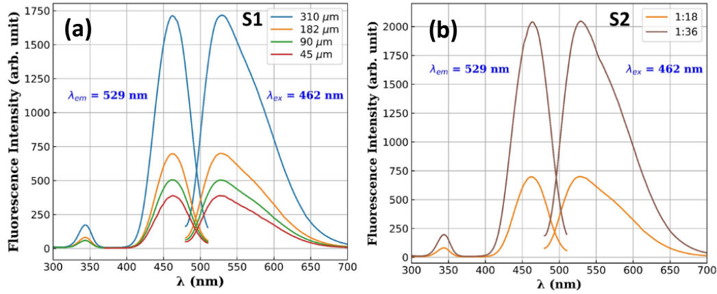
Figure 5.20: Excitation-Emission spectra of phosphors dispersed in PDMS mixture: (a) series S1 with mixing ratio 1:18 and varying thickness; (b) series S2 with thickness 182 µm and varying mixing ratio.
