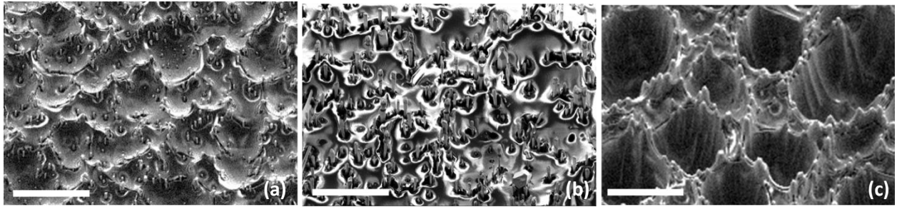
Figure 5.1: SEM images tilted at 30^\circ illustrating the top part of the wires protruding out of the photoresist for wires having length: (a) 25 (\pm 5) \mu\text{m} , (b) 45 (\pm 5) \mu\text{m} and (c) 85 (\pm 5) \mu\text{m} respectively. Scale bar in the SEM image corresponds to 50 \mu\text{m} .
