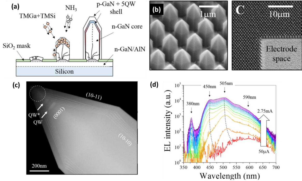
Figure 1.13: Taken from Ref. 86- (a) Schematics of the InGaN/GaN SAG nanorod containing n-GaN core, 5 InGaN QWs & a p-GaN shell observed with the SEM images shown in (b), (c) STEM image of the core-shell layers structure and (d) Room-temperature EL spectra recorded at different injection currents.
