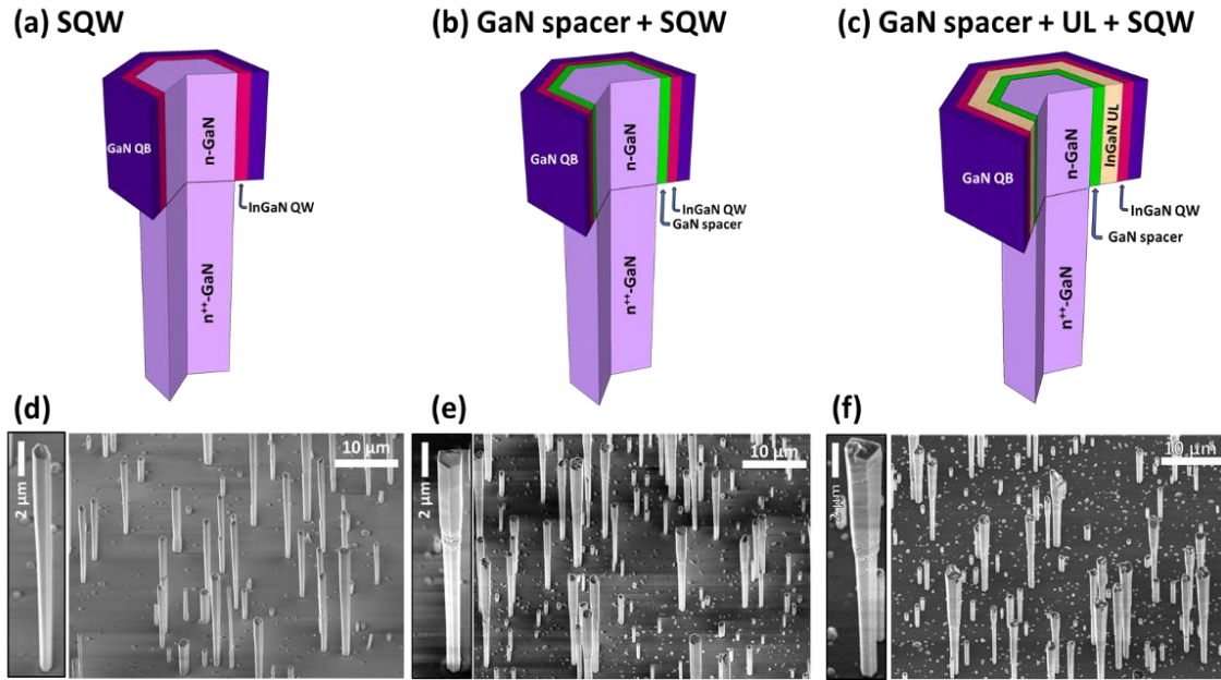
Figure 4.1: Schematics of the three core-shell heterostructures grown on \bar{c} -oriented GaN wires: (a) #1 InGaIn single quantum well (SQW), (b) #2 with the addition of a GaN spacer prior to SQW, (c) #3 with the adding of an InGaIn under-layer (UL) between the GaN spacer and the SQW. 30°-tilted SEM images of as-grown wires: (d), (e) and (f) corresponds to (a), (b) and (c) heterostructures respectively along with enlarged views on single wires. (#1: T2628, #2: T2594, #3: T2597)
