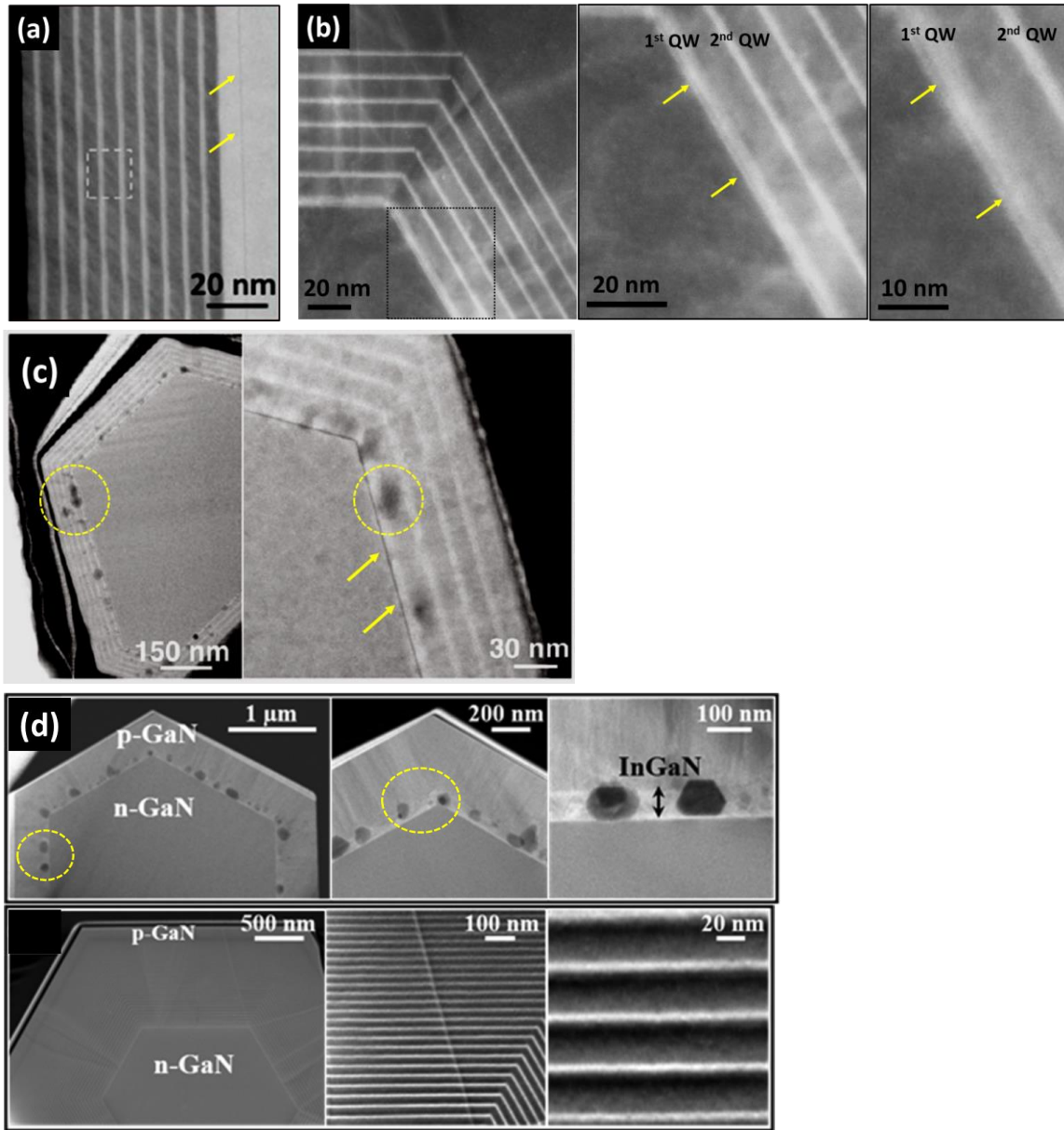
Figure 4.7: Previous results on structural characterization using STEM-HAADF images- (a) Adapted from Ref. 32 : Longitudinal cross-sectional view taken along [11\bar{2}0] zone-axis with MQWs on the wire sidewalls; (b) Adapted from Ref. 35 : Transversal cross-sectional images taken along the c -zone axis depicting the 7x QWs separating the core and p-GaN (left image) with corresponding zoomed images of the first two QWs (right images); (c) Adapted from Ref. 33 : Similar orientation of wire slice as (b) but without p-GaN; and (d) Adapted from Ref. 34 : Cross sectional images of a wire with 60 nm \text{In}_{0.1}\text{Ga}_{0.9}\text{N} shell (top image) and a wire with 30\times \text{In}_{0.18}\text{Ga}_{0.82}\text{N}/\text{GaN} MQWs shell (image below).
