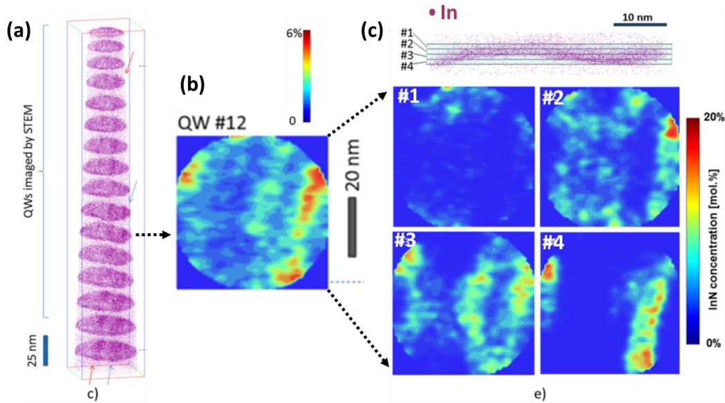
Figure 2.7: (Adapted from Ref. 14) Atom probe tomography measurements. (a) 3D reconstruction of the In-atom distribution in a wire slice, oriented along the [0001] zone axis but tilted to show the non-uniform In-distribution within the QW planes, (b) 2D-mapping of the in-plane fraction of InN calculated through 8 nm thick box of QW #12; and (c) InN fraction maps within 1 nm thick slices of QW #12 as shown in the upper part of the figure.
