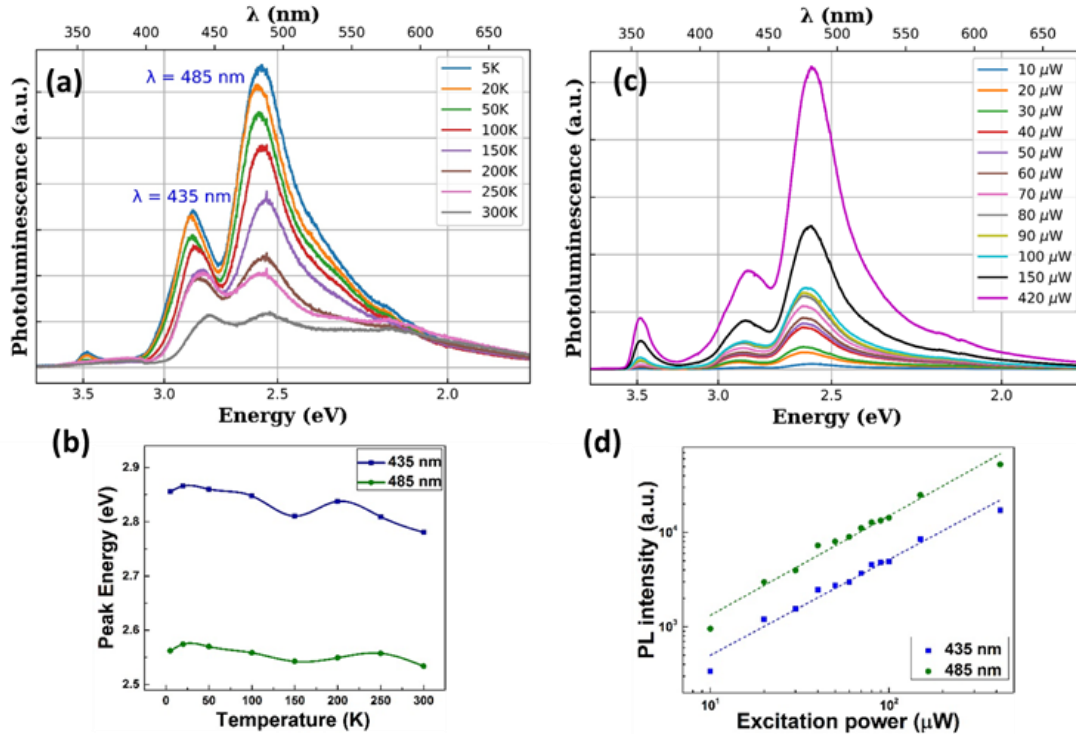
Figure 3.14: Photoluminescence (PL) measurement by exciting the wires with 244 nm laser: (a) temperature dependent PL (TDPL) spectra for a fixed laser power of 100 \mu W, (b) the temperature dependence of the PL peak positions for 435 and 485 nm contributions; (c) Excitation-power dependent PL (PDPL) spectra for a fixed temperature at 5 K, and (d) the power dependence of PL intensity for the two contributions.
