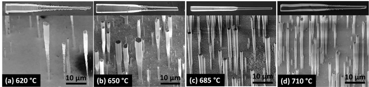
Figure 3.4: SEM images of as-grown wires with QWs grown at different temperatures: (a) 620, (b) 650, (c) 685 and (d) 710 ^{\circ}\text{C} . ((a) T2316, (b) T2313, (c) T2314, (d) T2315)) (Ref. 17)
