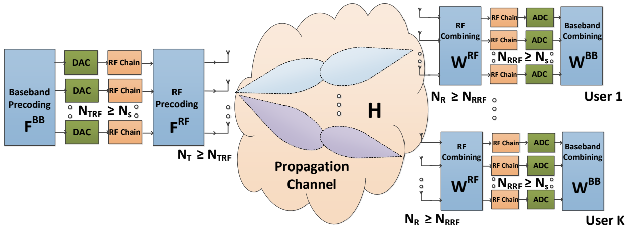
Figure 2.7: The MU MIMO Hybrid Beamforming Architecture
