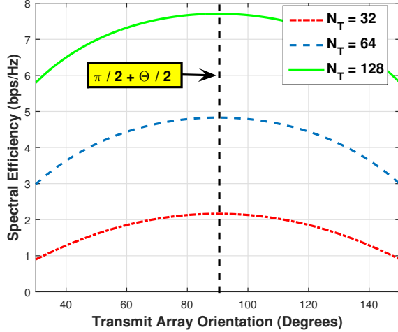
1) SE versus the ULA transmit array orientation for a given scenario ( N_R = 2, \rho = 10\text{dB}, d_r = 18\lambda, D = 5000\lambda ) in pure LoS environment.
