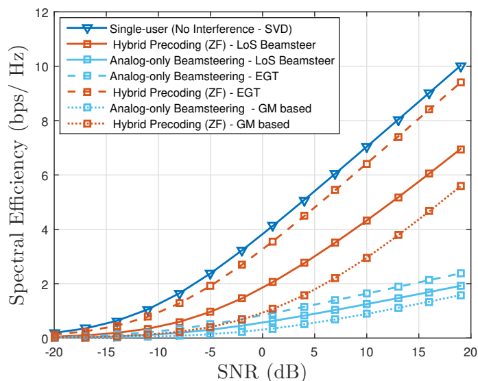
Figure 4.6: The effect of the random path blockage on different analog and hybrid beamforming approaches in terms of the SE
