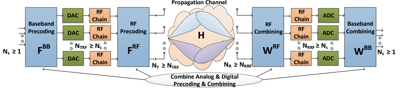
Figure 2.6: The Hybrid Beamforming Architecture
