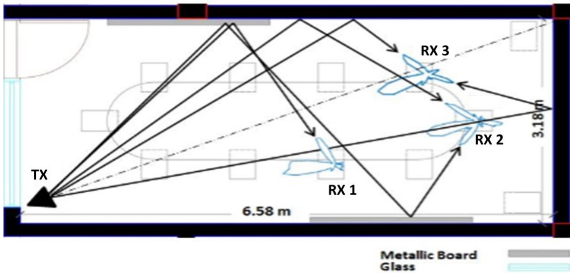
Figure 3.4: Meeting room plane with applying ray tracing.
