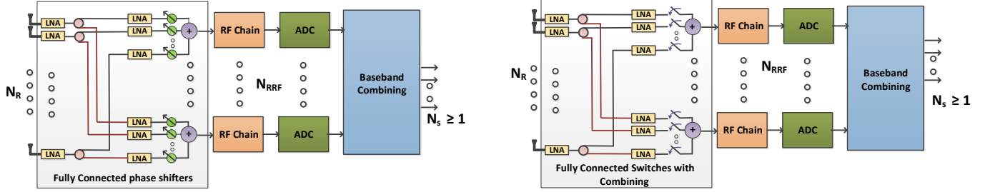
1) Fully Connected Analog Architecture with Phase Shifters
