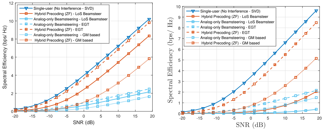
(a) Comparison between different analog and hybrid beamforming approaches without blockage in terms of the SE. (b) The effect of the LoS path blockage on different analog and hybrid beamforming approaches in terms of the SE.
