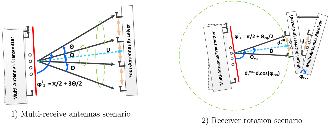
Figure 5.3: Illustration of the correlation minimization approach adopted for the RSM mmWave framework for multiple paths and multiple orientations of the receiver
