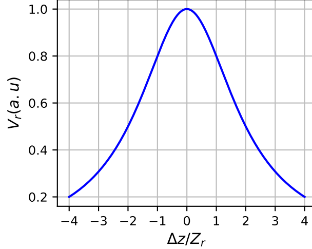
Figure VII.8: Laser wavefront rotation velocity as a function of the defocusing distance \Delta z for \xi = \xi_{max} in arbitrary units.
