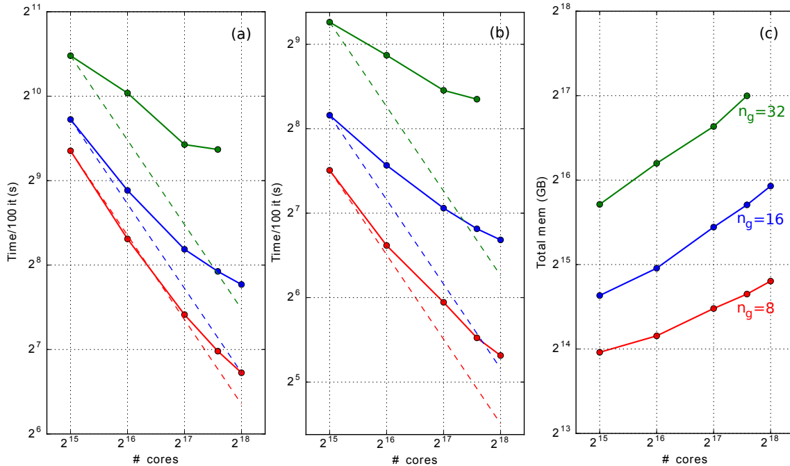
Figure V.5: Evolution of strong scaling and memory consumption (grid quantities) of the pseudo-spectral PIC algorithm for different number of guardcells n_g ( n_g = 8 : red, 1n_g = 16 : blue, n_g = 32 : green) on Cray XC40 THETA cluster at ALCF (using 32768-262144 cores) with one OpenMP thread per MPI task. The FFTs are computed using the Intel MKL library which is more efficient on Intel architectures than FFTW. The simulation box consists in a homogeneous plasma with one particle per cell for both electrons and ions. The grid size is 240 \times 6144 \times 12288 grid cells. Panel (a) represents the scaling of the full PIC loop. Panel (b) represents the scaling of the pseudo-spectral solver only, including MPI-exchanges for grid quantities. Panel (c) represents the total memory consumption of grid quantities (i.e. field quantities).
