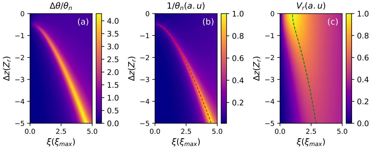
Figure VII.20: Panel (a): Evolution the angular separation ratio \frac{\Delta\theta}{\theta_n} as a function of the laser defocusing length and the pulse-front tilt \xi . Panel (b): the evolution of 1/\theta_n (in arbitrary units) as a function of the laser defocusing length \Delta z and the pulse-front tilt \xi . The dashed red line highlights the pulse-front tilt that minimizes the harmonic divergence at a given defocusing distance \Delta z . Panel (c): the evolution of the wavefront rotation velocity as a function of the pulse-front tilt amount and the defocusing distance. The dashed green line highlights the pulse-front tilt amount that maximizes the laser wavefront rotation velocity for a given defocusing distance \Delta z . In all panels, we assumed a laser incidence angle of 55^\circ and a plasma density scale length of L = \lambda_0/15 .
