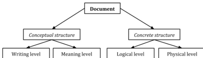
Fig. 5.3 Document structures
