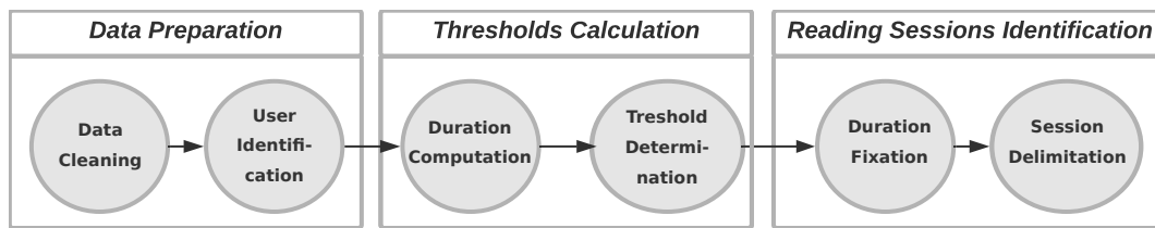
Fig. 6.4 Steps for computing reading sessions from learners' log data
