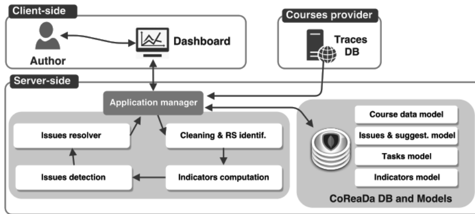
Fig. 7.3 Architecture of CoReaDa
