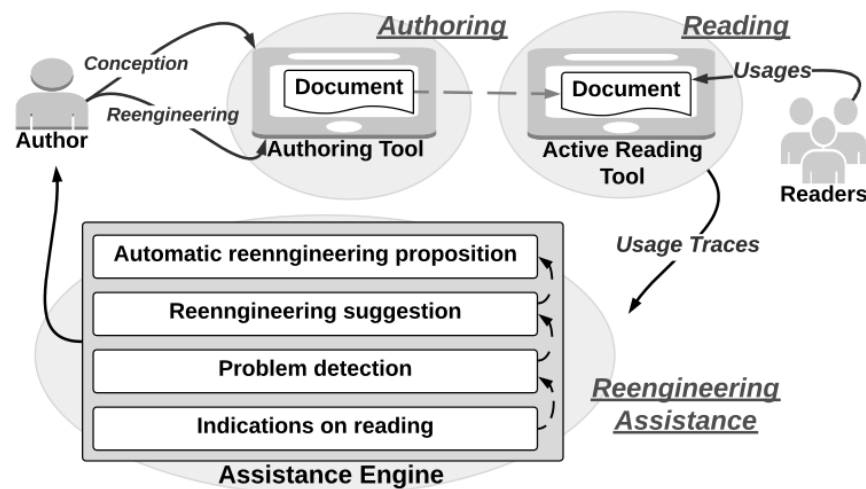
Fig. 5.2 Overview of the usage-based reengineering framework
