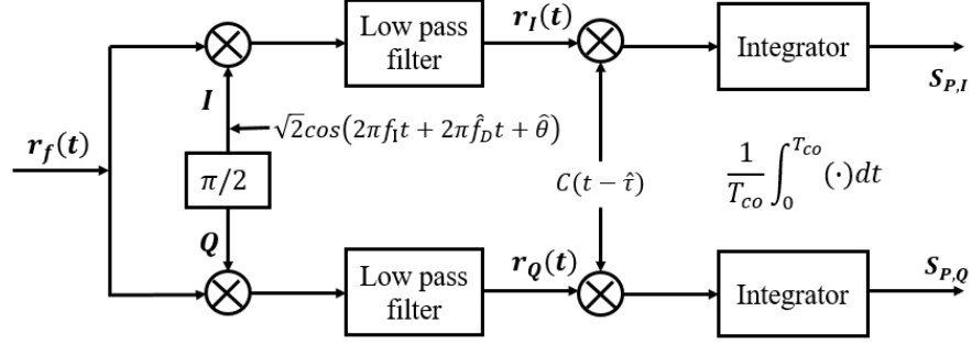
Figure 2-11. Signal acquisition
