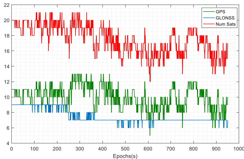
Figure 5-12. Number of tracked satellites during Data set 1. No elevation or C/N0 value mask is applied.
