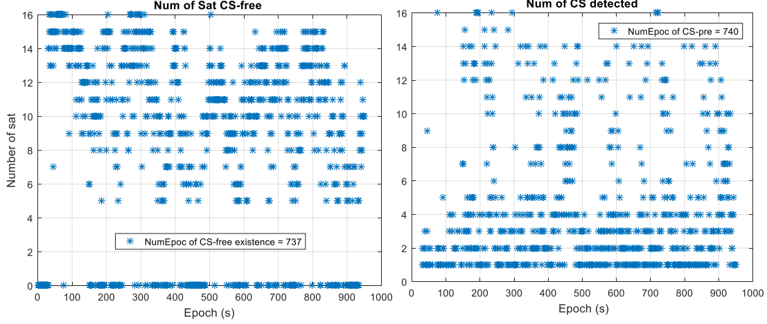
Figure 5-35. Data set 1. Number of epochs holding satellites declared CS-free(on the left), and Number of epochs holding satellites declared CS- deteriorated (on the right). CS-DR scheme takes the values (\alpha_1, \alpha_2, N_{cs}) = (0.003, 0.5, 10) .
