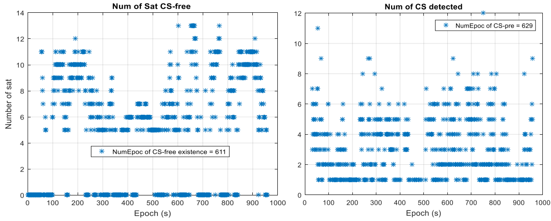
Figure 5-37. Data set 2. Number of epochs holding satellites declared CS-free(on the left), and Number of epochs holding satellites declared CS- deteriorated (on the right). CS-DR scheme takes the values (\alpha_1, \alpha_2, N_{cs}) = (0.003, 0, 10) .
