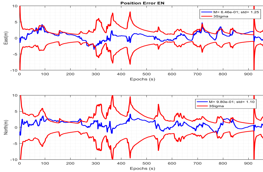
Figure 5-40. Horizontal Float GNSS (GPS+GLONASS) position difference between estimated trajectory and the reference trajectory (Data set 2) with associated environment type chosen as 'Rural'. CS-DR scheme takes the values (\alpha_1, \alpha_2, N_{cs}) = (0.003, 0.5, 10) .
