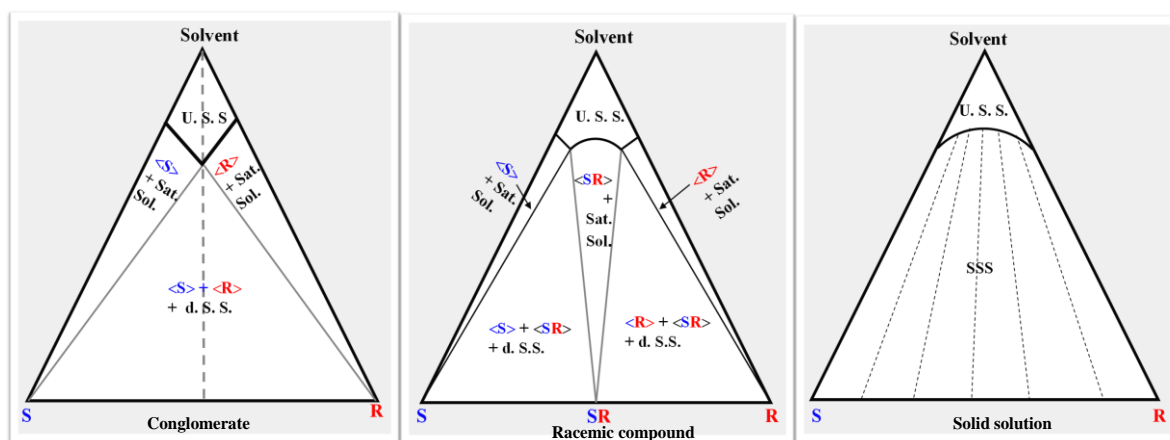
Figure 1.14: Fundamental types of ternary solubility phase diagrams for chiral systems in absence of partial solid solution and solid-solid transition (U.S.S. indicates under saturated solution; d.S.S.: double saturated solution and S.S.S.: indicates saturated solid solution).
