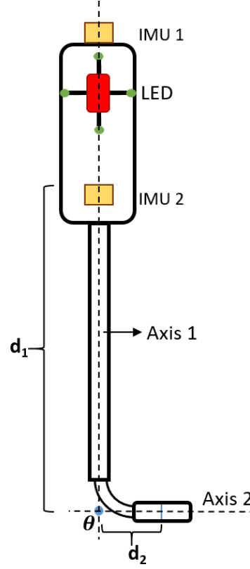
FIGURE 3.10: Schematic of the laparoscope
