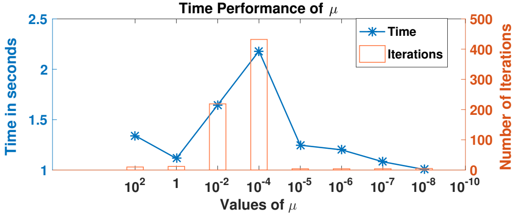
FIGURE 5.8: Average time performance while changing the regularization parameter. Left Y-axis: Average time taken by each iteration in 50 trials. Right Y-axis: Total number of iterations.
