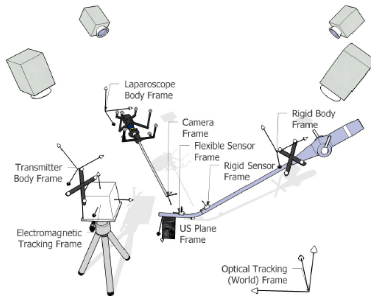
FIGURE 2.19: Electromagnetic sensors and camera based hybrid tracking system for US laparoscopes (Image from [Feu+07])
