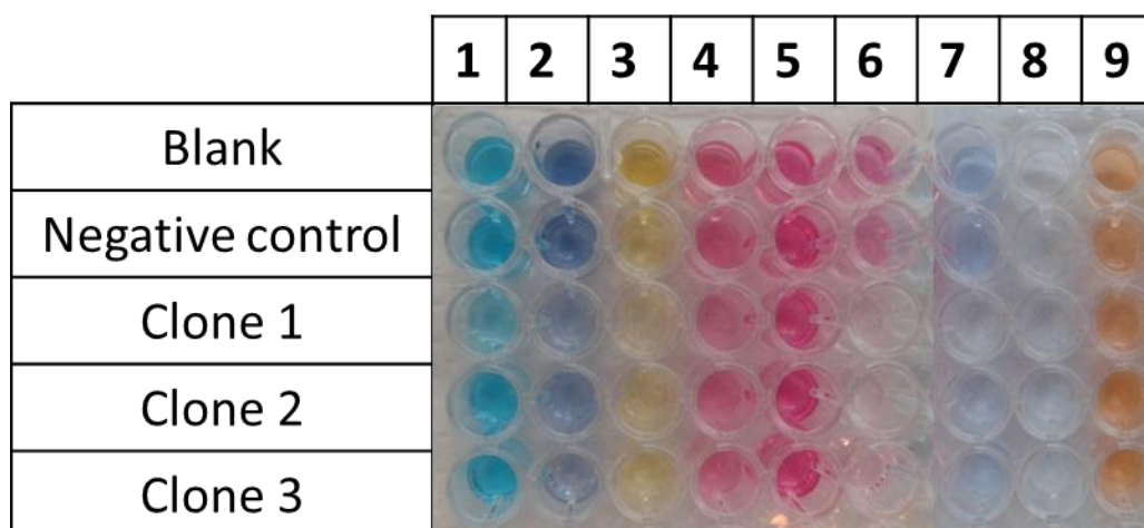
Figure 30 : Dye discoloration by the hit metagenomic clones. The pictures show the supernatants of the reaction media after 72h of reaction with enzymatic extracts. 1: Malachite Green; 2: Reactive Black 5; 3: Tropaeolin O; 4: Amaranth; 5: Acid Fuchsin; 6: Cibracon Brilliant Red 3BA; 7: Remazol Brilliant Blue R; 8: Indigo Carmin; 9: Reactive Orange 16
