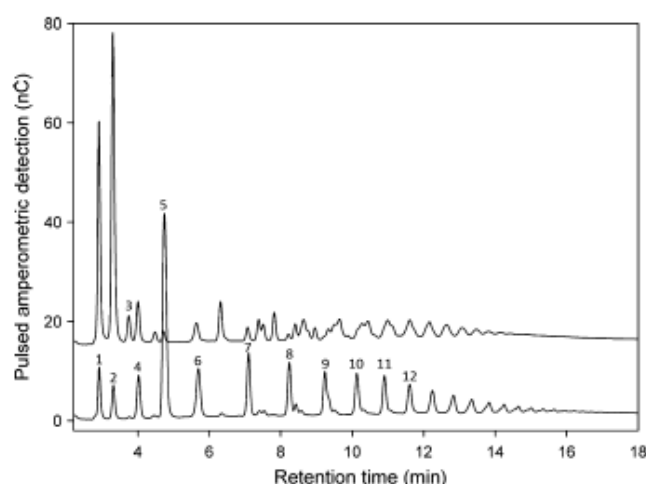
Fig. 5. HPAEC-PAD chromatograms of the acceptor reaction using sucrose (146 mM) and 1500 g·mol -1 dextran (33 mM) performed by BRS-A at 30 °C and pH 5.75. The bottom line represents the reaction at the initial time (1 min reaction time). The top line represents the reaction after 8 h, indicating \alpha -(1→2)-branched products formed from the dextran acceptor, as well as fructose and leucrose by-products: (1) glucose, (2) fructose, (3) leucrose, (4) isomaltose, (5) sucrose, and (6–12) isomalto-oligosaccharides with degrees of polymerization of 3–9, respectively.
