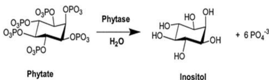
Figure 14: Mechanism of phytate hydrolysis by phytases (Mittal et al., 2011)
