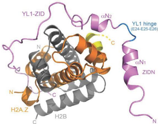
YL1-ZID-H2A.Z-H2B structure
