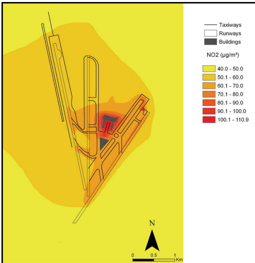
Figure 9-2: Contour plot of modelled total \text{NO}_2 concentrations ( \mu\text{g m}^{-3} ) around Beirut Airport (2012) ( z = 2 \text{ m} )
