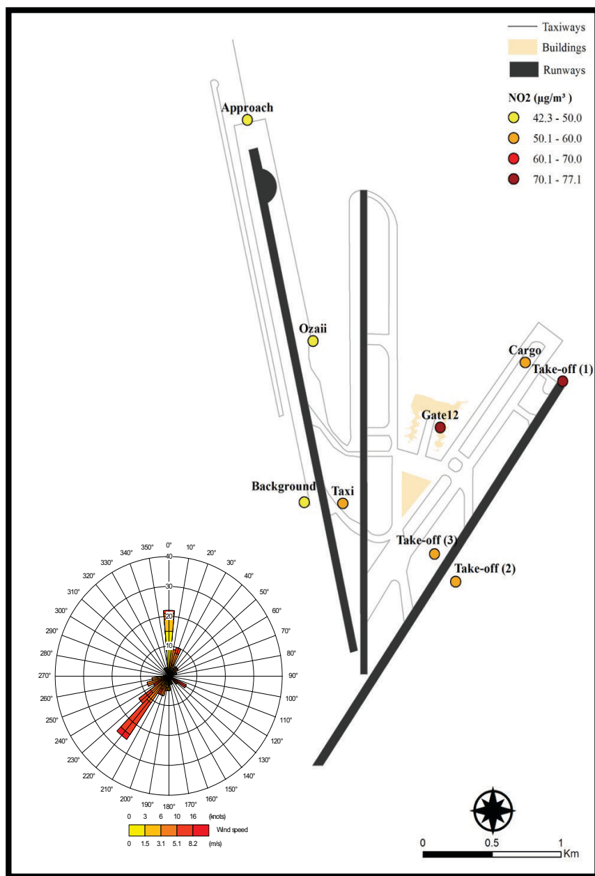
Figure 6-12: Measured \text{NO}_2 Concentrations ( \mu\text{g m}^{-3} ) at Beirut Airport (May 16-23, 2015)
