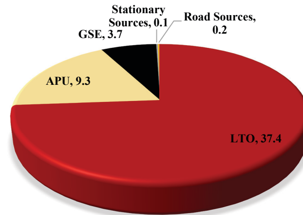
(a) NO 2 EMISSION INVENTORY (2012): 50.7 TONNES
