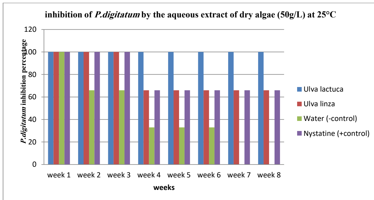
Figure 3: inhibition of P. digitatum by crude extracts of Ulva linza and Ulva lactuca ( 50 \text{ g L}^{-1} )
