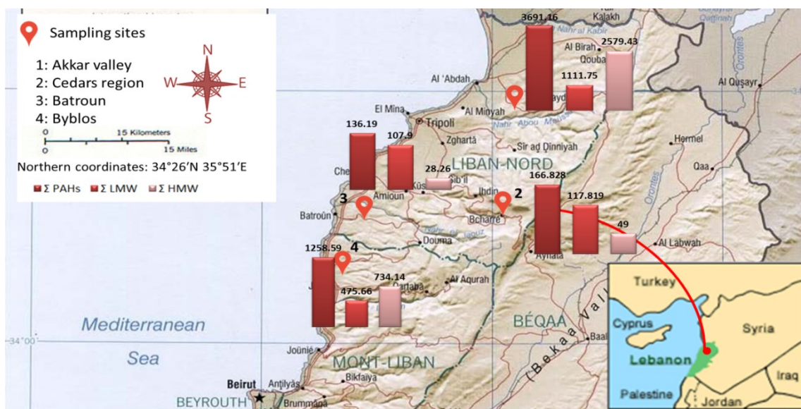
Figure 2: Distribution of PAHs in the different studied regions
