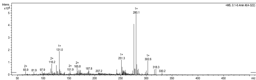
Fig. 5. Mass spectra for the positive peak of orange eluted with 80/20 of methanol/water.
