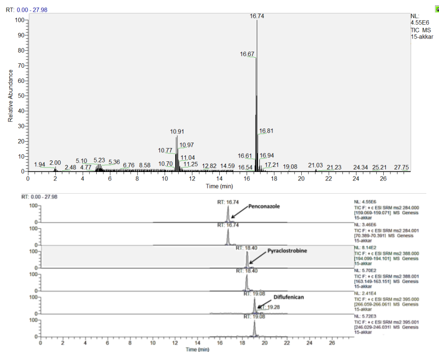
Figure 2: LC-MS/MS chromatogram of a sampling site in Akkar region
