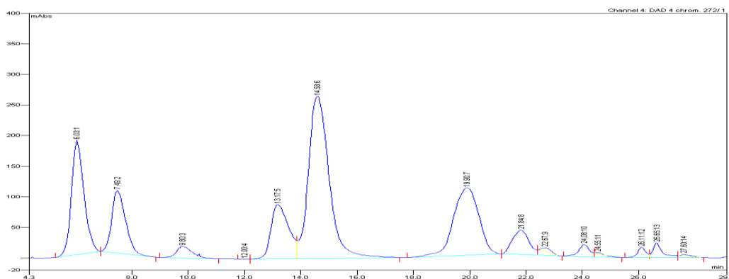
Figure 5s: Chromatogram of spiked apples
