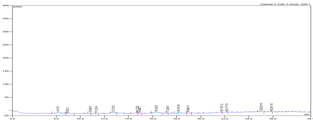
Figure 4s: Chromatogram of not spiked apples
