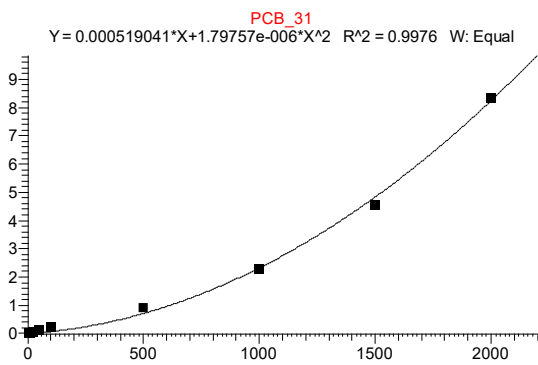
Figure 1s: Calibration curves of some analyzed compounds
