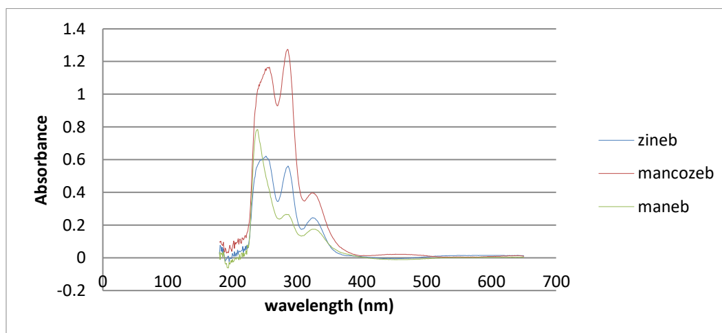
Figure 2. UV-visible spectrum for Zineb, Maneb and Mancozeb.
