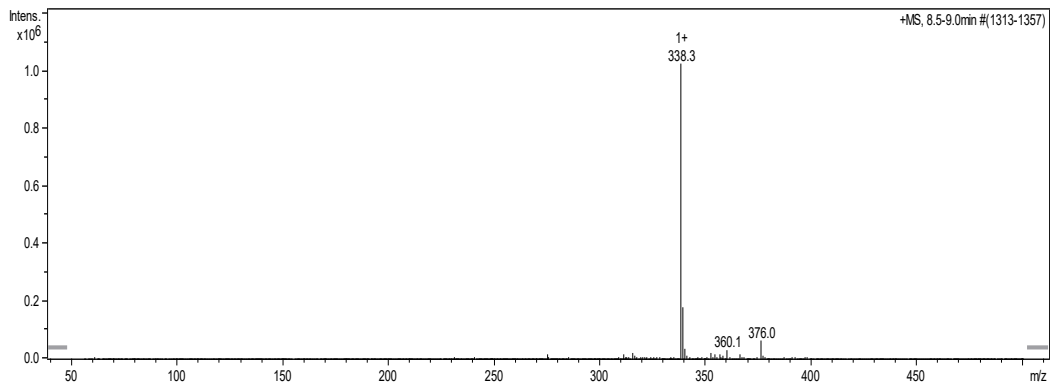
Fig. A2. Mass spectra of Trifluralin.
