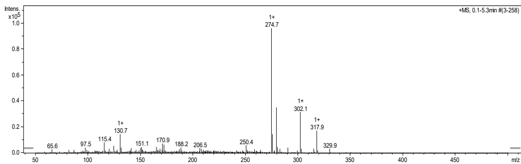
Fig. 4. Mass spectra for the positive peak of orange eluted with 60/40 of methanol/water.
