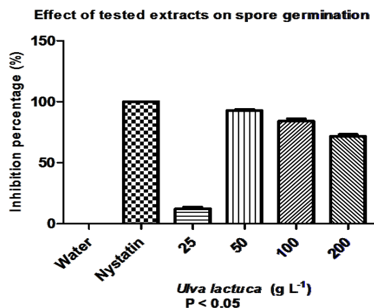
Figure 3: Inhibition percentage of the germination of P. digitatum incubated for 20 h at 22 °C in PDB containing Ulva lactuca extracts at different concentrations, water as negative control and Nystatine as positive control.
