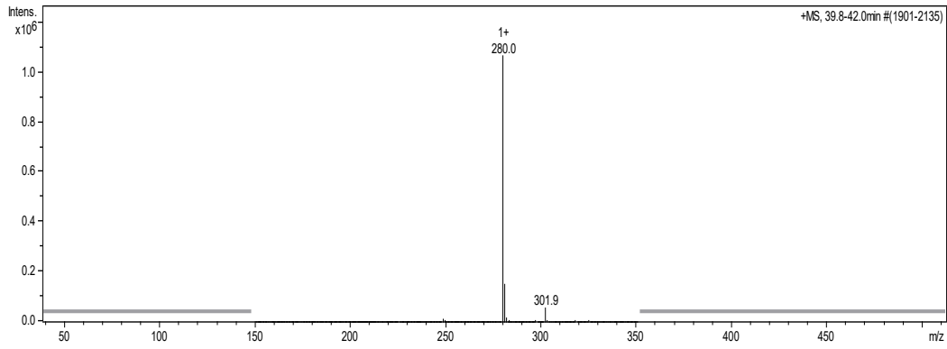
Fig. A1. Mass spectra of Metalaxyl
