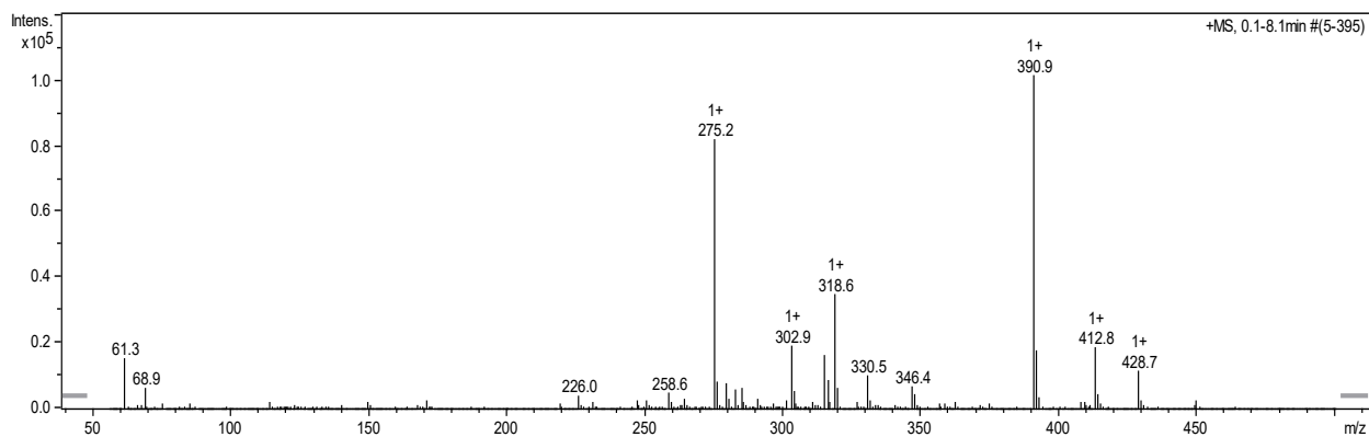
Fig. 3. Mass spectra for the positive peak of tomato eluted with 75/25 of PB/ACN.
