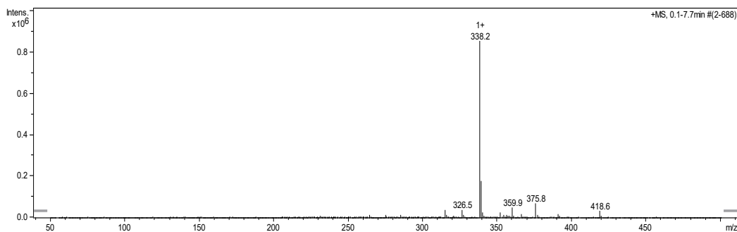
Fig. 8. Mass spectra for the positive peak of strawberries.
