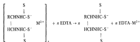
Figure 3. Complexation reaction of DTCs.
