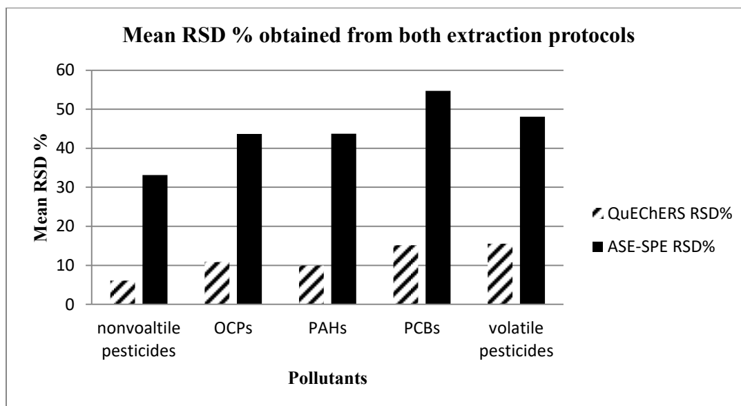
Figure 2: Mean RSD % of each pollutant type obtained with the two extraction methods
