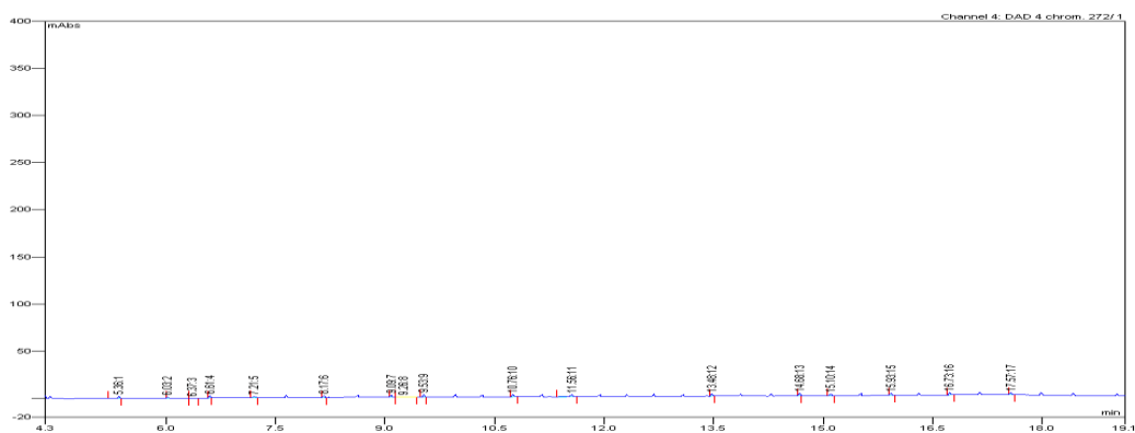
Figure 2s: Chromatogram of not spiked leeks
