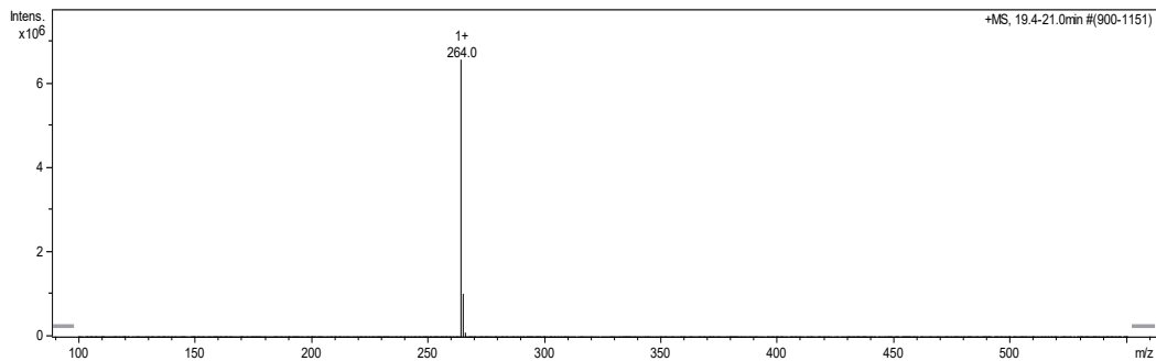
Fig. 7. Mass spectra for the positive peak of peach.
