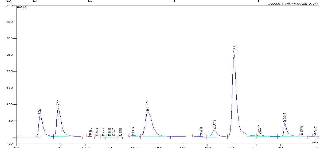
Figure 1. Chromatogram of DTCs mixture (1-Dazomet (T.R:6.26), 2-Metam-Na (T.R:7.77), 3-DMDTCs (T.R:15.11), 4-EBDTCs (T.R:22.19), 5-Propineb (T.R:26.35))
