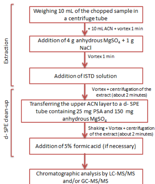
Figure 2: The main steps of the original QuEChERS extraction procedure
