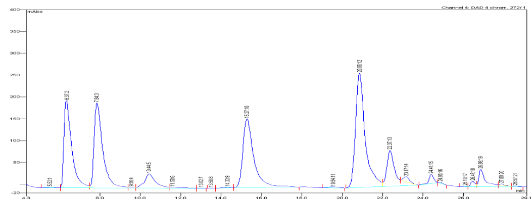
Figure 3s: Chromatogram of spiked leeks
