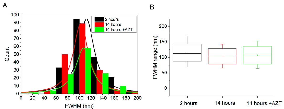
Figure 3.2.16. Histogram and box chart of the size distribution of NCp7-TC containing viral particles in the cytoplasm. Mean value is 115 +/- 30 nm at 2 h p.i. and 105 +/- 25 nm at 14 h p. i. and 110 +/- 30 nm 14 h p.i. in the presence of AZT. Comparison of the size distribution at 2 h and 14 h by chi square test: p=0,0023 . Difference of size populations for 2 h and 14 h in the presence of AZT is not significant.
