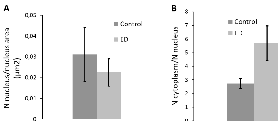
Figure 3.3.11. Quantification of labeled NC complexes inside the nuclear compartment. (A) Number of detected viral complexes per nucleus area ( p -value = 0.0559) and (B) ratio between the numbers of complexes found in cytoplasm vs nucleus.
