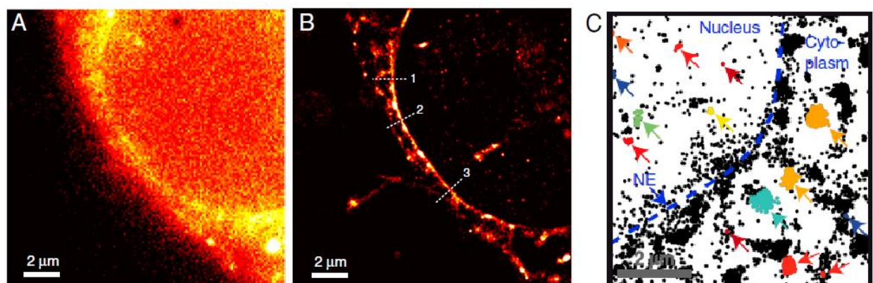
Figure 1.7.34. FIAsh-PALM imaging and analysis of HIV-1 particles labeled on IN-TC. (A) Widefield image and (B) SR reconstruction of 20,000 frames of the same region of HeLa cell infected for 2h. (C) All detected positions of FIAsh-IN clusters (multicolor arrows) (Adapted from (Lelek, Di Nunzio et al. 2012)).
