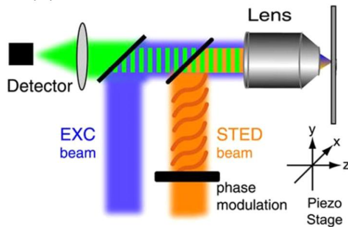
Figure 1.7.19. Basic setup of STED microscopy. It is composed of two laser beams, phase modulator, piezo stage, lenses and detector (Adapted from (Farahani, Schibler et al. 2010)).
