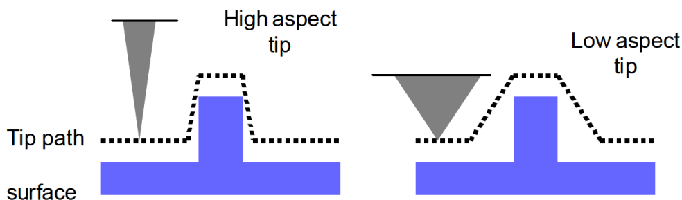
Figure 1.7.4. Influence of tip sharpness on surface sensing. The image of an object is spread by the tip profile and this process is both tip and sample dependent. As well, smaller objects will be in the shadow of tall ones and not recognized.
