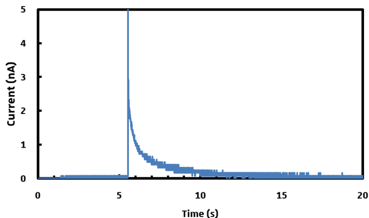
Figure 66: OASLM with a P3HT:PCBM (1:1) photosensitive layer current behaviour before and after the laser light is switched on.
