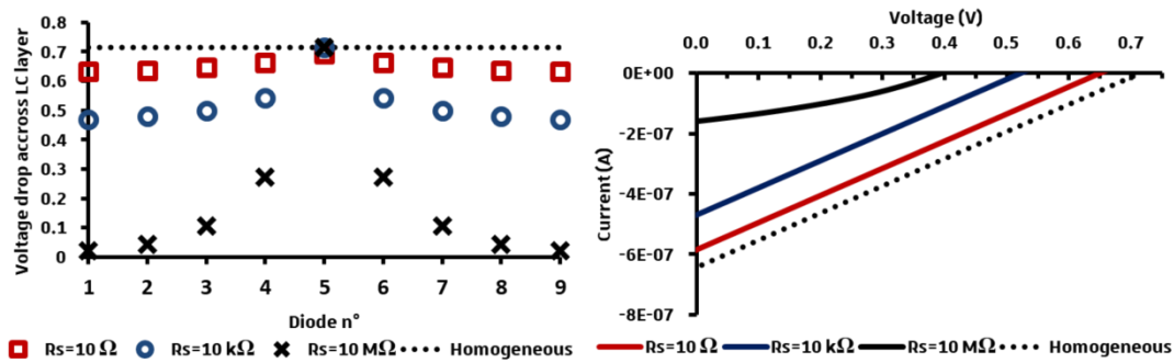
Figure 92: (a) Voltage drop across each layer as a function of diode location and sheet resistance value as specified on the graph. (b) Respective current vs voltage curve of the whole structure as a function of sheet resistance value as specified on the graph. Case of idealized silicon diodes
