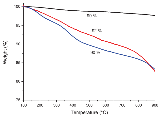
Figure 3.3 TG curves of pMWCNTs (black), oxMWCNTs 1 (red) and MWCNTs 3 (blue).
