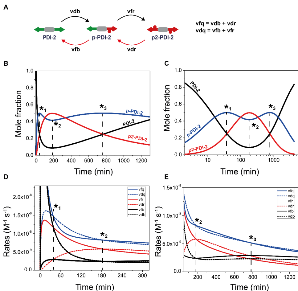
Figure 4.23. Reaction rates. (A) Rates of formation and disappearance of PDI-2 , p-PDI-2 , and p2-PDI-2 , due to their interconversion. (B) Simulation of the transient assembly reported in Figure 4.10A of the main text, with PDI-2 = 100 \mu\text{M} , ATP = 1 mM, PKA = 0.13 \mu\text{M} , and \lambda\text{PP} = 0.3 \mu\text{M} , as initial concentrations and using the optimized kinetic constants reported in Supplementary Table 4.4. (C) The same plot as panel (B) reported in semilog scale to better appreciate the maxima. (D) Change with time of the rates defined in panel (A) during the transient assembly reported in panel (B): zoom at shorter times; (E) Same data as (D) but zoomed at longer times. Reproduced from ref. *** (see page 79) with permission from Nature Research.
