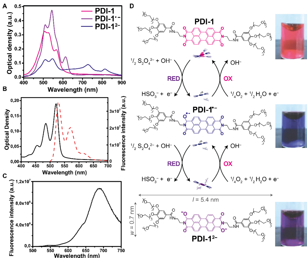
Figure 2.2. Model system PDI-1. (A) UV-Vis spectroscopy of 100 \mu\text{M} PDI-1 (pink line), PDI-1 •- (blue line) and PDI-1 2- (violet line) solutions in 50 mM borate buffer pH 8 (optical path 2 mm). (B) UV-Vis (black line) and fluorescence (red dashed line) spectra of 5 mM PDI-1 in acetonitrile (optical path 1 cm) show the characteristic vibronic progression of the PDI scaffold and the mirror image emission. (C) Fluorescence emission spectra of freshly prepared PDI-1 in 50 mM borate buffer pH 8 shows the absence of monomeric PDI-1 . (D) Redox cycle of PDI-1 . The neutral PDI-1 is reduced to PDI-1 •- upon addition of 1 eq. of \text{Na}_2\text{S}_2\text{O}_4 , further addition of \text{Na}_2\text{S}_2\text{O}_4 yields PDI-1 2- , which can be oxidized back by \text{O}_2 , via radical anion. Reproduced from ref. ** (see page 29) with permission from the Royal Society of Chemistry.
