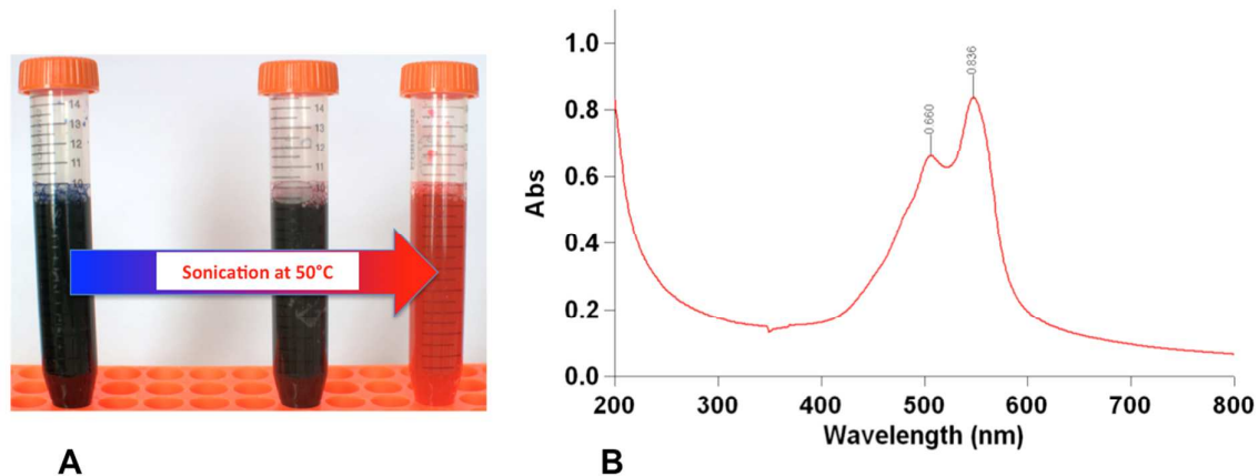
Figure S5: (A) Formation of the fluorescent crimson-red Nanofibers PDA-Nfs out of the initially blue solution, (B) UV-Vis absorption spectrum of the diluted PDA-Nfs solution (30 µg/mL).
