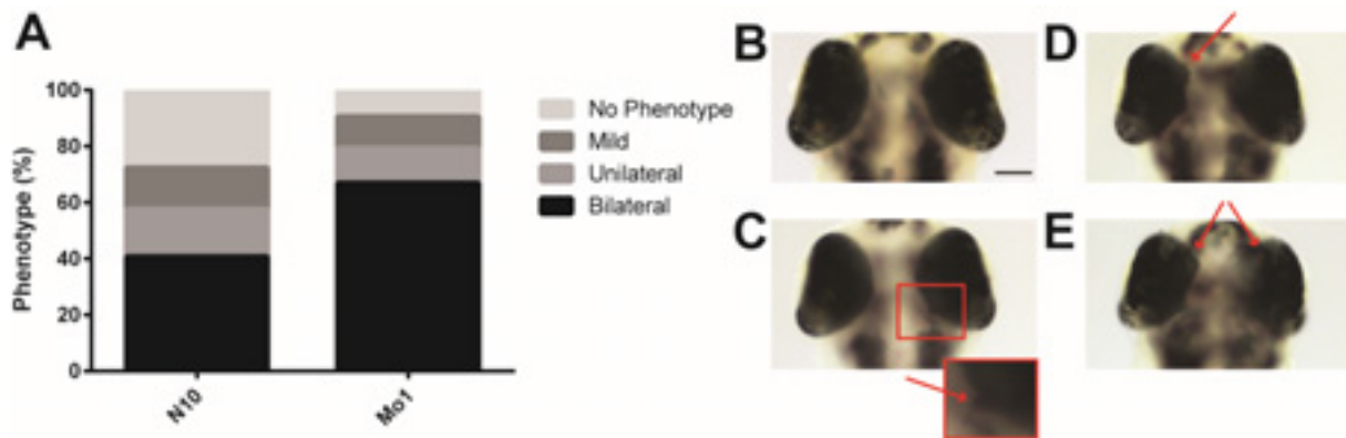
Figure 3 Human ATXN7 can partially compensate the loss of zebrafish atxn7 .
