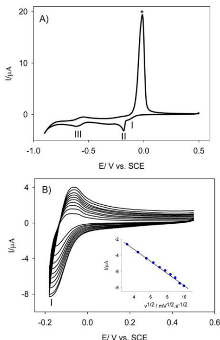
Figure 5. (A) CV of 0.1 mM P_2W_{15}CuAle in a pH 5 buffer solution (1 M CH_3COOLi + CH_3COOH ). v = 2 \text{ mV}\cdot\text{s}^{-1} . (B) Variation of scan rates (from inner to outer curve): 10, 20, 30, 40, 50, 60, 70, 80, 90, and 100 \text{ mV}\cdot\text{s}^{-1} . The potential reversal is fixed after the Cu^{II} to Cu^I redox process. (inset) Variation of the cathodic peak current intensity as a function of the square root of the scan rate. The working electrode was glassy carbon, and the reference electrode was the SCE. *Reoxidation peak of the deposited Cu^0 on electrode surface.
