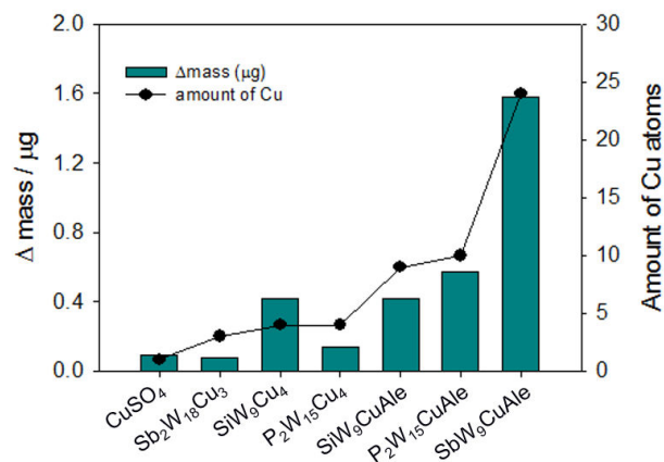
Figure III.7: Comparison of mass change in the presence of 0.1 \text{ mmol}\cdot\text{L}^{-1} sample in pH 5 1 \text{ mol}\cdot\text{L}^{-1} \text{CH}_3\text{COOLi} + \text{CH}_3\text{COOH} solution. v = 2 \text{ mV}\cdot\text{s}^{-1} (the deposition time is ca. 550 seconds) during EQCM measurement on a carbon deposited resonator ( A = 0.2 \text{ cm}^2 ) and the number of Cu atoms in structure.
