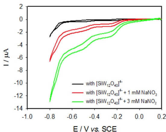
Figure II.6: Electrochemical reduction of \text{HNO}_2 in the presence of 0.1 \text{ mmol}\cdot\text{L}^{-1} [\text{SiW}_{12}\text{O}_{40}]^{4-} on GC electrode in \text{pH } 1 0.5 \text{ mol}\cdot\text{L}^{-1} \text{Na}_2\text{SO}_4 + \text{H}_2\text{SO}_4 , v = 2 \text{ mV}\cdot\text{s}^{-1} .
