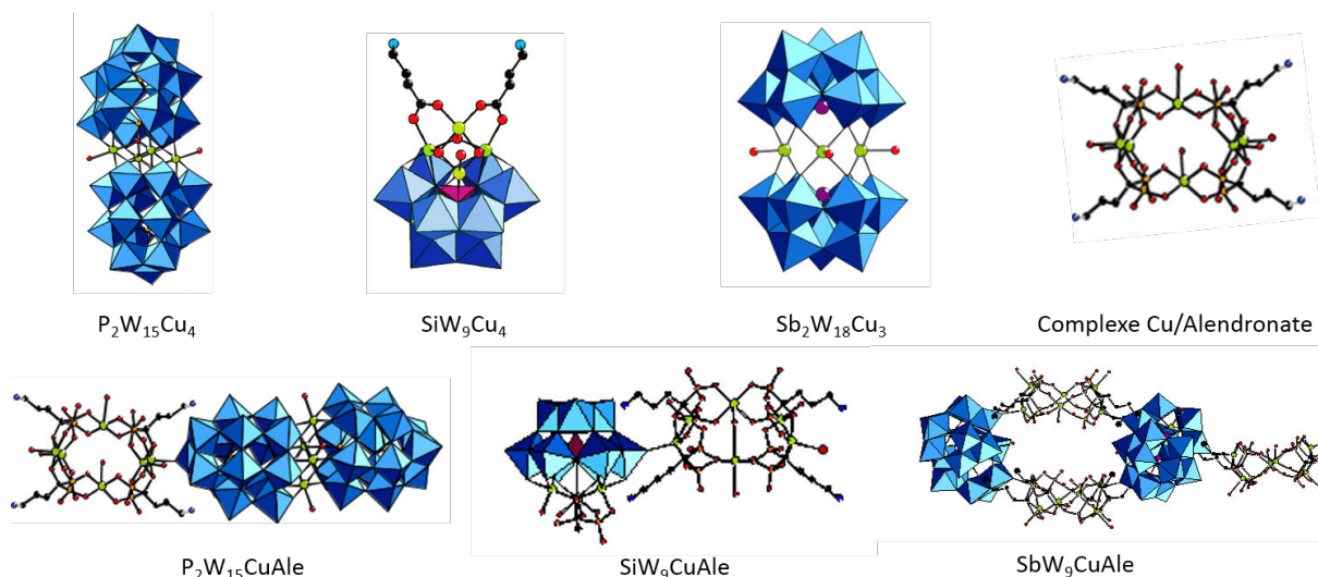
Figure III.1: Representation of various structures of Cu-substituted polyoxometalates and Cu complex synthesized from the Cu ions and Alendronate ligand (Ale) (Reproduced from reference 8. Copyright (2017) American Chemical Society).
