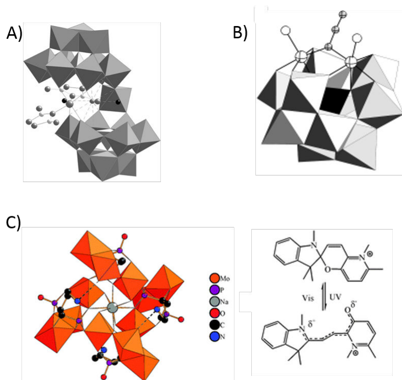
Figure I.5: Structures of A) Na_4K_9[(PW_9O_{34})_2(cis-WO_2)(cis-RuL^{Me})_2] \cdot 23H_2O reprinted from reference 51, Copyright (2017) American Chemical Society. B) [((Ni^{II}(H_2O))_2(\mu_{1,1}-N_3)(A-\alpha-PW_{10}O_{37}))^{6-}] reprinted from reference 52 with the permission from John Wiley and Sons. C) Structure of [(Mo_3O_8)_4(O_3PC(C_3H_6NH_3)(O)PO_3)_4]^{8-} unit and the representation of the closed and open forms of the spiropyran counteranion SP^+ . These representations are reprinted from reference 53 with the permission from Royal Society of Chemistry.
