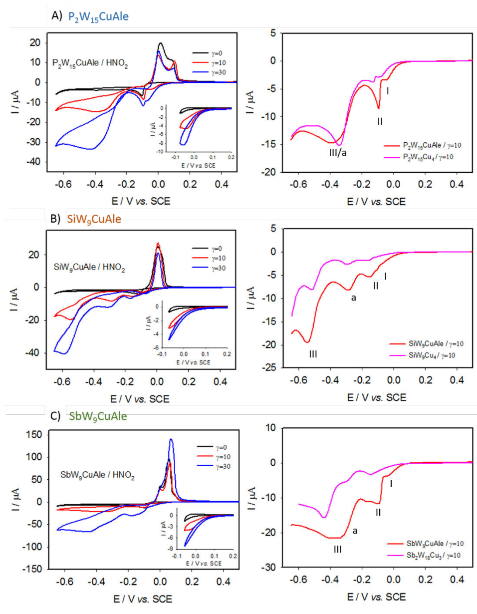
Figure III.17: (Left) Reduction of HNO_2 in the presence of 0.1 \text{ mmol}\cdot\text{L}^{-1} (A) P_2W_{15}CuAle , (B) SiW_9CuAle or (C) SbW_9CuAle . (Right) Reduction scans obtained for CuPOM/Ale (red curve) and the corresponding CuPOM (pink curve) after adding of 1 \text{ mmol}\cdot\text{L}^{-1} NaNO_2 ( \gamma = 10 ). Buffer solution: pH 1 0.5 \text{ mol}\cdot\text{L}^{-1} Na_2SO_4 + H_2SO_4 , v = 2 \text{ mV}\cdot\text{s}^{-1} .
