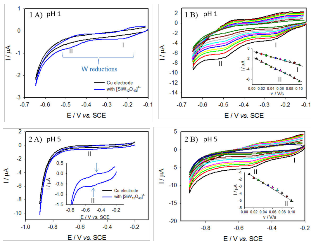
Figure II.2: Top: 1A) CV of 0.1 mmol·L -1 [SiW 12 O 40 ] 4- in pH 1 0.5 mol·L -1 Na 2 SO 4 + H 2 SO 4 solution on Cu electrode, \nu = 2 \text{ mV}\cdot\text{s}^{-1} . 1B) Variation of scan rates from inner to outer curve: 10, 20, 30, 40, 50, 60, 70, 80, 90 and 100 mV·s -1 . (Inset) variation of cathodic peak current intensity as a function of the scan rate. Bottom: 2A) CV of 0.1 mmol·L -1 [SiW 12 O 40 ] 4- in pH 5 1 mol·L -1 CH 3 COOLi + CH 3 COOH solution on Cu electrode, \nu = 2 \text{ mV}\cdot\text{s}^{-1} . 2B) Variation of scan rates from inner to outer curve: 10, 20, 30, 40, 50, 60, 70, 80, 90 and 100 mV·s -1 . (Inset) variation of cathodic peak current intensity as a function of the scan rate.
