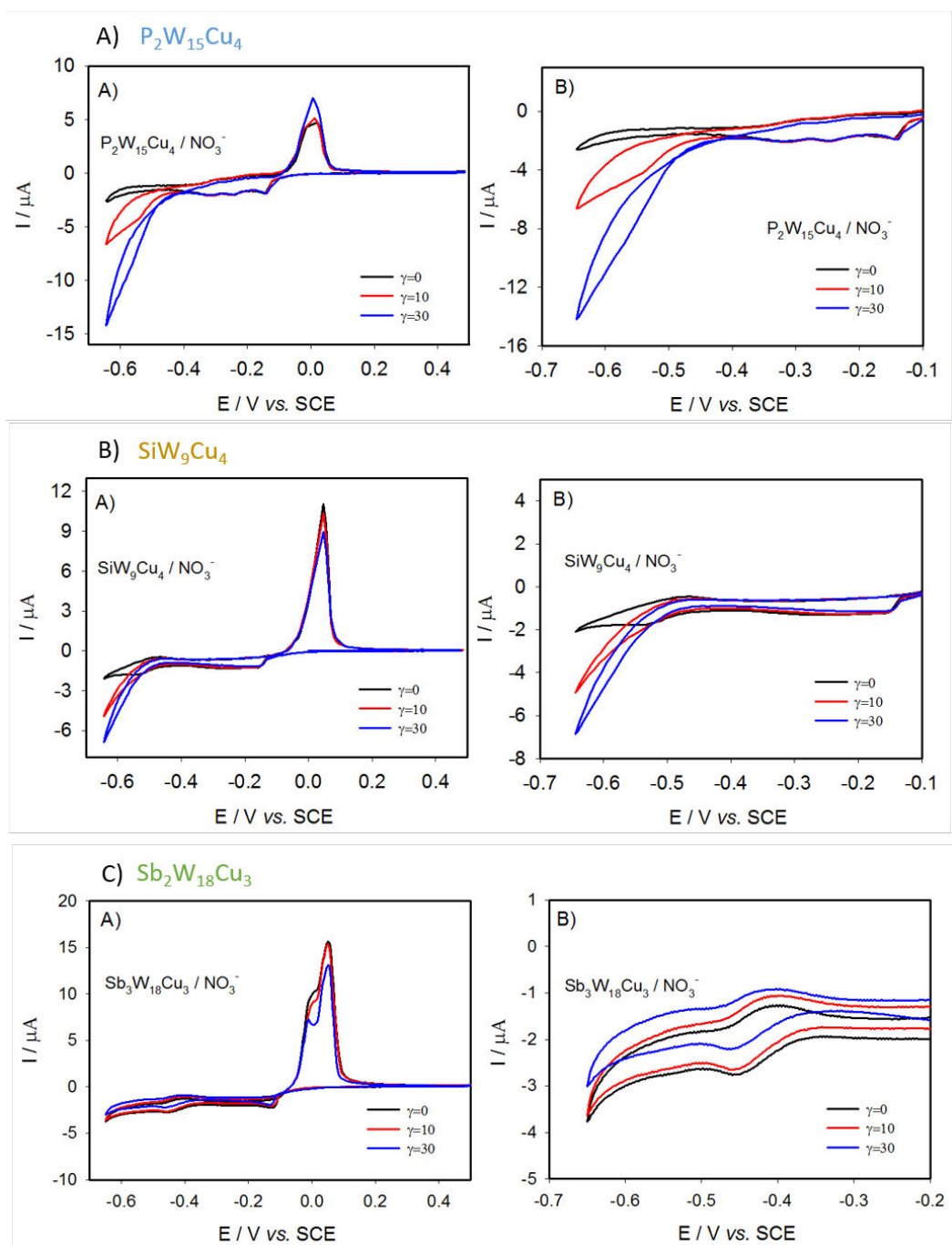
Figure III.13: (Left) Reduction of \text{NO}_3^- in presence of 0.1 \text{ mmol}\cdot\text{L}^{-1} (A) \text{P}_2\text{W}_{15}\text{Cu}_4 , (B) \text{SiW}_9\text{Cu}_4 or (C) \text{Sb}_2\text{W}_{18}\text{Cu}_3 (Right) Magnification of nitrate reduction at the potential of reduced POM. Buffer solution: \text{pH } 1 0.5 \text{ mol}\cdot\text{L}^{-1} \text{Na}_2\text{SO}_4 + \text{H}_2\text{SO}_4 , v = 2 \text{ mV}\cdot\text{s}^{-1} .
