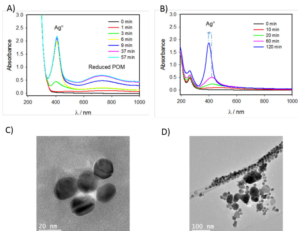
Figure IV.2: UV-visible absorption spectra and TEM micrographics of: synthesis a) a deaerated solution of [\text{SiW}_{12}\text{O}_{40}]^{4-} ( 3.5 \times 10^{-4} \text{ mol}\cdot\text{L}^{-1} ), \text{Ag}_2\text{SO}_4 ( 1 \times 10^{-4} \text{ mol}\cdot\text{L}^{-1} ) and propan-2-ol ( 0.5 \text{ mol}\cdot\text{L}^{-1} ) under illumination (A and C); synthesis b) a deaerated solution of [\text{SiW}_{12}\text{O}_{40}]^{4-} ( 8.4 \times 10^{-6} \text{ mol}\cdot\text{L}^{-1} ), \text{Ag}_2\text{SO}_4 ( 1 \times 10^{-4} \text{ mol}\cdot\text{L}^{-1} ) and propan-2-ol ( 0.5 \text{ mol}\cdot\text{L}^{-1} ) (B and D).
