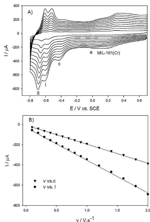
Figure 3. Top: cyclic voltammograms of Fe 6 W 18 @MIL-101(Cr) immobilized at a PG electrode in a 0.5 M pH 2.5 H 2 SO 4 -Na 2 SO 4 buffer solution at 2.0, 1.8, 1.2, 1.0, 0.8, 0.6, 0.4, 0.2 and 0 V s -1 (from top to bottom). Bottom: plots of i_{pc} vs. \nu for peak c (third Fe III/II redox couple) and peak I (first W VI/V redox couple).
