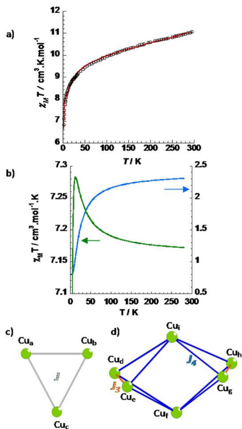
Figure 3. (a) Thermal behavior of \chi_M T for \text{SbW}_9\text{CuAle} at 1000 Oe in the 2–300 K range. The solid red line above the experimental data is the theoretical curve derived from the Hamiltonian 1 (see text); (b) deconvolution of the theoretical thermal behavior of \chi_M T for \text{SbW}_9\text{CuAle} highlighting the contributions of the POM (blue) and \{\text{Cu}_6\text{Ale}_4\} (green) fragments; (c) the coupling scheme used for modeling the magnetic behavior of the \{(\text{SbW}_9\text{O}_{33})_2\text{Cu}_3\} units in \text{SbW}_9\text{CuAle} ; (d) the coupling scheme used for modeling the magnetic behavior of the \{\text{Cu}_6(\text{Ale})_4(\text{H}_2\text{O})_4\} units in \text{SbW}_9\text{CuAle} and \text{SiW}_9\text{CuAle} .
