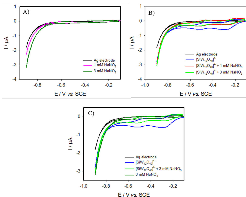
Figure II.20: A) Electrochemical reduction of NO 3 - on Ag electrode. B) Electrochemical reduction of NO 3 - in the presence of 0.1 mmol·L -1 [SiW 12 O 40 ] 4- on Ag electrode. C) Comparison of NO 3 - reduction with or without [SiW 12 O 40 ] 4- in solution. Buffer solution: pH 5 1 mol·L -1 CH 3 COOLi + CH 3 COOH, \nu = 2 \text{ mV}\cdot\text{s}^{-1} .
