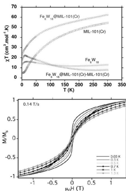
Figure 8. Top: temperature dependence of \chi_M T for MIL-101(Cr) (□), \text{Fe}_6\text{W}_{18}@\text{MIL}-101(\text{Cr}) (○), \text{Fe}_6\text{W}_{18} (◇), and [\chi_M T(\text{Fe}_6\text{W}_{18}@\text{MIL}-101(\text{Cr})) - \chi_M T(\text{MIL}-101(\text{Cr}))] (Δ). Bottom: magnetization vs. magnetic field hysteresis loops for \text{Fe}_6\text{W}_{18}@\text{MIL}-101(\text{Cr}) at the indicated temperatures and a sweep rate of 0.14 T/s. The contribution of the antiferromagnetic matrix was subtracted approximately. The magnetization is normalized to its saturation value M_s at 1.4 T.
