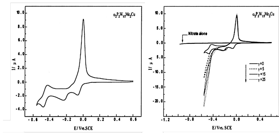
Figure I.15: Left) Cyclic voltammogram of the three first waves of 5 \times 10^{-4} \text{ mol} \cdot \text{L}^{-1} [\alpha_2\text{-P}_2\text{W}_{15}\text{Mo}_2\text{Cu}]^{8-} in 0.2 \text{ mol} \cdot \text{L}^{-1} \text{ Na}_2\text{SO}_4 + \text{H}_2\text{SO}_4 ( \text{pH} = 3 ), scan rate: 2 \text{ mV} \cdot \text{s}^{-1} . (Right) after adding of increasing amounts of nitrate with the excess parameter \gamma = C_{\text{NO}_3^-} / C_{\text{PO}_4^{3-}} . (Reprinted from reference 98 with the permission from Elsevier).
