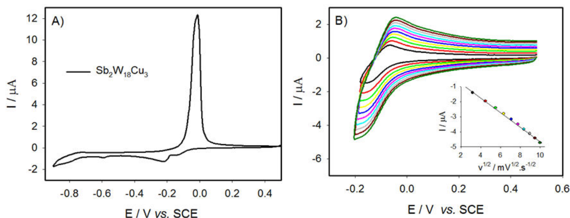
Figure S3: A) CV of 0.1 \text{ mmol}\cdot\text{L}^{-1} \text{Sb}_2\text{W}_{18}\text{Cu}_3 in \text{pH } 5 \text{ } 1 \text{ mol}\cdot\text{L}^{-1} \text{CH}_3\text{COOLi} + \text{CH}_3\text{COOH} solution, v = 2 \text{ mV}\cdot\text{s}^{-1} . B) Variation of scan rates of 0.1 \text{ mmol}\cdot\text{L}^{-1} \text{Sb}_2\text{W}_{18}\text{Cu}_3 in \text{pH } 5 \text{ } 1 \text{ mol}\cdot\text{L}^{-1} \text{CH}_3\text{COOLi} + \text{CH}_3\text{COOH} solution (from inner to outer curve: 10, 20, 30, 40, 50, 60, 70, 80, 90, and 100 \text{ mV}\cdot\text{s}^{-1} ). The potential reversal is fixed after \text{Cu}^{\text{II}} to \text{Cu}^{\text{I}} redox process. (Inset) Variation of the cathodic peak current intensity as a function of the square root of the scan rate.
