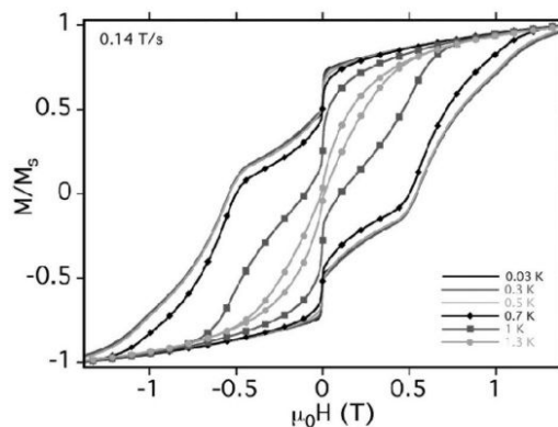
Figure 4. Magnetization vs. magnetic field hysteresis loops at the indicated temperatures and a sweep rate of 0.14 T/s for Fe 6 W 18 @Gel. The hysteresis loops are superimposed below 0.4 K establishing magnetization reversal through temperature-independent QTM. The magnetization is normalized to its saturation value M_s at 1.4 T.
