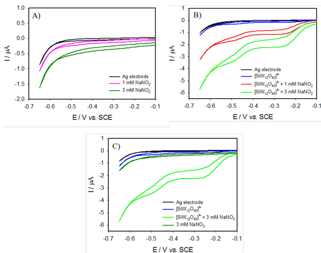
Figure II.8: A) Electrochemical reduction of HNO 2 on Ag electrode. B) Electrochemical reduction of HNO 2 in the presence of 1 mmol·L -1 [SiW 12 O 40 ] 4- on Ag electrode. C) Comparison of HNO 2 reduction with or without [SiW 12 O 40 ] 4- in solution. Buffer solution: pH 1 0.5 mol·L -1 Na 2 SO 4 + H 2 SO 4 , \nu = 2 \text{ mV}\cdot\text{s}^{-1} .
