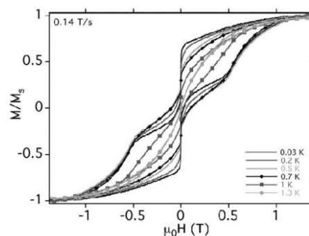
Figure 6. Magnetization vs. magnetic field hysteresis loops at the indicated temperatures and a sweep rate of 0.14 T/s for \text{Fe}_6\text{W}_{18}\text{@UiO-67} . The magnetization is normalized to its saturation value M_s at 1.4 T.
