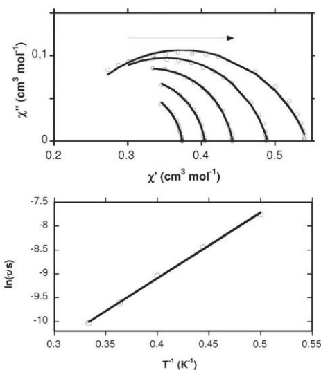
Figure 7. Top: Cole–Cole plots of \text{Fe}_6\text{W}_{18}\text{@UiO-67} constructed from the measurement of the frequency and temperature dependence of the in-phase \chi'_M and out-of-phase \chi''_M magnetic susceptibility under the zero applied dc field at (from left to right) 3, 2.75, 2.5, 2.25 and 2 K. The solid lines are fits of the experimental data using a generalized Debye model. Bottom: magnetization relaxation time plotted as \ln(\tau) vs. 1/T for \text{Fe}_6\text{W}_{18}\text{@UiO-67} . The solid line represents the fit to the Arrhenius law.
