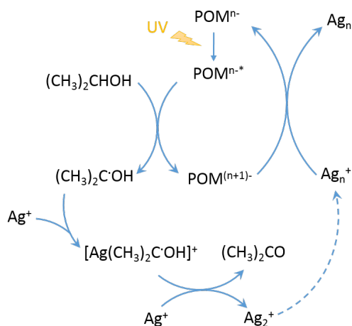
Figure I.11: Mechanism of the photoreduction of silver ions in the presence of POM.
