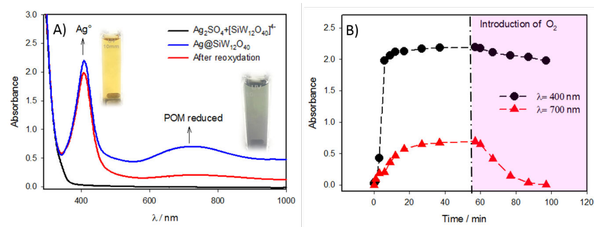
Figure IV.1: A) UV-visible absorption spectra of a solution containing [\text{SiW}_{12}\text{O}_{40}]^{4-} ( 3.5 \times 10^{-4} \text{ mol}\cdot\text{L}^{-1} ), \text{Ag}_2\text{SO}_4 ( 1 \times 10^{-4} \text{ mol}\cdot\text{L}^{-1} ) and propan-2-ol ( 0.5 \text{ mol}\cdot\text{L}^{-1} ) before (—), after (—) 50 minutes of illumination and after reoxydation in air (—). B) Measured absorbance bands at 400 nm and 700 nm as a function of illumination time.
