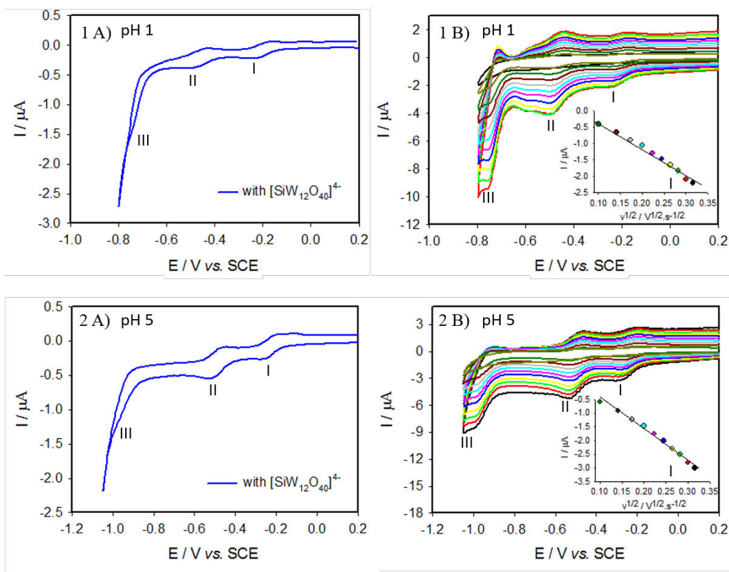
Figure II.1: Top: 1A) CV of 0.1 mmol·L -1 [SiW 12 O 40 ] 4- in pH 1 0.5 mol·L -1 Na 2 SO 4 + H 2 SO 4 solution on GC electrode, v = 2 mV·s -1 . 1B) Variation of scan rates from inner to outer curve: 10, 20, 30, 40, 50, 60, 70, 80, 90 and 100 mV s -1 . (Inset) variation of cathodic peak current intensity as a function of the scan rate. Bottom: 2A) CV of 0.1 mmol·L -1 [SiW 12 O 40 ] 4- in pH 5 1 mol·L -1 CH 3 COOLi + CH 3 COOH solution on GC electrode, v = 2 mV·s -1 . 2B) Variation of scan rates from inner to outer curve: 10, 20, 30, 40, 50, 60, 70, 80, 90 and 100 mV·s -1 . (Inset) variation of cathodic peak current intensity as a function of the scan rate.
