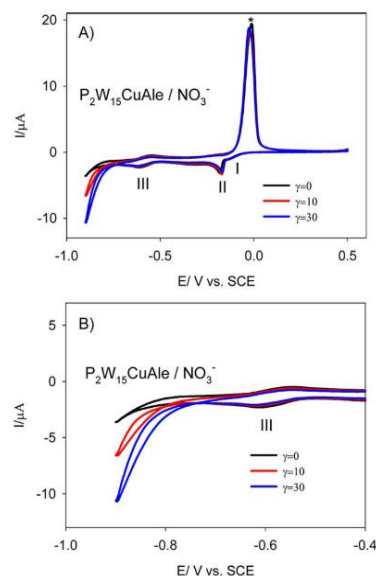
Figure 6. (A) Electrocatalysis of NO_3^- reduction in the presence of 0.1 mM P_2W_{15}CuAle in a pH 5 medium, v = 2 \text{ mV}\cdot\text{s}^{-1} . (B) Magnification of (A) to highlight the reduction of nitrate ions. *Reoxidation peak of the deposited Cu^0 on electrode surface.
