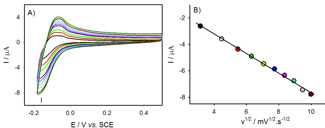
Figure III.3: A) Variation of scan rates of 0.1 \text{ mmol} \cdot L^{-1} P_2W_{15}CuAle in pH 5 1 \text{ mol} \cdot L^{-1} CH_3COOLi + CH_3COOH solution (from inner to outer curve: 10, 20, 30, 40, 50, 60, 70, 80, 90, and 100 \text{ mV} \cdot s^{-1} ). The potential reversal is fixed after Cu^{II} to Cu^I redox process. B) Variation of the cathodic peak current intensity as a function of the square root of the scan rate.
