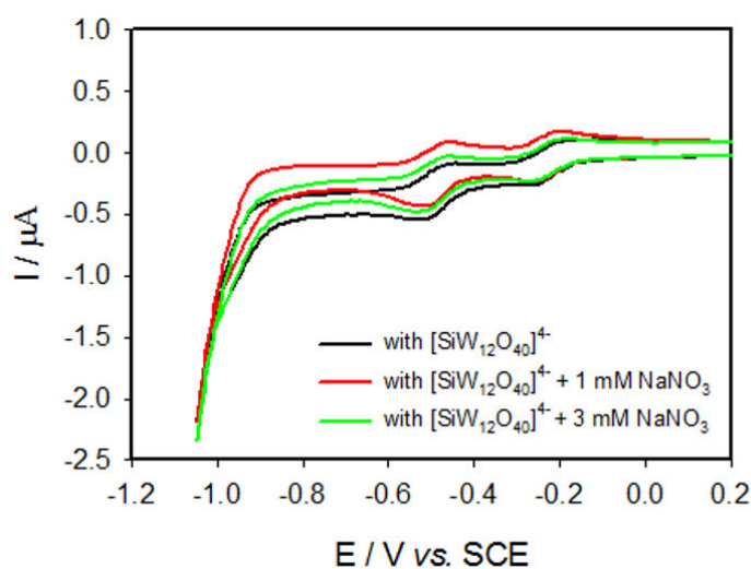
Figure II.18: Electrochemical reduction of NO 3 - in the presence of 0.1 \text{ mmol} \cdot \text{L}^{-1} [\text{SiW}_{12}\text{O}_{40}]^{4-} on GC electrode. Buffer solution: pH 5 1 \text{ mol} \cdot \text{L}^{-1} \text{CH}_3\text{COOLi} + \text{CH}_3\text{COOH} , v = 2 \text{ mV} \cdot \text{s}^{-1} .
