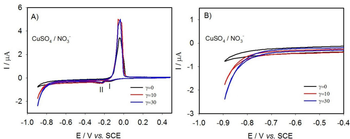
Figure III.14: A) Reduction of \text{NO}_3^- in the presence 0.1 \text{ mmol}\cdot\text{L}^{-1} \text{CuSO}_4 . B) Magnification of A) between -0.90 V to -0.40 V. Buffer solution: pH 5 1 \text{ mol}\cdot\text{L}^{-1} \text{CH}_3\text{COOLi} + \text{CH}_3\text{COOH} , \nu = 2 \text{ mV}\cdot\text{s}^{-1} .
