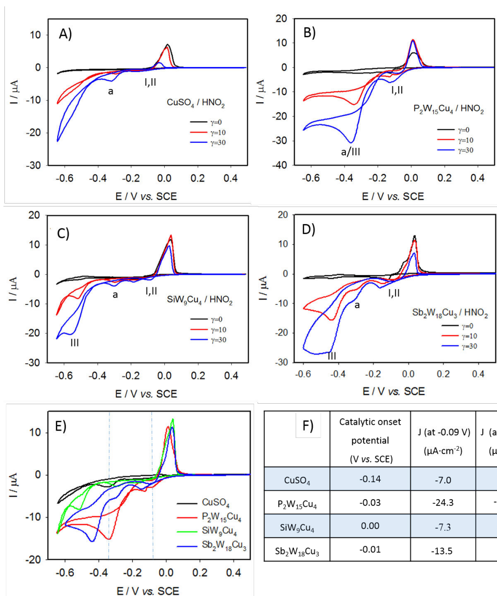
Figure III.8: Reduction of \text{HNO}_2 in the presence 0.1 \text{ mmol}\cdot\text{L}^{-1} (A) \text{CuSO}_4 , (B) \text{P}_2\text{W}_{15}\text{Cu}_4 , (C) \text{SiW}_9\text{Cu}_4 or (D) \text{Sb}_2\text{W}_{18}\text{Cu}_3 . E) Comparison of 1 \text{ mmol}\cdot\text{L}^{-1} \text{NaNO}_2 reduction (equivalent to \gamma = 10 ) by different samples ( 0.1 \text{ mmol}\cdot\text{L}^{-1} ). F) Catalytic onset potentials and kinetic current densities J_{\text{kinetic}}(\text{HNO}_2) in \mu\text{A}\cdot\text{cm}^{-2} calculated for 1 \text{ mmol}\cdot\text{L}^{-1} \text{NaNO}_2 (equivalent to \gamma = 10 ). Buffer solution pH 1 0.5 \text{ mol}\cdot\text{L}^{-1} \text{Na}_2\text{SO}_4 + \text{H}_2\text{SO}_4 , v = 2 \text{ mV}\cdot\text{s}^{-1} . For the discussion of waves I, a, and III, see text.
