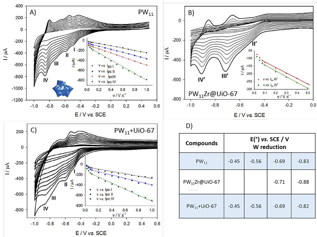
Figure V.4: Cyclic voltammograms of (A) PW_{11} , (B) PW_{11}Zr@UiO-67 and (C) PW_{11}+UiO-67 (mechanical mixing) immobilized on a PG electrode at different scan rate from 0.025 to 1.000 V \cdot s^{-1} . (Inset) plots of I_{pc} vs. v for reduction peaks. D) Reduction potentials of each composite immobilized on PG electrode. Buffer Solution: pH 2.5 0.5 mol·L -1 Na_2SO_4 + H_2SO_4 .
