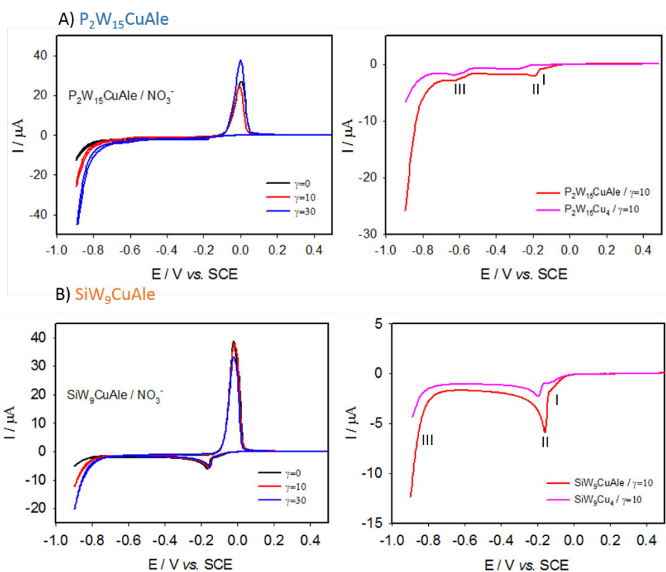
Figure III.22: (Left) Reduction of NO_3^- in the presence of 0.1 mmol·L -1 (A) P_2W_{15}CuAle or (B) SiW_9CuAle . (Right) Negative scans obtained for CuPOM/Ale (red curve) and the corresponding CuPOM (pink curve) after adding of 1 mmol·L -1 NO_3^- . Buffer solution: pH 5 1 mol·L -1 CH_3COOLi + CH_3COOH solution, v = 2 \text{ mV} \cdot \text{s}^{-1} .
