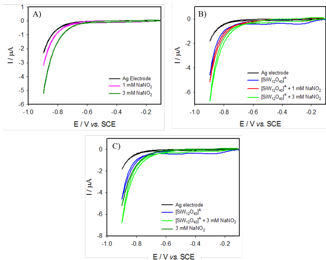
Figure II.12: A) Electrochemical reduction of NO 2 - on Ag electrode. B) Electrochemical reduction of NO 2 - in the presence of 0.1 mmol·L -1 [SiW 12 O 40 ] 4- on Ag electrode. C) Comparison of NO 2 - reduction with or without [SiW 12 O 40 ] 4- in solution. Buffer solution: pH 5 1 mol·L -1 CH 3 COOLi + CH 3 COOH, \nu = 2 \text{ mV}\cdot\text{s}^{-1} .
