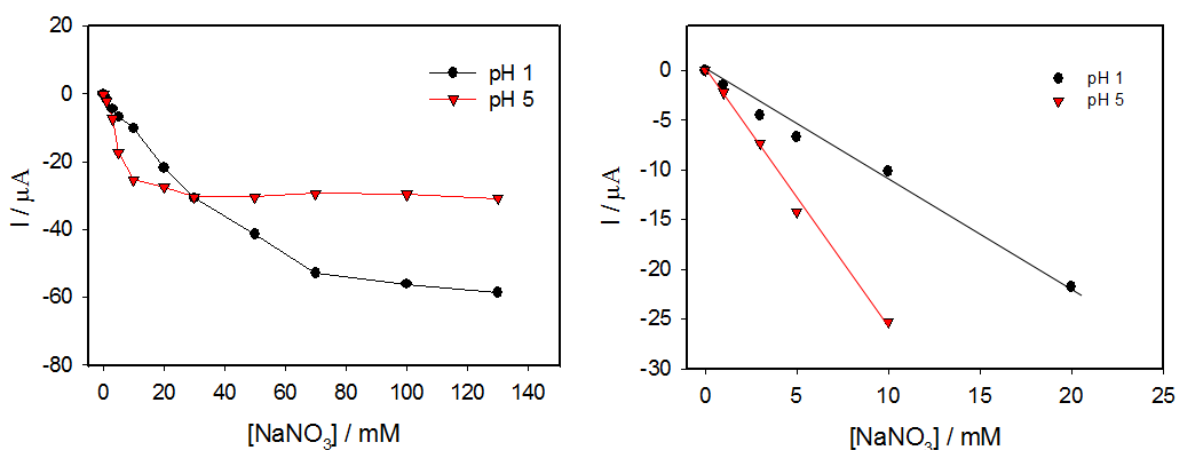
Figure III.24: Sensing properties of P_2W_{15}CuAle towards nitrate reduction in pH 1 0.5 mol·L -1 Na 2 SO 4 + H 2 SO 4 solution or in pH 5 1 mol·L -1 CH 3 COOLi + CH 3 COOH solution. The current is measured at -0.55 V at pH 1 and at -0.85 V at pH 5.
