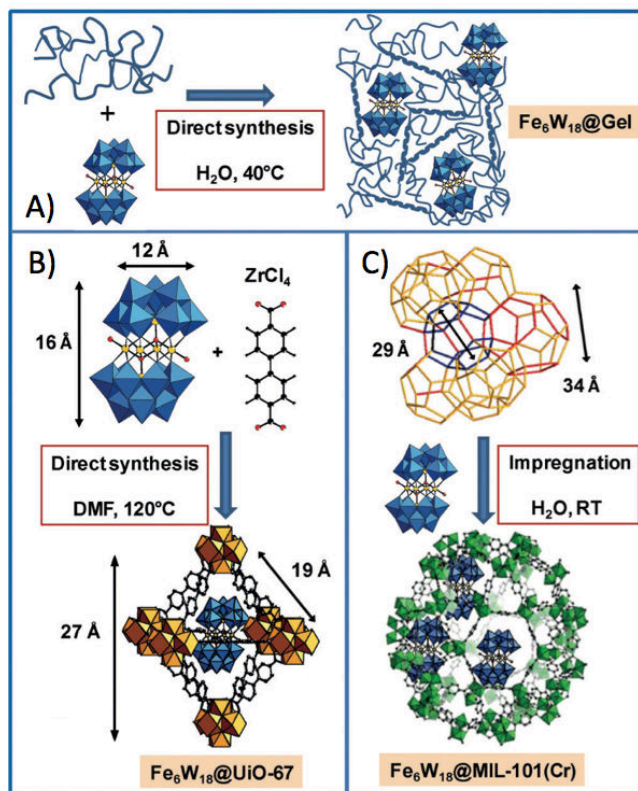
Figure V.5. Representations of POM [\text{Fe}_4(\text{FeW}_9\text{O}_{39})_2(\text{H}_2\text{O})_2]^{10-} ( \text{Fe}_6\text{W}_{18} ), UiO-67, MIL-101(Cr), gelatin and the synthetic routes to the three composite materials A) \text{Fe}_6\text{W}_{18}@\text{Gel} , (B) \text{Fe}_6\text{W}_{18}@\text{UiO-67} and C) \text{Fe}_6\text{W}_{18}@\text{MIL-101(Cr)} . (Reprinted from reference 15 with the permission from John Wiley and Sons).
