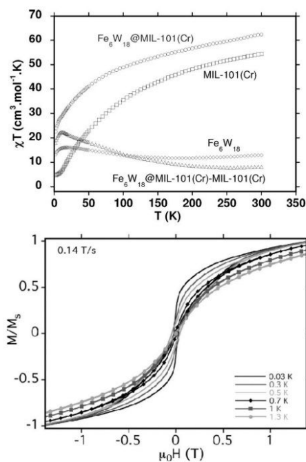
Figure 8. Top: temperature dependence of \chi_M T for MIL-101(Cr) (□), \text{Fe}_6\text{W}_{18} @MIL-101(Cr) (○), \text{Fe}_6\text{W}_{18} (◊), and [\chi_M T(\text{Fe}_6\text{W}_{18}@MIL-101(Cr)) - \chi_M T(\text{MIL-101(Cr)})] (Δ). Bottom: magnetization vs. magnetic field hysteresis loops for \text{Fe}_6\text{W}_{18} @MIL-101(Cr) at the indicated temperatures and a sweep rate of 0.14 T/s. The contribution of the antiferromagnetic matrix was subtracted approximately. The magnetization is normalized to its saturation value M_s at 1.4 T.
