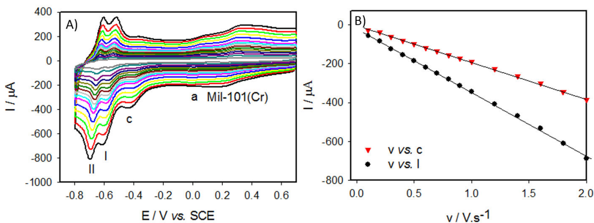
Figure V.8: Cyclic voltammograms of \text{Fe}_6\text{W}_{18}@MIL-101(\text{Cr}) immobilized on PG electrode in pH 2.5 0.5 \text{ mol}\cdot\text{L}^{-1} \text{Na}_2\text{SO}_4 + \text{H}_2\text{SO}_4 solution at different scan rates from 0.1 to 2.0 \text{ V}\cdot\text{s}^{-1} . (Inset): plots of I_{pc} vs. \nu for peak c ( \text{Fe}^{\text{III/II}} redox couple) and peak I ( \text{W}^{\text{VI/V}} redox couple).
