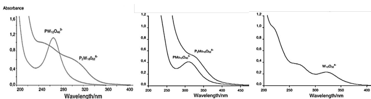
Figure I.6: Examples of UV-visible spectra of certain POMs. (Reprinted from reference 61 with permission from Royal Society of Chemistry).
