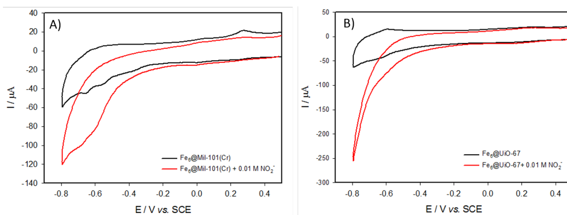
Figure V.9: reduction of 0.01\text{ mol}\cdot\text{L}^{-1}\text{ NaNO}_2 in the presence of (A) \text{Fe}_6\text{W}_{18}\text{@MIL-101}(\text{Cr}) or (B) \text{Fe}_6\text{W}_{18}\text{@UiO-67} immobilized on PG electrode. Buffer solution: \text{pH } 2.5\text{ } 0.5\text{ mol}\cdot\text{L}^{-1}\text{ Na}_2\text{SO}_4 + \text{H}_2\text{SO}_4 , scan rate: \nu = 10\text{ mV}\cdot\text{s}^{-1} .
