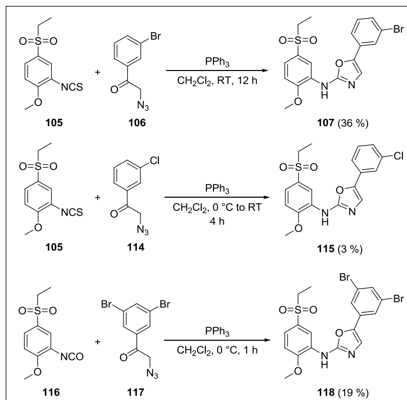
Scheme 6. Examples of the cyclization reactions leading to N ,5-diaryloxazol-2-amine derivatives 107 , 115 and 118 (reaction conditions: \text{PPh}_3 , \text{CH}_2\text{Cl}_2 , 0^\circ\text{C} or RT, 1 h to 12 h).
