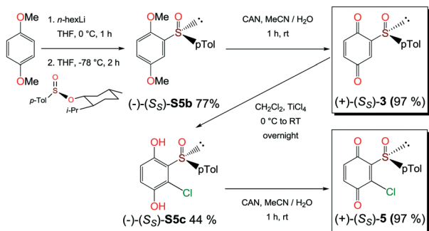
Scheme 2 Syntheses of quinones 3 and 5 from 1,4-dimethoxybenzene.
