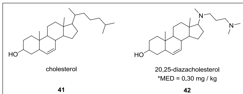
Figure 13. Cholesterol ( 41 ) and its bioisosteric analogue 20,25-diazacholesterol ( 42 ).
