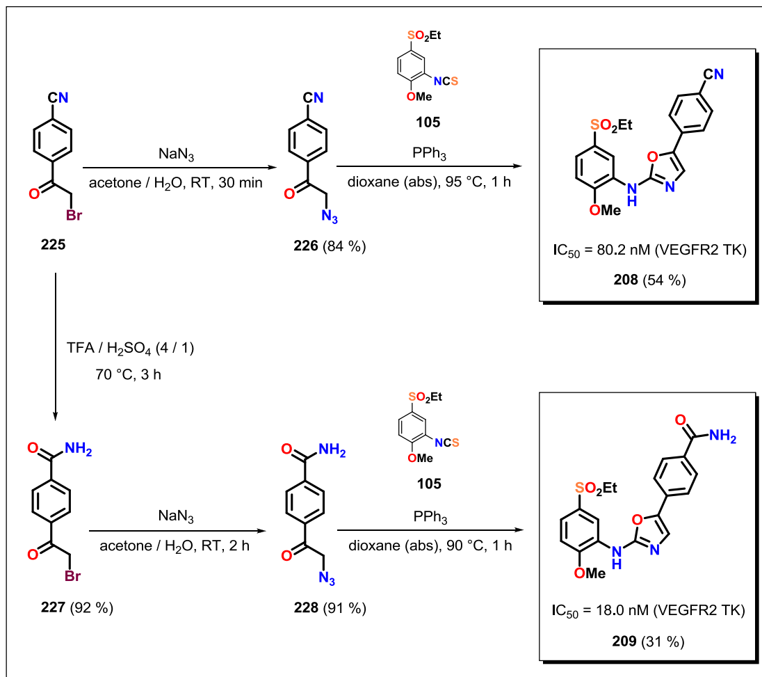
Scheme 30. Synthesis of p -substituted N ,5-diaryloxazol-2-amines 208 , 209 .
