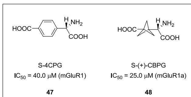
Figure 18. The example of unconventional phenyl / propellane bioisosteric replacement.
