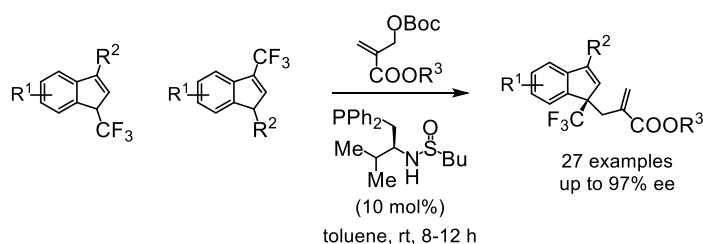
Scheme 3.5. Enantioselective allylic alkylation of mix -CF 3 indenenes (Zhang et al. 2017)
