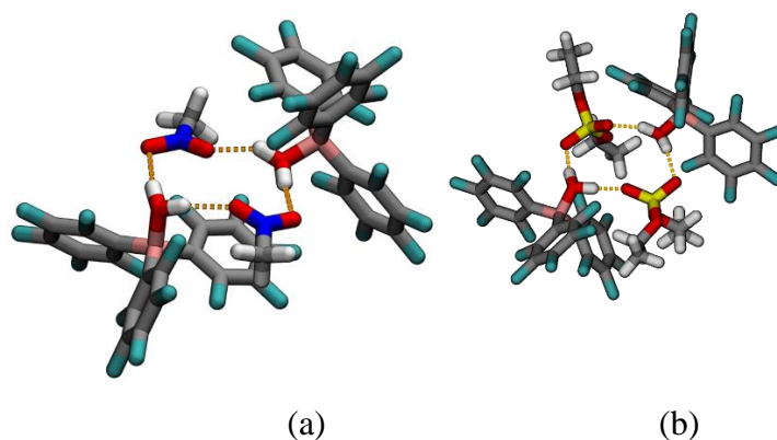
Figure 1.7. (a) Complex of B(C 6 F 5 ) 3 ·H 2 O and nitromethane. (b) Complex of B(C 6 F 5 ) 3 ·H 2 O and diethylsulfate.
