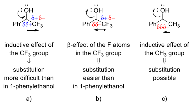
Figure 2.6. (a) Inductive effect of the CF_3 group on the alcohol reactivity. (b) \beta -effect of the CF_3 group on the alcohol reactivity. (c) Inductive effect of the methyl group on the alcohol reactivity.
