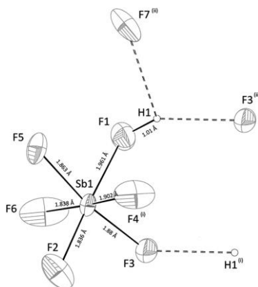
Figure 1.8. An \text{HSbF}_6 molecule with intermolecular hydrogen bonds in the crystal
