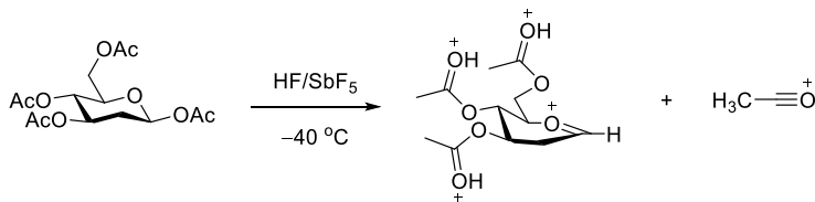
Scheme 1.9. The use of \text{HSbF}_6 for capture of the glucosyl cation
