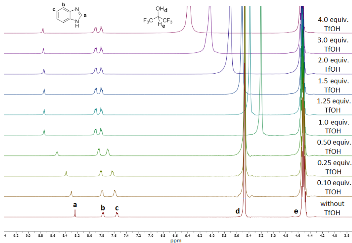
Figure 2.2. ^1\text{H-NMR} titration of benzimidazole in HFIP with TfOH
