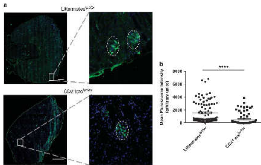
Figure 8 Invalidation of autophagy in B cells reduces IgG deposits in the kidney of lupus-prone mice. Mice bearing the \beta mutation on the C57BL/6 background were crossed with Atg5^{fl/fl} CD21 cre mice ( CD21 cre ^{Atg5^{fl/fl}} ) and their kidneys were collected at the age of 8 months. Atg5^{fl/fl} CD21 cre littermates or harbouring the \beta mutation were used for comparison (littermates ^{Atg5^{fl/fl}} ). Organ sections stained with anti-mouse IgG Abs before analysis on a spinning disk confocal microscope. (a) The total section was scanned and a representative image for each genotype is shown on the left. The white bars represent 500 \mu m. A magnification is indicated on the right to exemplify a glomerulus positive for IgG deposition, delimited by the dashed line. (b) The intensity of IgG staining was determined for each glomerulus as indicated in Materials and methods. Individual values of littermates ^{Atg5^{fl/fl}} ( n = 5 ) and CD21 cre ^{Atg5^{fl/fl}} ( n = 4 ) ( n = 20 glomeruli per animal) for each genotype were pooled and plotted on the graph. The bars represent the mean of glomerular IgG staining intensity for each genotype. ****P < 0.001 (Mann-Whitney U-test).
