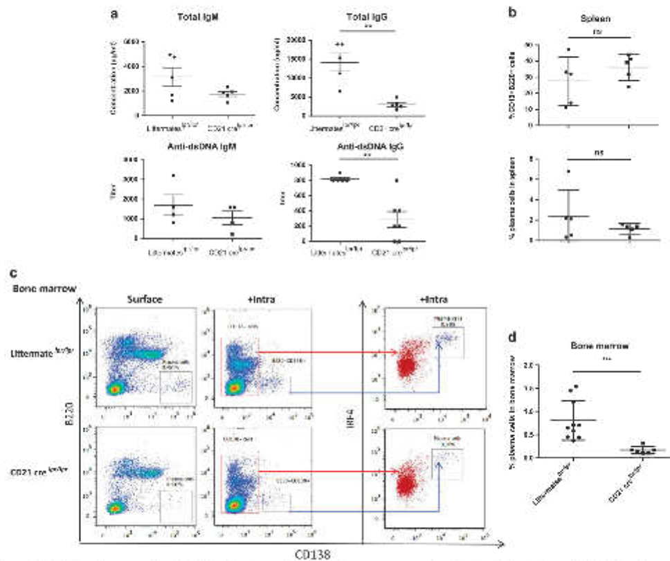
Figure 7 Autophagy is necessary for survival of long-lived plasma cells during subimmune responses. Mice harbouring the \beta mutation on the C57BL/6 background were crossed with \text{Atg5}^{\text{fl/fl}} CD21 ^{cre/+} mice (CD21 ^{cre/+} ). They were compared with littermate \text{Atg5}^{\text{fl/fl}} CD21 ^{cre/+} mice, also crossed with \beta mice (littermates ^{+/+} ), in the age of 9 months. (a) Individual values for each mouse assayed for absolute IgG and IgM concentrations in the serum, determined by ELISA and titres of anti-dsDNA IgM and IgG Abs. Means and SEM are represented (at least four mice in each group). (b) The spleens of the animals were collected, cells were stained by anti-CD138, anti-CD135, and anti-B220 Abs, and analysed by flow cytometry. Each point represents the value for an individual mouse. The central bar represents the means and the upper and lower bars symbolize the S.D. (c) Staining of bone marrow cells collected from one femur per mouse. Each dot plot stands for one representative case for each genotype. On the left, the gate delimiting B220 + CD138 + cells should indicate the percentages of plasma cells resident in the bone marrow (surface). In the middle, results obtained after an intracellular staining of IRF4 molecule performed after surface staining of the previous markers (intra). The red population corresponding to CD138 + cells is IRF4 hi or IRF4 lo . The CD138 + blue population corresponding to plasma cells is IRF4 hi . This latter staining was performed on four littermate ^{+/+} mice and one CD21 ^{cre/+} mouse. (d) Percentage of plasma cells among the bone marrow cells for individual mice analysed as in (c). n = 10 for littermate ^{+/+} and n = 6 for CD21 ^{cre/+} . Mean and S.D. are indicated. ** P < 0.01 , *** P < 0.001 (Mann-Whitney U-test).
