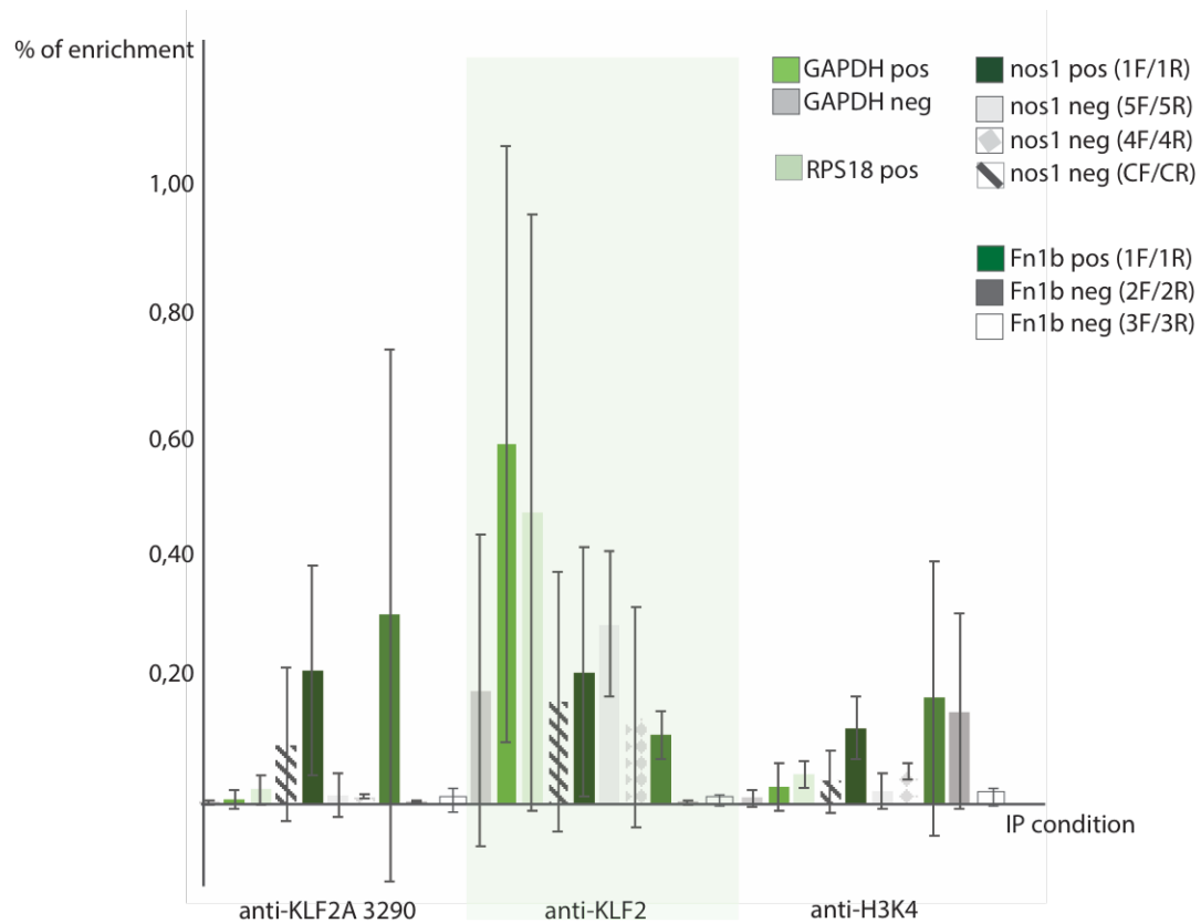
Figure 30: ChIP-qPCR
