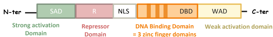
Figure 12: zebrafish Egr1 protein domains.
