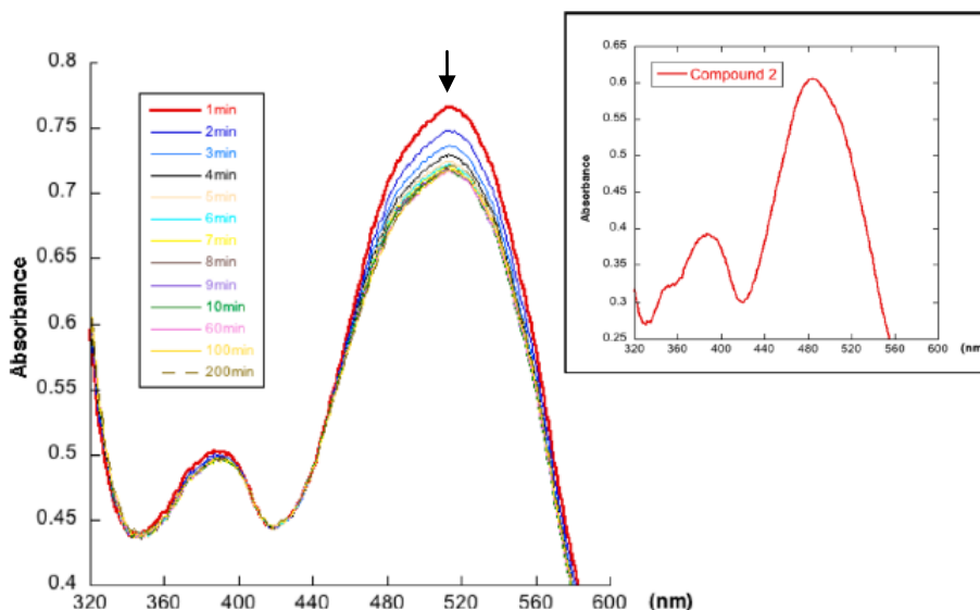
Figure 7. Behavior of 2 in a MeCN/ \text{CH}_2\text{Cl}_2 solution in the presence of 5 equiv of \text{Bu}_4\text{NCl} . Inset shows the spectrum of 2 in the same solvent mixture (no change with time)
