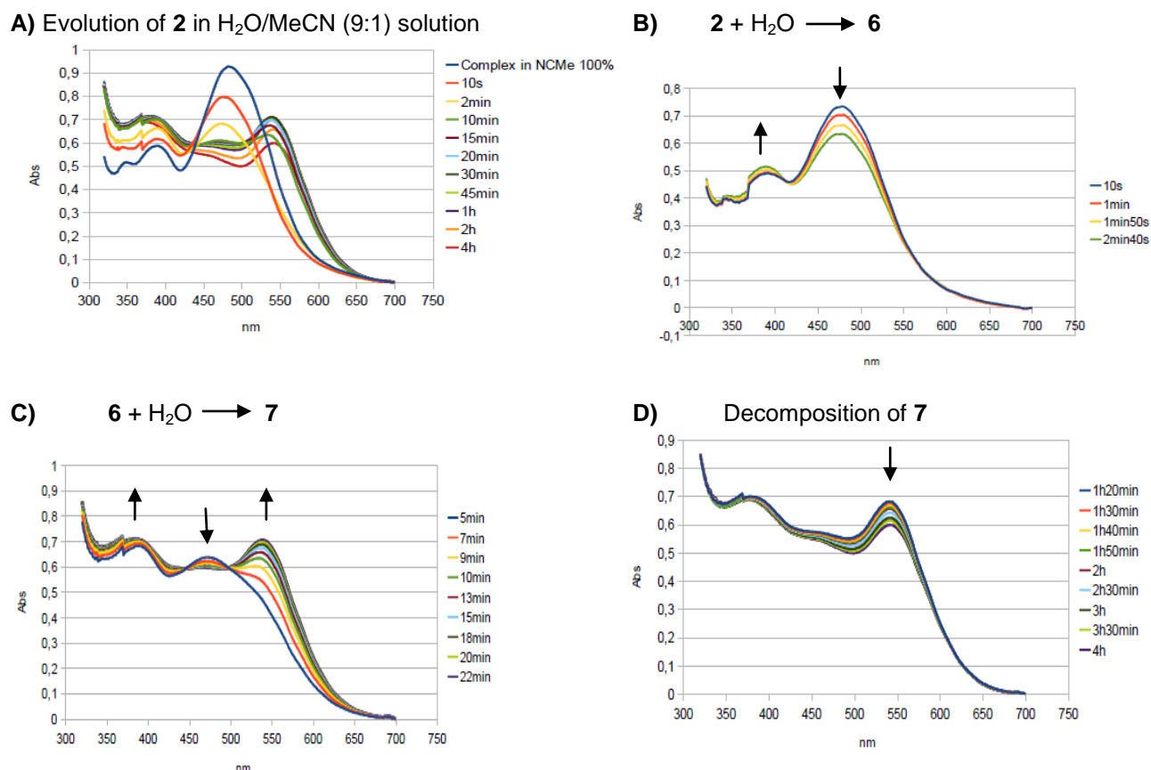
Figure 5. Electronic spectra of 2 in H 2 O/MeCN (9:1) solution (10 -4 M): (A) evolution from 10 s to 4 h, (B) evolution from 10 s to 160 s (isosbestic point at 412 nm), (C) evolution from 5 min to 22 min (isosbestic points: 455 and 498 nm), and (D) evolution after 80 min
