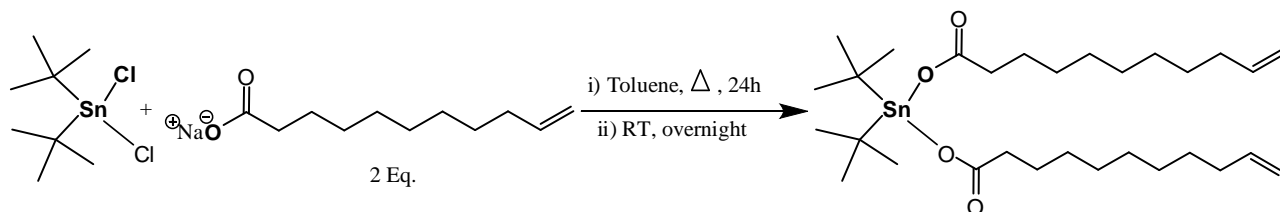
Figure 3. General reaction conditions employed for the synthesis of R_nSn(OOCR')_{4-n} ( n=1 to 3). Example: t\text{-Bu}_2SnUnd_2
