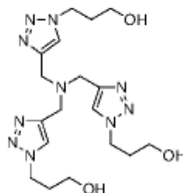
Figure 7. Chemical structure of the accelerating ligand THPTA
