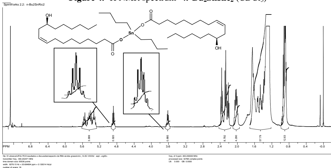
Figure 4. ^1H NMR spectrum - n\text{-Bu}_2SnRic_2 ( CDCl_3 )
