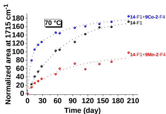
Figure IV-19: Normalized area at 1715 cm -1 describing the oxidation process of 14 alone, with 9Co-2-F4 and with 9Mn-2-F4 as a function of time at 70 °C.
