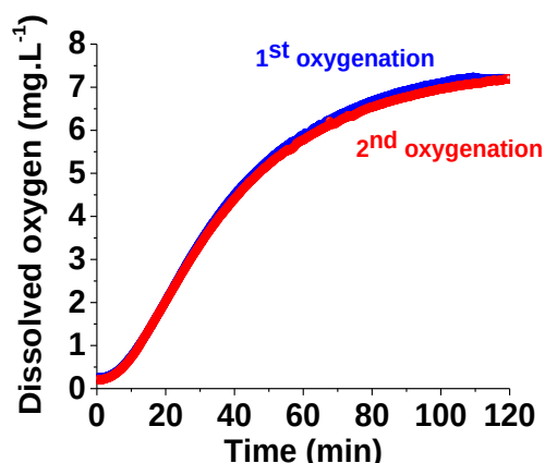
Figure II-43: Superimposition of the two oxygenation curves of 8Co ; [8Co] = 2 \times 10^{-4} M , solvent: dioxane:H 2 O (1:1 v/v).
