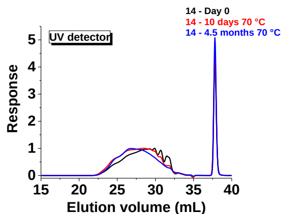
Figure IV-50: SEC measurements of non-oxidized 14 before (black) and after 10 days (red) and 4.5 months (blue) of oxidation at 70 °C - UV detector.
