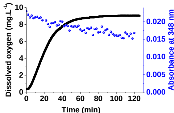
Figure II-45: Dioxygen concentration and absorbance variation at 348 nm as a function of time for the second oxygenation stage of 1Co ; [1Co] = 6 \times 10^{-4} M , solvent: dioxane:H 2 O (1:1 v/v), l = 1 cm.
