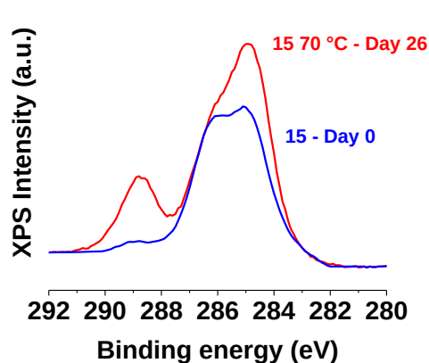
Figure IV-64: XPS C 1s scans of 15 .
