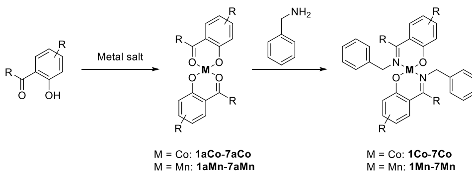
Scheme II-7: Second synthetic route for the preparation of the metal catalysts.
