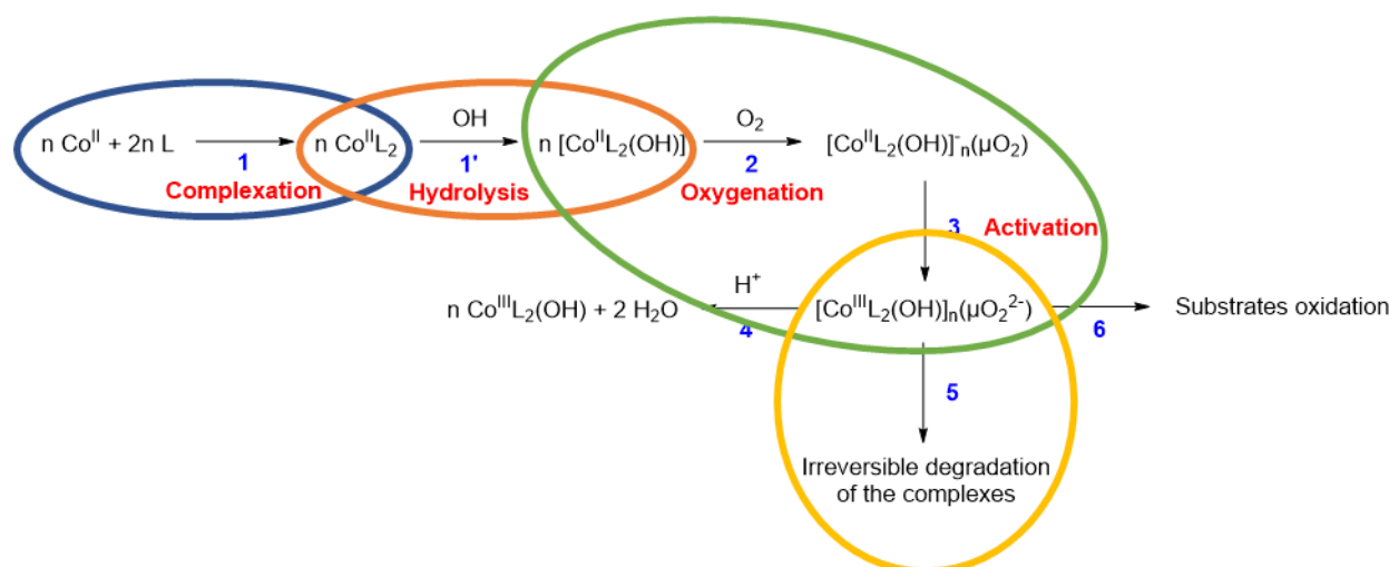
Figure II-77: Putative mechanism of complexation, oxygenation and activation of cobalt(II) complexes. Main steps are noted 1 to 6 . Adapted from Cabani.
