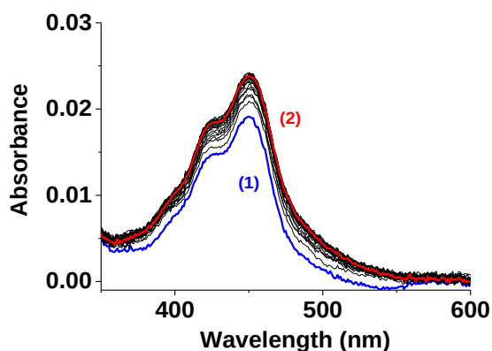
Figure III-11: UV-visible absorption spectrophotometric variations of 11 with m -CPBA (5 equiv.) as a function of time; (1) t = 0 , (2) t = 50 min, [11] = 7.71 \times 10^{-3} M , solvent: EtOH, l = 1 cm.
