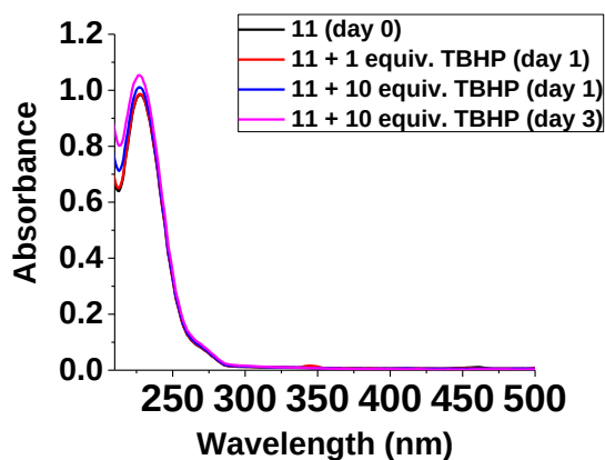
Figure III-2: Oxidation of 11 with TBHP (1 and 10 equiv.) monitored by UV-visible absorption spectrophotometry; [ 11 ] = 1.05 \times 10^{-4} M, solvent: \text{CH}_3\text{CN}:\text{H}_2\text{O} (1:1 v/v), l = 1 cm.
