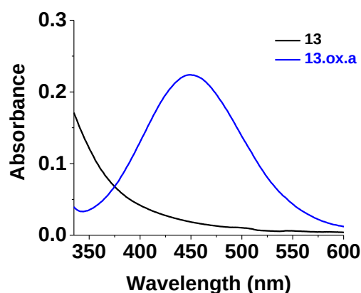
Figure III-10: UV-visible absorption spectra of 13 and 13.ox.a ; [13] = [13.ox.a] = 2.0 \times 10^{-2} M, solvent: MeOH, l = 1 cm.
