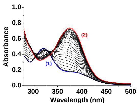
Figure II-28: UV-visible absorption spectrophotometric titration of 1Co as a function of pH; (1) pH: 7.57, (2) pH: 12.61, [L^1] = 6.89 \times 10^{-4} \text{ M} ; [Co] = 3.45 \times 10^{-4} \text{ M} ; solvent: dioxane:H 2 O (1:1 v/v); T = 25.0(2)^\circ\text{C} ; I = 0.1 \text{ M (NaClO}_4\cdot\text{H}_2\text{O)} ; l = 0.2 \text{ cm} .
