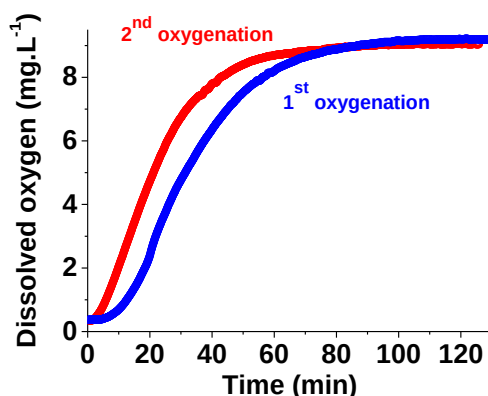
Figure II-46: Superimposition of the two oxygenation curves of 1Co during the oxygenation stages; [1Co] = 6 \times 10^{-4} \text{ M} , solvent: dioxane:H 2 O (1:1 v/v).
