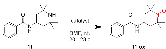
Scheme III-16: Oxidation of 11 by metal catalyst.
