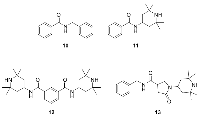
Scheme III-11: Organic model additives that have been investigated in this project.
