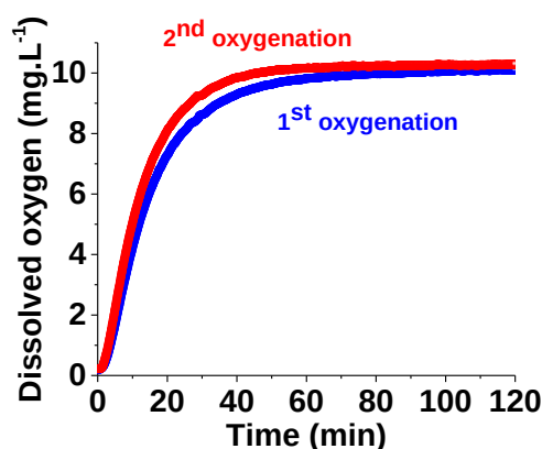
Figure II-49: Superimposition of the two oxygenation profiles of 1Co during the oxygenation stages; [1Co] = 4.79 \times 10^{-4} M , solvent: EtOH.
