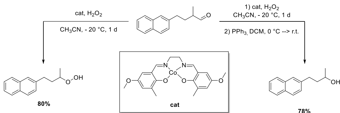
Scheme III-8: Transformation of aldehyde into alcohol or hydroperoxide catalysed by cobalt(II) Schiff base complex and related by the group of Iwasawa.
