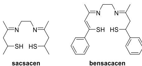
Scheme I-11: Examples of N_2S_2 ligand type.
