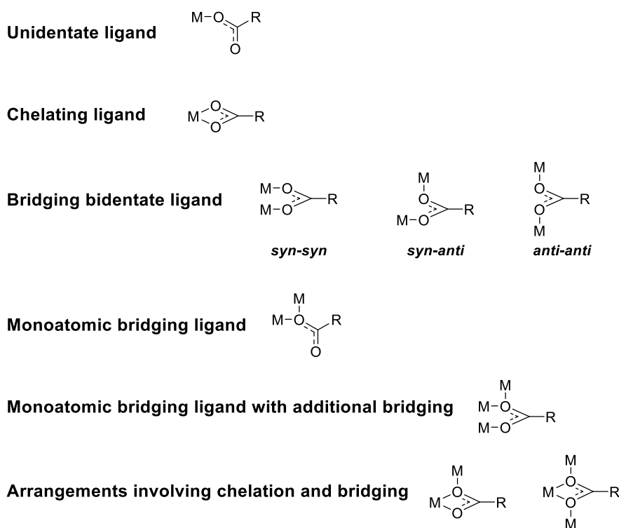
Scheme II-8: Chelating modes of carboxylate anions to metal centres.
