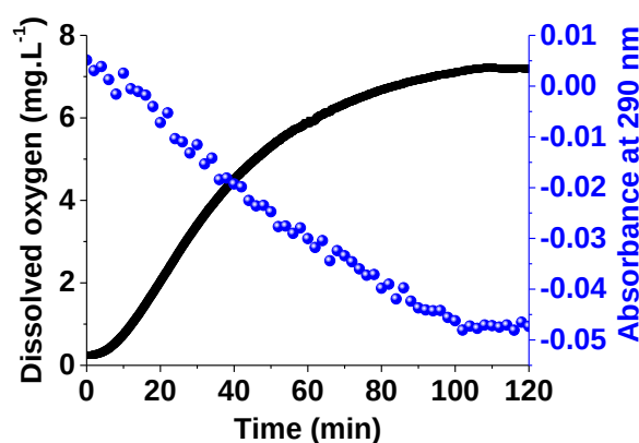
Figure II-40: Dissolved oxygen concentration and absorbance variation at 290 nm as a function of time for the first oxygenation stage of 8Co ; [8Co] = 2 \times 10^{-4} M, solvent: dioxane:H 2 O (1:1 v/v), l = 1 cm.
