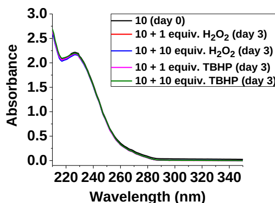
Figure III-1: Oxidation of 10 with H 2 O 2 (1 and 10 equiv.) and TBHP (1 and 10 equiv.) monitored by UV-visible absorption spectrophotometry; [ 10 ] = 9.70 × 10 -5 M, solvent: CH 3 CN:H 2 O (1:1 v/v), l = 1 cm.
