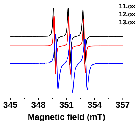
Figure III-6: EPR spectra of 11.ox , 12.ox.b and 13.ox.a at r.t. recorded on solutions; [ 11.ox ] = 3.2 \times 10^{-3} M, [ 12.ox.b ] = 2.2 \times 10^{-3} M, [ 13.ox.a ] = 2.1 \times 10^{-3} M, solvent: degassed DCM.
