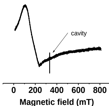
Figure II-21: EPR spectrum of cobalt(II) stearate 9Co-1 at 4 K.
