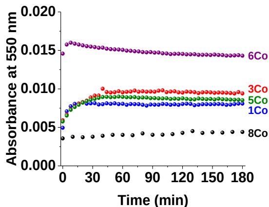
Figure II-34: Absorbance at 550 nm of 1Co , 3Co , 5Co , 6Co and 8Co over time; [ 1Co-6Co ] \sim 3 \times 10^{-4} M, solvent: dioxane, l = 1 cm; [ 8Co ] = 8.94 \times 10^{-5} M, solvent: dioxane:H 2 O (1:1 v/v), l = 1 cm.
