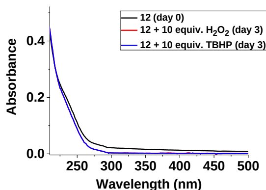
Figure III-4: Oxidation of 12 with \text{H}_2\text{O}_2 (10 equiv.) and TBHP (10 equiv.) followed by UV-visible absorption spectrophotometry; [ 12 ] = 1.06 \times 10^{-5} M, solvent: EtOH, l = 1 cm.
