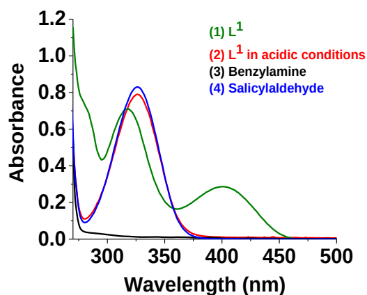
Figure II-11: UV-visible absorption spectra of L^1 in neutral and acidic conditions, benzylamine and salicylaldehyde; (1) [L^1] = 2.26 \times 10^{-4} M (pH = 8.6), (2) [L^1] = 2.20 \times 10^{-4} M (pH = 3.9), (3) [benzylamine] = 4.94 \times 10^{-2} M, (4) [salicylaldehyde] = 4.94 \times 10^{-4} M, solvent: dioxane:H 2 O (1:1 v/v), l = 1 cm.
