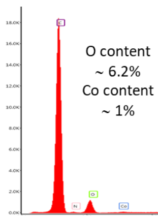
Figure IV-10: SEM-EDS analysis of 14 after oxidation with 9Co-1 at 70 °C.
