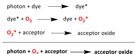
Scheme I-5: Photosensitive dye-based oxygen scavenger principle.
