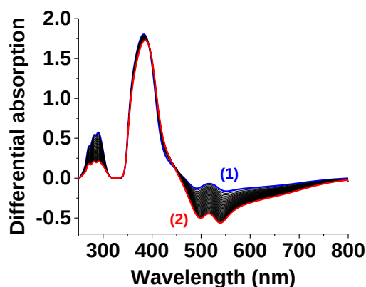
Figure II-64: Evolution of the UV-visible absorption spectra of 1Co with DPPH in open air conditions monitored over 3 h; (1): t = 0 , (2): t = 3 h, [1\text{Co}] = 2.92 \times 10^{-4} M, [1\text{Co}]/[\text{DPPH}] = 1.0 , solvent: dioxane, l = 1 cm, T = 25.0(2)^\circ\text{C} .
