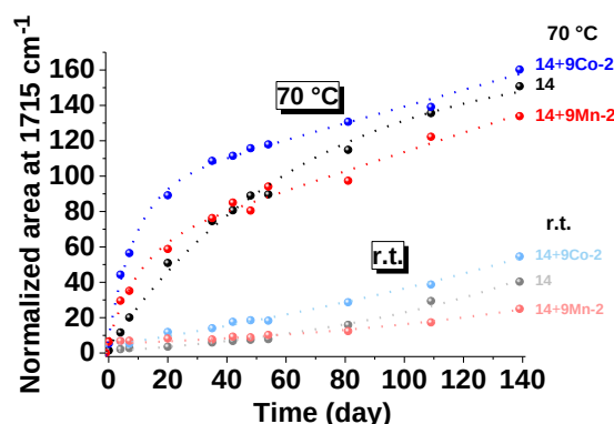
Figure IV-24: Normalized area at 1715 \text{cm}^{-1} representing the oxidation of 14 , with 9Co-2 and 9Mn-2 at r.t. and at 70 °C after 10 minutes of “extrusion”.
