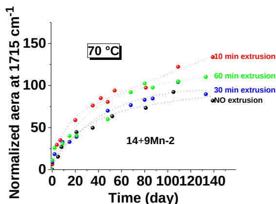
Figure IV-29: Normalized area at 1715 \text{cm}^{-1} representing the oxidation of 14 with 9Mn-2 at 70 °C after 0, 10, 30 and 60 minutes of “extrusion”.
