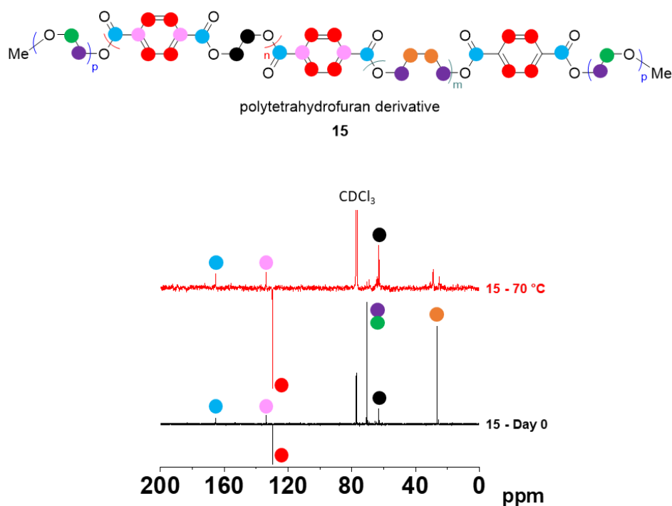
Figure IV-70: ^{13}\text{C} DEPT NMR spectra of non-oxidized polyTHF 15 before (black) and after (red) prolonged oxidation at 70 °C recorded in \text{CDCl}_3 at 500 MHz.
