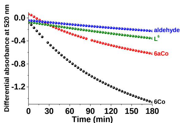
Figure II-71: Oxygenation/activation kinetics of the compound 6Co series probed by DPPH; [\text{Compounds}] \sim 3 \times 10^{-4}\text{M} , [\text{Compounds}]/[\text{DPPH}] = 1.0 , solvent: dioxane, l = 1\text{cm} , T = 25.0(2)^\circ\text{C} .
