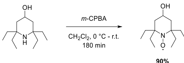
Scheme III-14: Oxidation of amine into nitroxide described by the group of Rajca.
