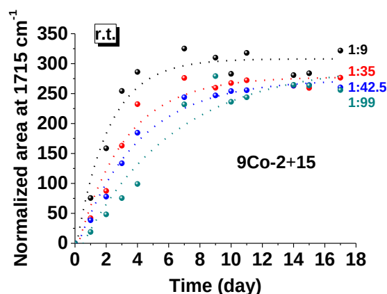
Figure IV-57: Normalized area at 1715\text{ cm}^{-1} showing the progress of the oxidation reaction of 15 with 9Co-2 at r.t. with different catalyst: additive ratios.
