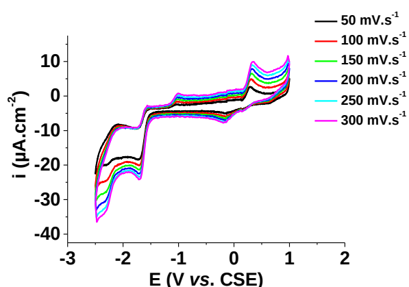
Figure II-74: CV voltammograms of complex 1Co measured at different scan rates; [\text{1Co}] = 9.74 \times 10^{-4} \text{ M} , solvent: DMSO, I = 0.1 \text{ M} ( n\text{-NBu}_4\text{PF}_6 ).
