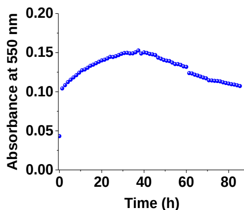
Figure II-36: Variation of the absorbance at 550 nm of 1Co as a function of time; [1\text{Co}] = 2.51 \times 10^{-3} \text{ M} , solvent: dioxane:H 2 O (1:1 v/v), l = 1 \text{ cm} .
