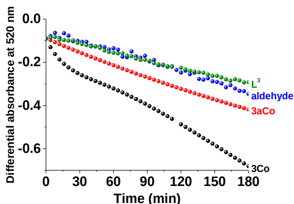
Figure II-69: Oxygenation/activation kinetics of the compound 3Co series probed by DPPH; [\text{Compounds}] \sim 3 \times 10^{-4}\text{M} , [\text{Compounds}]/[\text{DPPH}] = 1.0 , solvent: dioxane, l = 1\text{cm} , T = 25.0(2)^\circ\text{C} .
