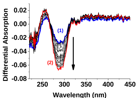
Figure II-41: Differential absorption spectra recorded during the second oxygenation stage of 8Co ; (1) t = 0 , (2) t = 2 h, [8Co] = 2 \times 10^{-4} M, solvent: dioxane:H 2 O (1:1 v/v), l = 1 cm.
