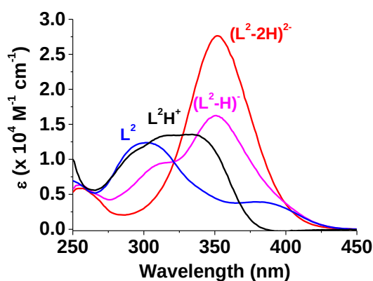
Figure II-17: Electronic spectra of the protonated L^2 species; [L^2] = 7.31 \times 10^{-5} M, solvent: dioxane:H 2 O (1:1 v/v), T = 25.0(2)^\circ\text{C} , I = 0.1 M (NaClO 4 .H 2 O), l = 1 cm.
