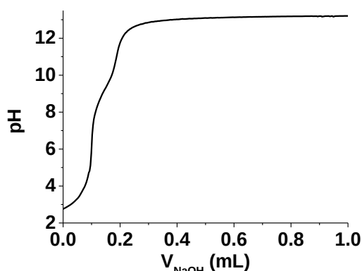
Figure II-18: Potentiometric titration curve of L 2 ; [ L 2 ] = 1.05 \times 10^{-3} M, solvent: dioxane:H 2 O (1:1 v/v), T = 25.0(2)^\circ\text{C} , I = 0.1 M (NaClO 4 .H 2 O).
