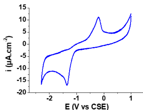
Figure II-73: CV voltammogram of free cobalt (cobalt(II) perchlorate) at 200 \text{ mV.s}^{-1} [\text{Co(II)}] = 1.13 \times 10^{-3} \text{ M} , solvent: DMSO, I = 0.1 \text{ M} ( n\text{-NBu}_4\text{PF}_6 ).
