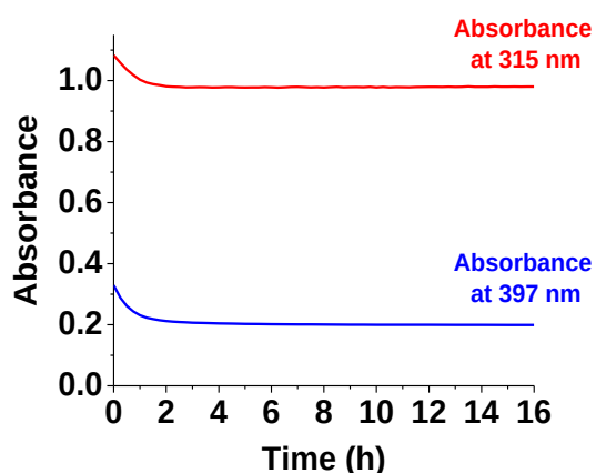
Figure II-6: Kinetics of the hydrolysis reaction of L^1 solution at 315 and 397 nm; [L^1] = 2.50 \times 10^{-4} M, solvent: dioxane: H_2O (1:1 v/v), l = 1 cm.
