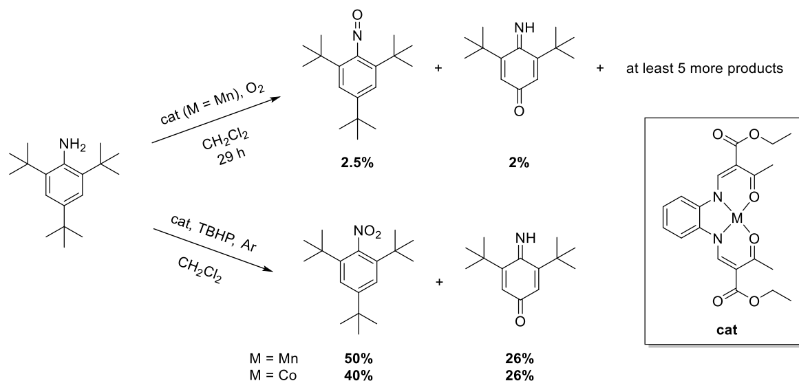
Scheme III-9: Oxidation of 2,4,6-tri-tert-butylaniline into 1,3,5-tri-tert-butyl-2-nitrosobenzene and 3,5-di-tert-butyl-4-iminocyclohexa-2,5-dien-1-one or 1,3,5-tri-tert-butyl-2-nitrobenzene and 3,5-di-tert-butyl-4-iminocyclohexa-2,5-dien-1-one catalysed by cobalt(II) and manganese(II) Schiff base catalysts and described by the group of Jäger; TBHP: tert -butylhydroperoxide.
