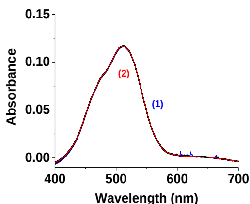
Figure II-32: UV-visible absorption spectra of cobalt(II) perchlorate measured over time; (1) t = 0 , (2) t = 24 h, [\text{Co}(\text{ClO}_4)_2 \cdot 6\text{H}_2\text{O}] = 2.51 \times 10^{-3} M, solvent: dioxane: \text{H}_2\text{O} (1:1 v/v); l = 1 cm.
