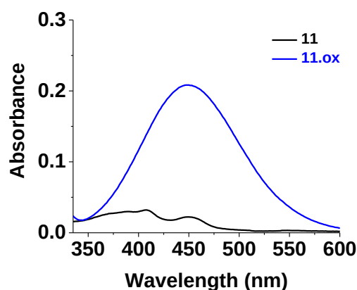
Figure III-8: UV-visible absorption spectra of 11 and 11.ox ; [11] = [11.ox] = 2.0 \times 10^{-2} M, solvent: MeOH, l = 1 cm.
