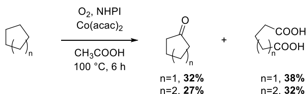
Scheme III-5: Oxidation of alkanes catalysed by cobalt(II)(acac) 2 described by Ishii, (NHPI: N-hydroxyphthalimide).
