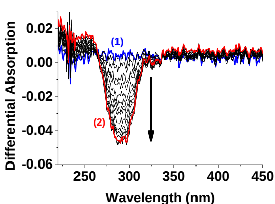
Figure II-39: Differential absorption spectra measured at regular intervals during the first oxygenation stage of 8Co ; (1) t = 0 , (2) t = 2 h, [8Co] = 2 \times 10^{-4} M, solvent: dioxane:H 2 O (1:1 v/v), l = 1 cm.
