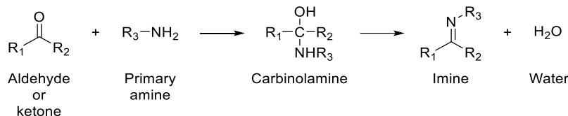
Scheme I-8: Formation of a Schiff base from an aldehyde or a ketone and an amine.
