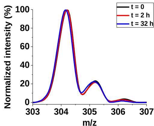
Figure II-8: Stability of a L^2 solution over time (zoom on the [L^2+H]^+ peak centred at m/z = 304.2 ); [ L^2 ] = 1.0 \times 10^{-4} M; solvent: CH_3CN:H_2O (1:1 v/v); + 100 V.
