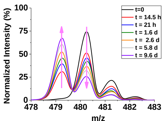
Figure II-55: ESI-MS spectra of 1Co recorded over 10 days - zoom between m/z = 478 and 483 ; [\text{1Co}] = 1.0 \times 10^{-4} M, solvent: \text{CH}_3\text{CN}:\text{H}_2\text{O} (1:1 v/v), + 170 V.
