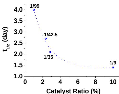
Figure IV-58: Half-life times of the oxidation reaction of 15 in the presence of 9Co-2 at r.t. as a function of the catalyst: additive ratio.
