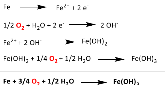
Scheme I-1: Iron-based oxygen scavenger principle.
