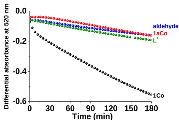
Figure II-67: Oxygenation/activation kinetics of the 1Co series probed by DPPH; [Compounds] \sim 3 \times 10^{-4} M , [Compounds]/[DPPH] = 1.0 , solvent: dioxane, l = 1 \text{ cm} , T = 25.0(2)^\circ C .
