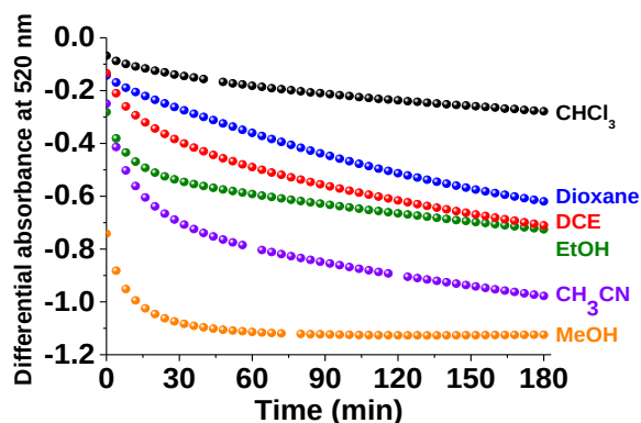
Figure II-66: Oxygenation/activation kinetics of the complex 1Co probed by DPPH in different solvents; [1Co] \sim 3 \times 10^{-4} M , [1Co]/[DPPH] = 1.0 , l = 1 \text{ cm} , T = 25.0(2)^\circ C .
