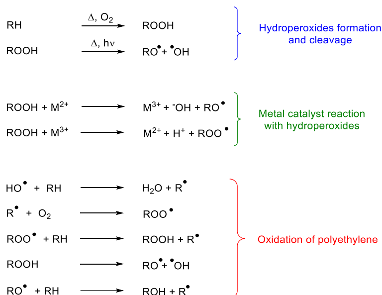
Scheme IV-6: Putative thermo-oxidative degradation of HDPE that may account for our observations (from Maryudi 190 )
