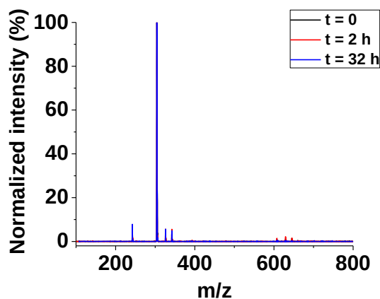
Figure II-7: Stability of a L^2 solution assessed by ESI-MS; [ L^2 ] = 1.0 \times 10^{-4} M; solvent: CH_3CN:H_2O (1:1 v/v); + 100 V.
