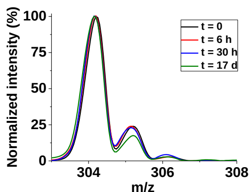
Figure II-58: ESI-MS spectra of 2Co recorded over 17 d - zoom between m/z = 303 and 308 ; [2Co] = 1.0 \times 10^{-4} M, solvent: CH_3CN:H_2O (1:1 v/v), + 225 V.
