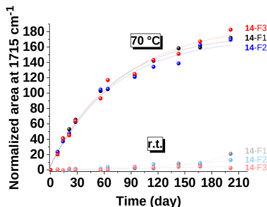
Figure IV-16: Normalized area at 1715 cm⁻¹ illustrating the oxidation reaction of the three-different particle size distributions of 14 alone at r.t. and at 70 °C.
