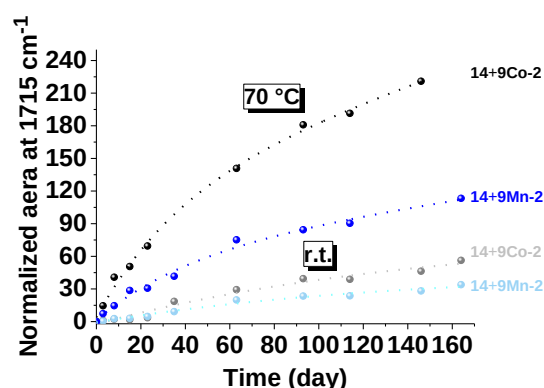
Figure IV-31: Normalized area at 1715 cm -1 representing the oxidation process of 14 in the presence of either 9Co-2 or 9Mn-2 at r.t. and at 70 °C after 10 minutes of catalyst "extrusion" at 100 °C.
