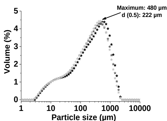
Figure IV-11: Laser diffraction granulometry of 14 after grinding and before sieving.
