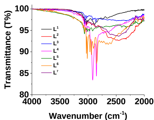
Figure II-1: FTIR spectra - expansion of the 4000 - 2000 \text{cm}^{-1} wavenumber range - of the Schiff base ligands investigated in this work.
