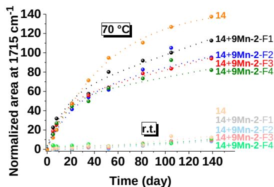
Figure IV-22: Normalized area at 1715 \text{cm}^{-1} describing the oxidation process of 14 with the four different particle size distributions of 9Mn-2 at r.t. and at 70 °C.
