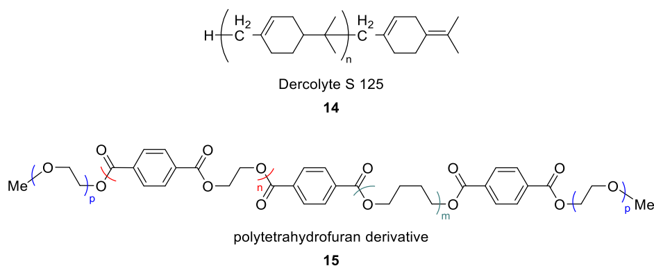
Scheme IV-1: Polymeric additives investigated in this Ph.D. work.
