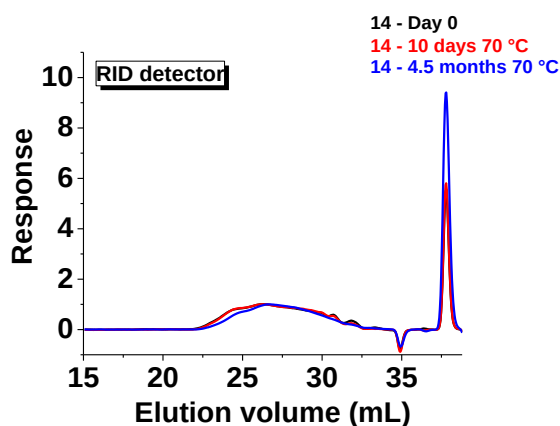
Figure IV-49: SEC measurements of non-oxidized 14 before (black) and after 10 days (red) and 4.5 months (blue) of oxidation at 70 °C - refractive index detector (RID).
