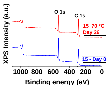
Figure IV-63: XPS survey scans of 15 .
