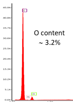
Figure IV-8: SEM-EDS analysis of fresh 14 .
