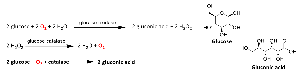
Scheme I-3: Enzyme-based oxygen scavenger principle (glucose oxidase/catalase).
