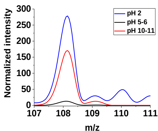
Figure II-13: ESI-MS spectra of L^1 at different pH conditions (zoom on the [benzylamine+H] + peak centred at m/z = 108.1 ); [L^1] = 9.0 \times 10^{-5} M, solvent: CH 3 CN:H 2 O (1:1 v/v), + 100 V.
