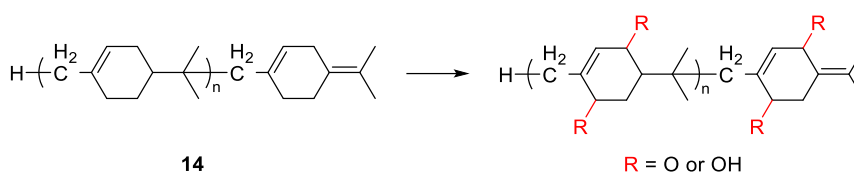
Scheme IV-2: Proposed metal catalyst-assisted aerobic oxidation route of the polymeric additive 14 .
