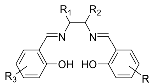
Scheme I-10: Salen-type ligand.
