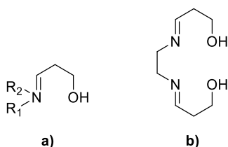
Scheme I-9: Schiff base in coordination chemistry.
