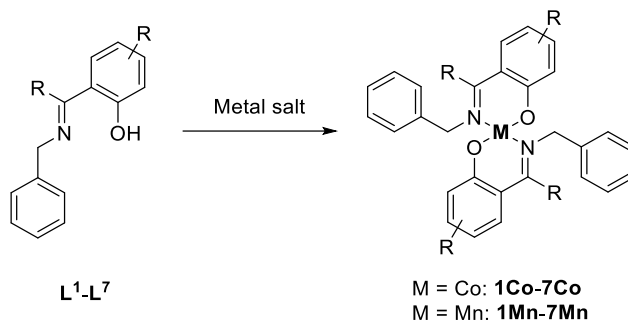
Scheme II-5: Synthetic approach for the preparation of the targeted cobalt(II) and manganese(II) catalysts - ligand/metal version.
