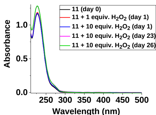
Figure III-3: Oxidation of 11 with \text{H}_2\text{O}_2 (1 and 10 equiv.) monitored by UV-visible absorption spectrophotometry; [ 11 ] = 1.05 \times 10^{-4} M, solvent: \text{CH}_3\text{CN}:\text{H}_2\text{O} (1:1 v/v), l = 1 cm.
