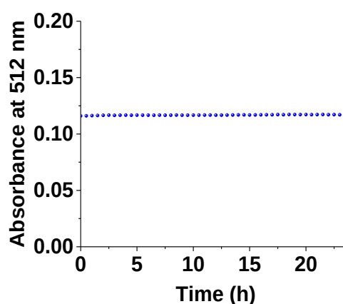
Figure II-33: Absorbance at 512 nm as a function of time; [\text{Co}(\text{ClO}_4)_2 \cdot 6\text{H}_2\text{O}] = 2.51 \times 10^{-3} M, solvent: dioxane: \text{H}_2\text{O} (1:1 v/v); l = 1 cm.
