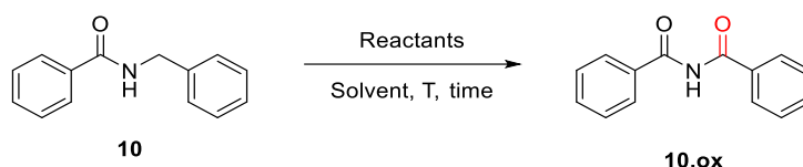
Scheme III-13: Oxidation of N-phenylmethylbenzamide 10 into N-benzoylbenzamide 10.ox .
