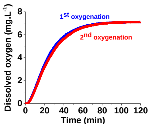
Figure II-52: Superimposition of the two oxygenation profiles of 9Co during the oxygenation stages; [9Co] = 5.91 \times 10^{-4} M , solvent: iso-butanol.
