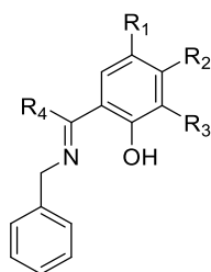
Scheme I-14: Schiff base ligands studied in this work.
