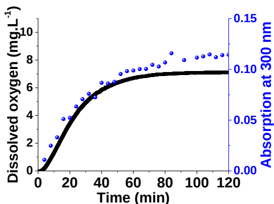
Figure II-50: Dioxygen concentration and absorbance at 300 nm recorded as a function of time for the first oxygenation stage of 9Co ; [9Co] = 5.91 \times 10^{-4} M , solvent: iso-butanol, l = 1 cm.
