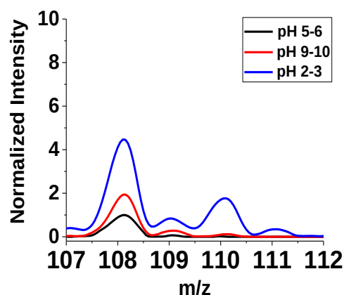
Figure II-15: ESI-MS spectra of L 6 in different pH conditions (zoom on the [benzylamine+H] + peak centred at m/z = 108.1 ); [ L 6 ] = 1.06 \times 10^{-4} M, solvent: CH 3 CN:H 2 O (1:1 v/v), + 150 V.
