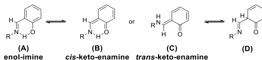
Scheme II-3: Keto-enol equilibrium.
