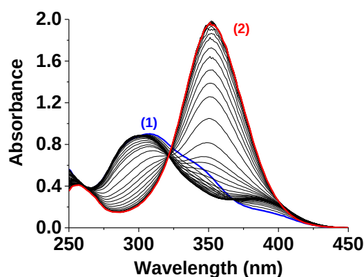
Figure II-16: UV-visible absorption spectrophotometric titration of the free L^2 ligand as a function of pH; (1) pH: 4.00, (2) pH: 12.54, [L^2] = 7.31 \times 10^{-5} M, solvent: dioxane:H 2 O (1:1 v/v), T = 25.0(2)^\circ\text{C} , I = 0.1 M (NaClO 4 .H 2 O), l = 1 cm.
