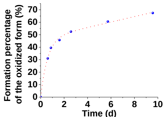
Figure II-56: Formation percentage of the oxidized form of 1Co over 10 days.
