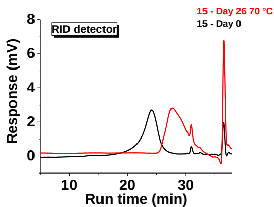
Figure IV-71: SEC measurements of non-oxidized polyTHF 15 before (black) and after (red) prolonged oxidation at 70 °C - refractive index detector (RID).
