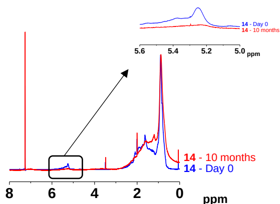
Figure IV-51: ^1\text{H} NMR of 14 , \text{CDCl}_3 , 400 MHz.
