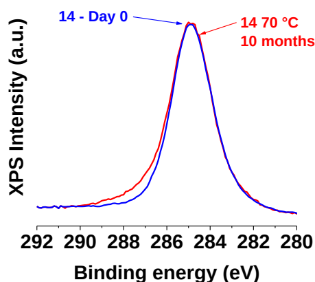
Figure IV-44: XPS C 1s scans of 14 .
