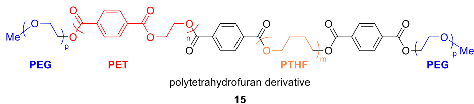
Scheme IV-4: Chemical structure of the polymeric additive 15 .
