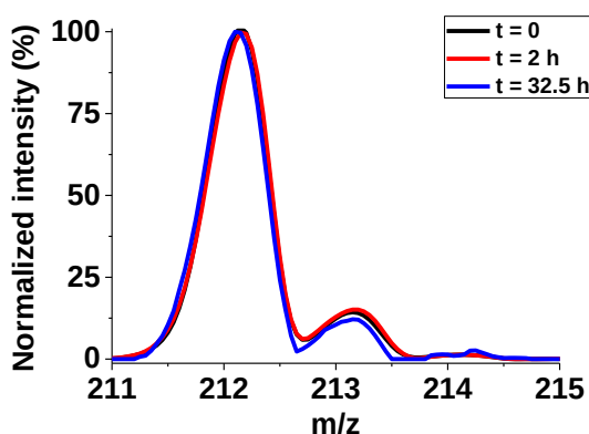
Figure II-3: Stability of a L^1 solution over time (zoom on the [L^1+H]^+ peak centred at m/z = 212.1 ); [L^1] = 1.0 \times 10^{-4} M; solvent: CH_3CN:H_2O (1:1 v/v); + 100 V.
