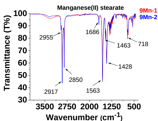
Figure II-22: FTIR spectra of manganese(II) stearate 9Mn .
