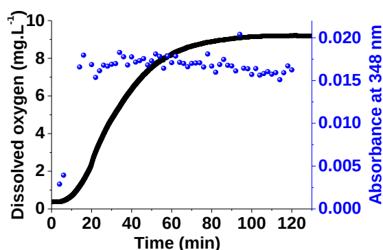
Figure II-44: Dioxygen concentration and absorbance at 348 nm as a function of time for the first oxygenation stage of 1Co ; [1Co] = 6 \times 10^{-4} M , solvent: dioxane:H 2 O (1:1 v/v), l = 1 cm.
