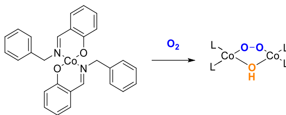
Scheme II-10: Oxygenation reaction for 1Co .
