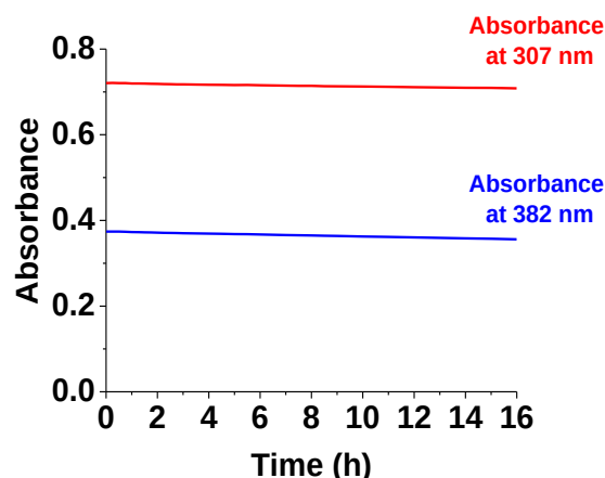
Figure II-10: Kinetics of the hydrolysis reaction of a L^2 solution at 307 and 382 nm; [ L^2 ] = 5.02 \times 10^{-5} M, solvent: dioxane: H_2O (1:1 v/v), l = 1 cm.
