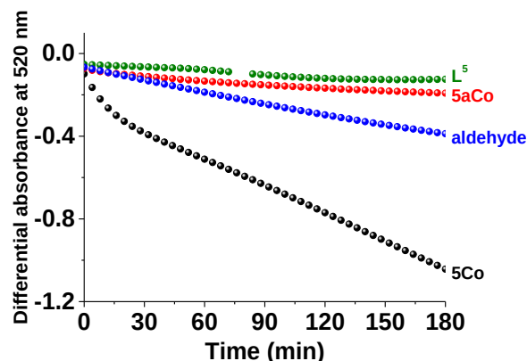
Figure II-70: Oxygenation/activation kinetics of the compound 5Co series probed by DPPH; [\text{Compounds}] \sim 3 \times 10^{-4}\text{M} , [\text{Compounds}]/[\text{DPPH}] = 1.0 , solvent: dioxane, l = 1\text{cm} , T = 25.0(2)^\circ\text{C} .
