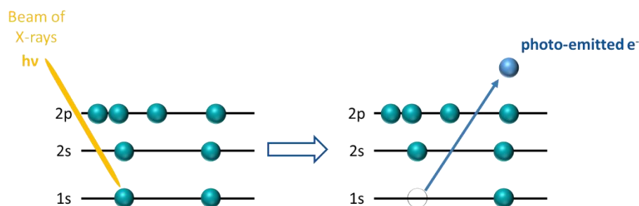
Figure IV-74: XPS principle.
