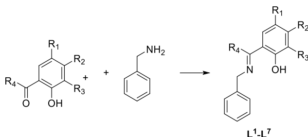
Scheme II-1: Synthesis of the Schiff base ligands investigated in this work.
