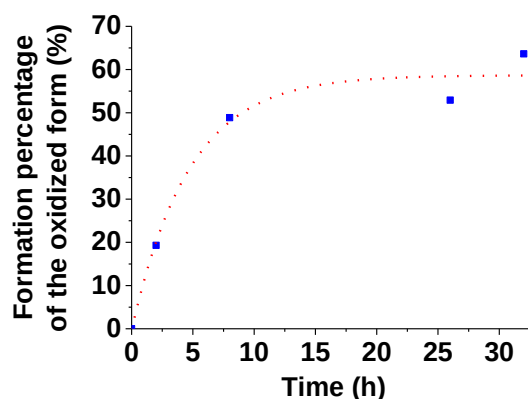
Figure II-54: Formation percentage of the oxidized form of 1Co over a time span of 32 h.
