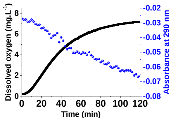
Figure II-42: Dissolved oxygen concentration and absorbance variation at 290 nm as a function of time for the second oxygenation stage of 8Co ; [8Co] = 2 \times 10^{-4} M, solvent: dioxane:H 2 O (1:1 v/v), l = 1 cm.
