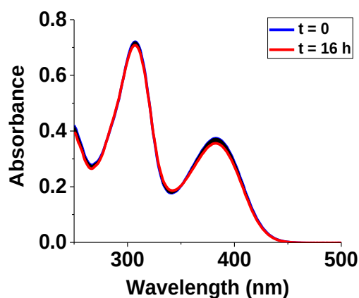
Figure II-9: Stability of a L^2 solution monitored by UV-visible absorption spectrophotometry for 16 hours; [ L^2 ] = 5.02 \times 10^{-5} M, solvent: dioxane: H_2O (1:1 v/v), l = 1 cm.
