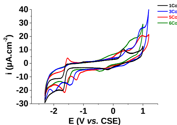
Figure II-75: CV voltammograms of complexes 1Co , 3Co , 5Co and 6Co ; [Complex] \sim 1 \times 10^{-3} M, solvent: DMSO, I = 0.1 M (n-NBu 4 PF 6 ).
