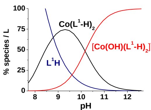
Figure II-30: Distribution diagrams of the protonated cobalt(II) L^1 species; [L^1] = 6.89 \times 10^{-4} \text{ M} ; [Co] = 3.45 \times 10^{-4} \text{ M} ; solvent: dioxane:H 2 O (1:1 v/v); T = 25.0(2)^\circ\text{C} ; I = 0.1 \text{ M (NaClO}_4\cdot\text{H}_2\text{O)} .
