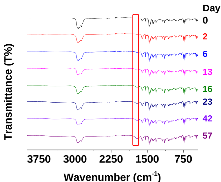
Figure IV-3: Oxidation of 14 in the presence of 1Co ( 1Co:14 , 1:35 w/w) probed by FTIR; the samples were stored at 70 °C.
