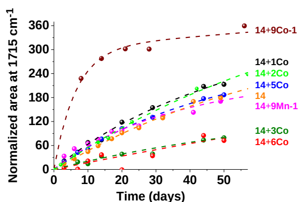
Figure IV-4: Normalized area at 1715 \text{cm}^{-1} representing the oxidation of 14 at 70 °C with the different metal catalysts considered in this work. The dash lines correspond to the first order processing of the data.
