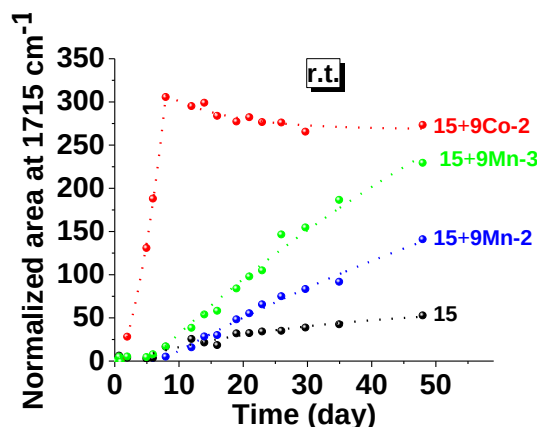
Figure IV-55: Normalized area at 1715\text{ cm}^{-1} describing the oxidation of 15 either alone or with 9Co-2 , 9Mn-2 or 9Mn-3 at r.t..
