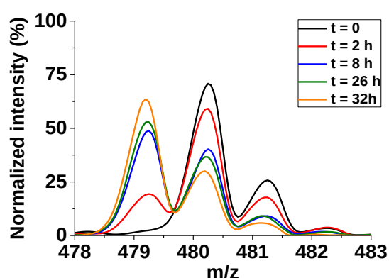
Figure II-53: ESI-MS spectra of 1Co recorded over 32 h - zoom between m/z = 478 and 483 ; [\text{1Co}] = 1.0 \times 10^{-4} M, solvent: \text{CH}_3\text{CN}:\text{H}_2\text{O} (1:1 v/v), + 170 V.
