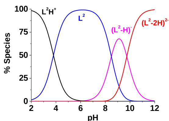
Figure II-19: Distribution diagrams of the protonated L 2 species; [ L 2 ] = 7.31 \times 10^{-5} M, solvent: dioxane:H 2 O (1:1 v/v), T = 25.0(2)^\circ\text{C} , I = 0.1 M (NaClO 4 .H 2 O), l = 1 cm.
