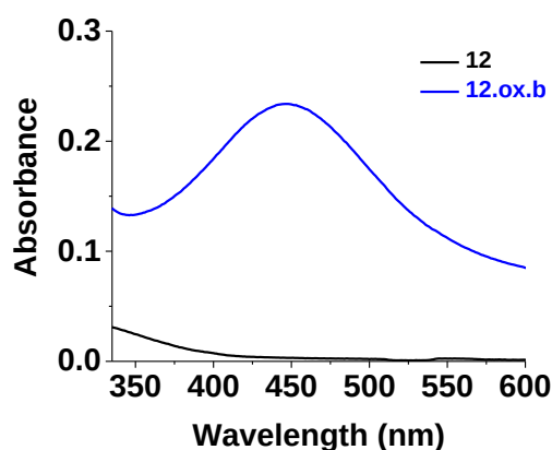
Figure III-9: UV-visible absorption spectra of 12 and 12.ox.b ; [12] = [12.ox.b] = 2.0 \times 10^{-2} M, solvent: MeOH, l = 1 cm.
