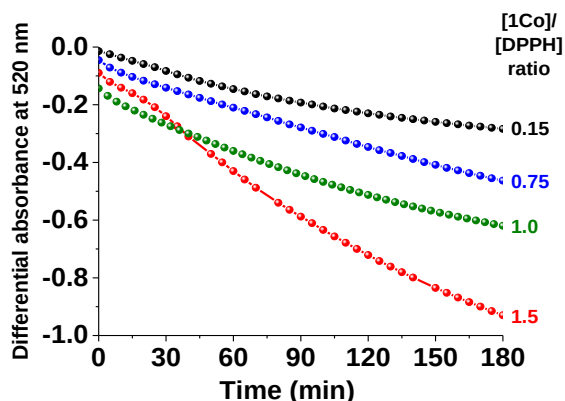
Figure II-65: Oxygenation/activation kinetics of the compound 1Co probed by DPPH with various [1\text{Co}]/[\text{DPPH}] ratios; [1\text{Co}] \sim 3 \times 10^{-4} M, [1\text{Co}]/[\text{DPPH}] = 0.15\text{--}1.5 , solvent: dioxane, l = 1 cm, T = 25.0(2)^\circ\text{C} .
