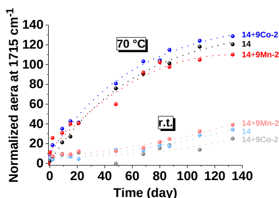
Figure IV-26: Normalized area at 1715 cm -1 showing the oxidation reaction of 14 , with 9Co-2 and 9Mn-2 at r.t. and at 70 °C following an “extrusion” process of 1 hour.
