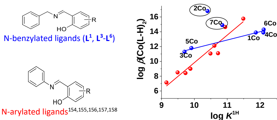
Figure II-31: Relationships between the global stability constants of the cobalt(II) complexes and the acido-basic properties of a broad range of Schiff bases including those of interest in the frame of this study.
