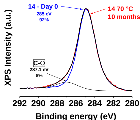
Figure IV-45: XPS – deconvolution of C 1s scans of 14 .
