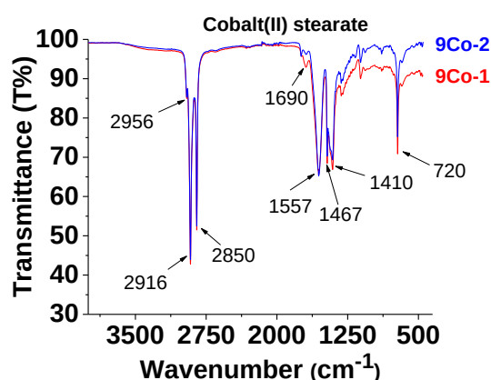
Figure II-20: FTIR spectra of cobalt(II) stearate 9Co .
