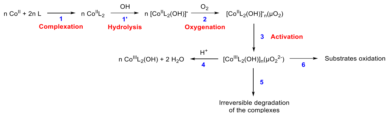
Scheme I-12: Putative mechanism of complexation, oxygenation and activation of cobalt(II) complexes. Main steps are noted 1 to 6. Adapted from Cabani.
