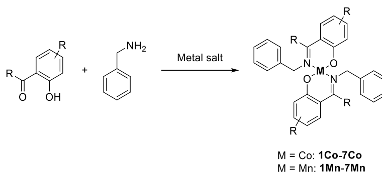
Scheme II-6: Synthetic approach for the preparation of the cobalt(II) and manganese(II) catalysts - one-pot version.
