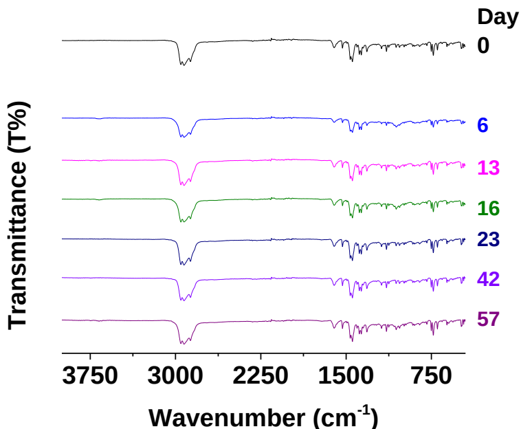
Figure IV-2: Oxidation of 14 in the presence of 1Co ( 1Co:14 , 1:35 w/w) monitored by FTIR; the samples were stored at r.t..
