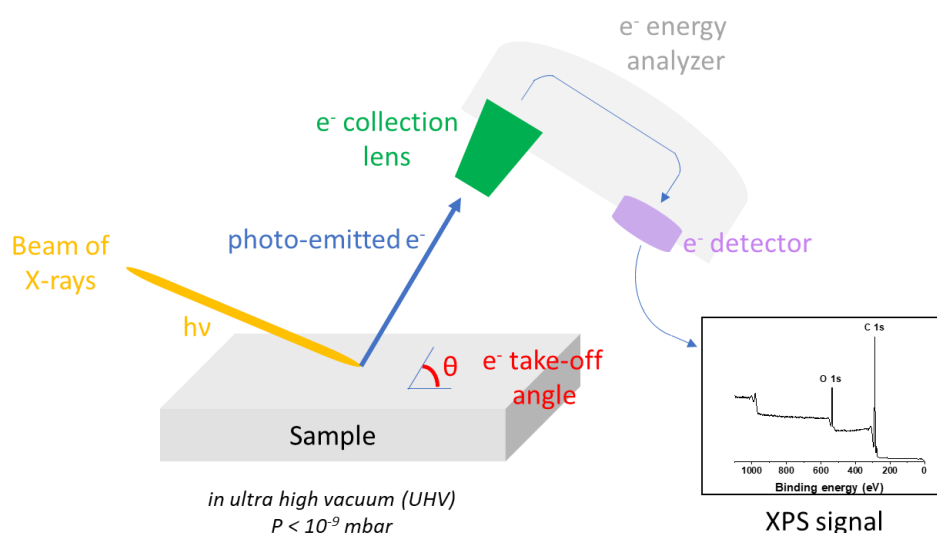
Figure IV-75: XPS equipment.
