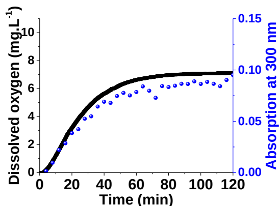
Figure II-51: Dioxygen concentration and absorbance at 300 nm recorded as a function of time for the second oxygenation stage of 9Co ; [9Co] = 5.91 \times 10^{-4} M , solvent: iso-butanol, l = 1 cm.
