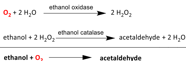
Scheme I-4: Enzyme-based oxygen scavenger principle (ethanol oxidase/catalase).
