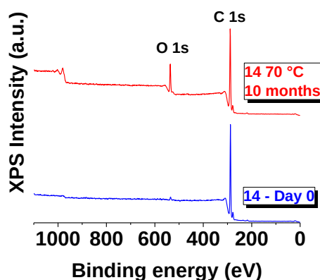
Figure IV-43: XPS survey scans of 14 .
