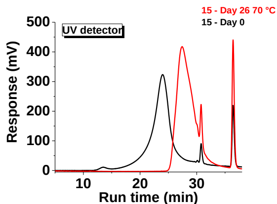
Figure IV-72: SEC measurements of non-oxidized polyTHF 15 before (black) and after (red) prolonged oxidation at 70 °C - UV detector.
