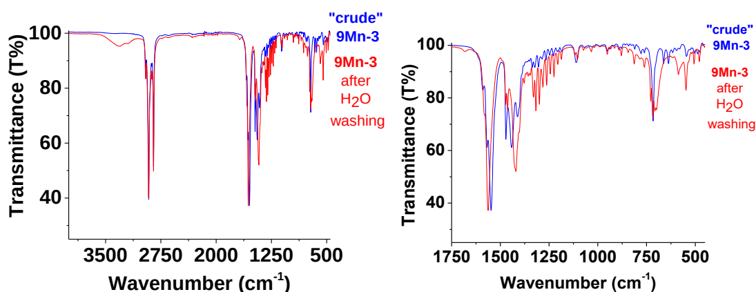
Figure II-26: FTIR spectra of the complex 9Mn-3 without any purification and after water washing.
