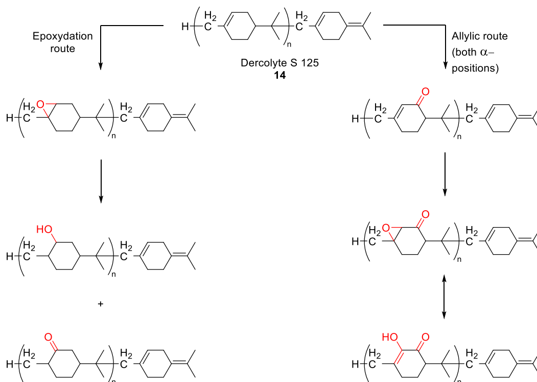
Scheme IV-3: Suggested oxidized products among other and their putative mechanism of formation. For the allylic oxidation, the two \alpha -positions can be involved. As an example, only the products resulting from one \alpha -position are described in the scheme.
