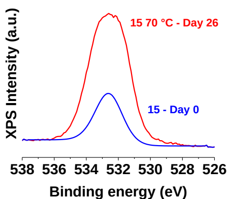
Figure IV-66: XPS O 1s scans of 15 .
