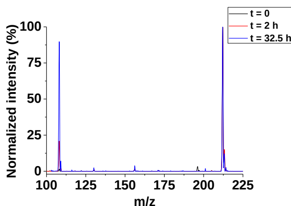
Figure II-2: Stability of a solution of \text{L}^1 monitored by ESI-MS; [\text{L}^1] = 1.0 \times 10^{-4} \text{ M} ; solvent: \text{CH}_3\text{CN}:\text{H}_2\text{O} (1:1 v/v); + 100 V.
