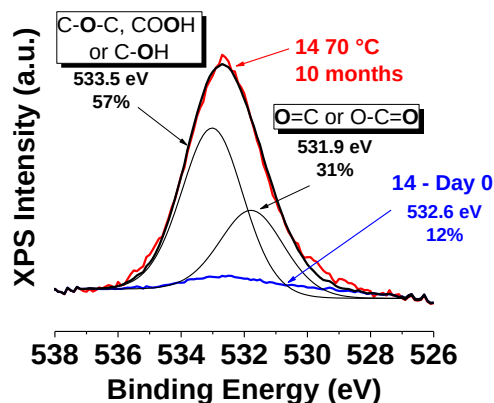
Figure IV-47: XPS – deconvolution of O 1s scans of 14 .
