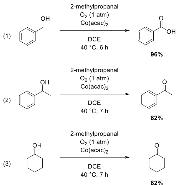
Scheme III-2: Oxidation of alcohols into ketones or carboxylic acid catalysed by cobalt(II)(acac) 2 and described by the group of Mastorilli.
