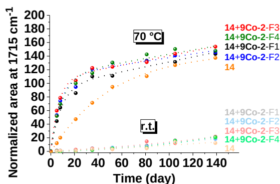
Figure IV-21: Normalized area at 1715 \text{cm}^{-1} illustrating the oxidation process of 14 with the four different particle size distributions of 9Co-2 at r.t. and at 70 °C.
