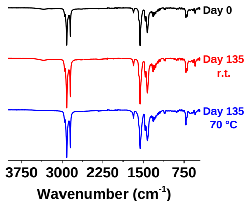
Figure IV-35: FTIR spectra of 14:9Mn-2 (1:2 w/w).
