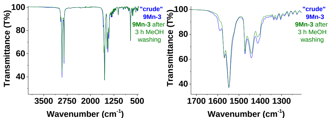
Figure II-27: FTIR spectra of the complex 9Mn-3 without any purification and after methanol washing.
