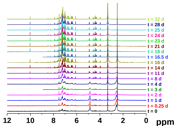
Figure II-62: ^1\text{H} NMR spectra of 1\text{Co} recorded over time; solvent: (\text{CD}_3)_2\text{SO} .
