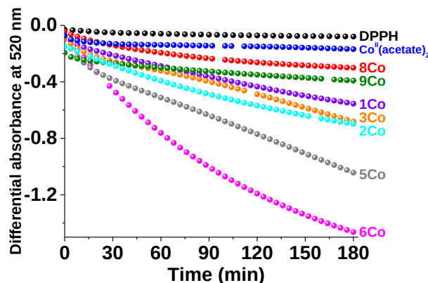
Figure II-72: Reactivity (oxygenation/activation) of the different cobalt(II) complexes probed with DPPH; [Complex] \sim 3 \times 10^{-4} M, [Complex]/[DPPH] = 1.0, solvent: dioxane, l = 1 cm, T = 25.0(2)^\circ\text{C} .
