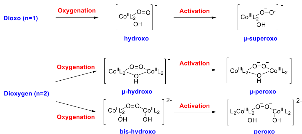
Scheme I-13: Chemical structures of the key oxygenated cobalt(II)/cobalt(III) species.
