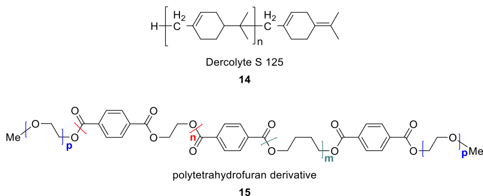
Scheme I-19: Polymeric additives studied in this work.
