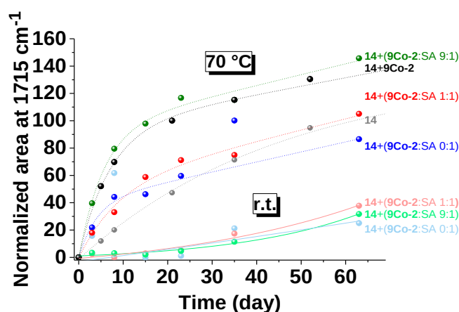
Figure IV-39: Normalized area at 1715\text{ cm}^{-1} representing the oxidation of 14 with 9Co-2 at r.t. and at 70\text{ }^{\circ}\text{C} in the absence and in the presence of stearic acid (SA).
