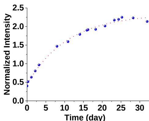
Figure II-63: Kinetics of oxidation of 1Co and conversion to its cobalt(III) trischelate monitored by ^1\text{H} NMR; solvent: (\text{CD}_3)_2\text{SO} .
