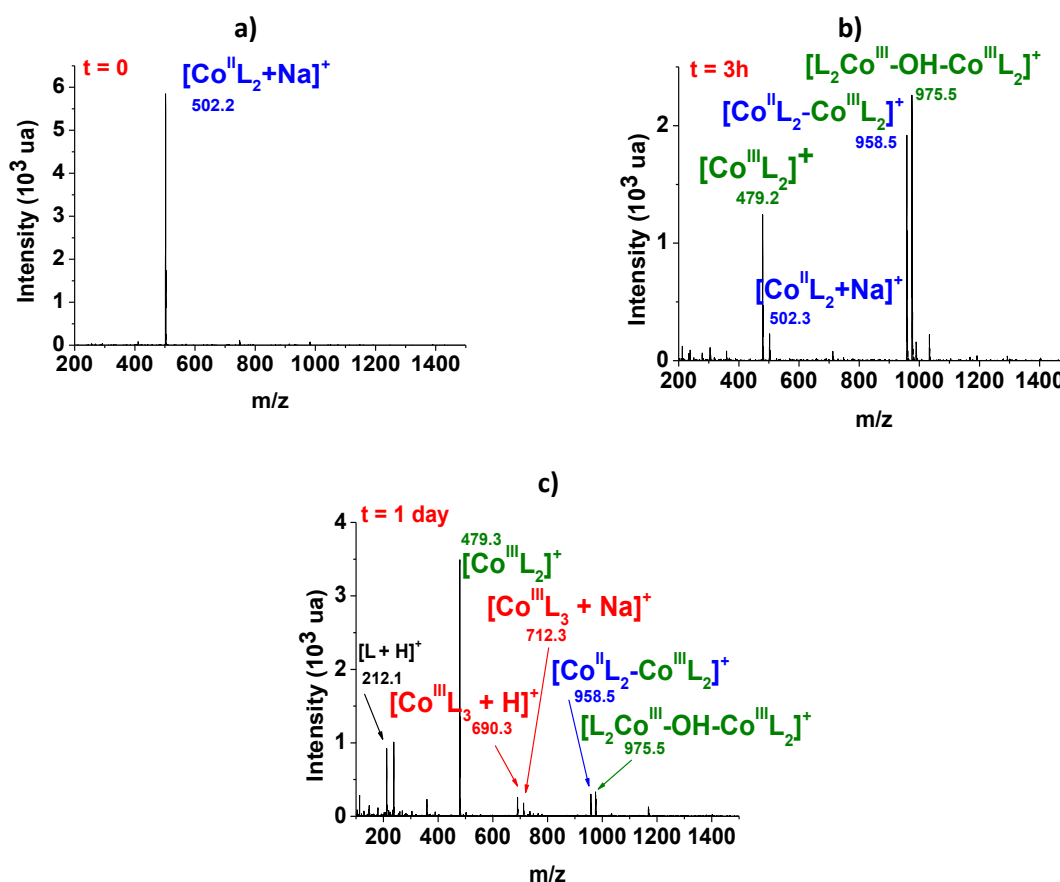
Figure II-57: Full ESI-MS spectra of 1Co recorded over one day; a) t = 0 , b) t = 3 h, c) t = 1 day, [\mathbf{1Co}] = 6.97 \times 10^{-4} M, solvent: dioxane, + 100 V.
