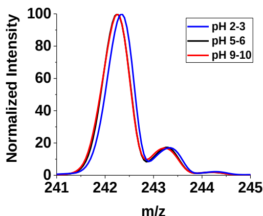
Figure II-14: ESI-MS spectra of L 6 in different pH conditions (zoom on the [ L 6 +H] + peak centred at m/z = 242.1 ); [ L 6 ] = 1.06 \times 10^{-4} M, solvent: CH 3 CN:H 2 O (1:1 v/v), + 150 V.
