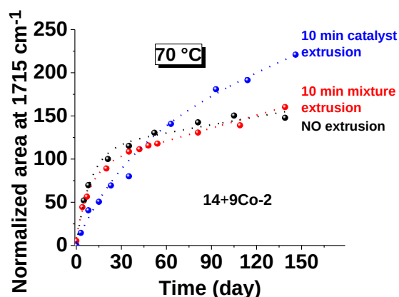
Figure IV-32: Normalized area at 1715\text{ cm}^{-1} representing the oxidation of 14 with 9Co-2 at 70\text{ }^{\circ}\text{C} after 0 or 10 minutes of “extrusion” of the catalyst/ 14 additive and after 10 minutes of “extrusion” of only the catalyst.
