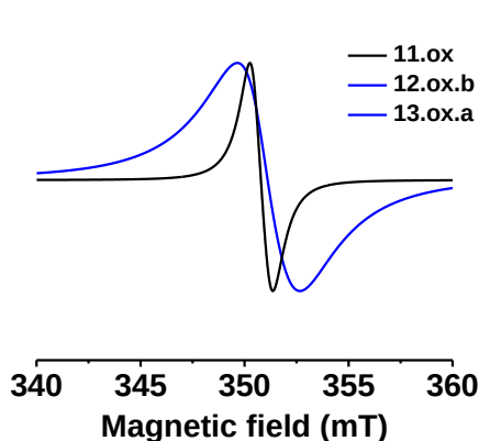
Figure III-5: EPR spectra of 11.ox , 12.ox.b and 13.ox.a at r.t. recorded on powders.
