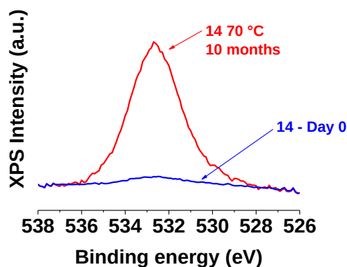
Figure IV-46: XPS O 1s scans of 14 .
