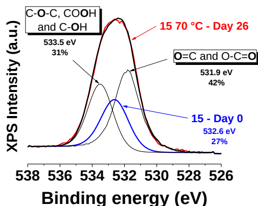
Figure IV-67: XPS – deconvolution of O 1s scans of 15 .
