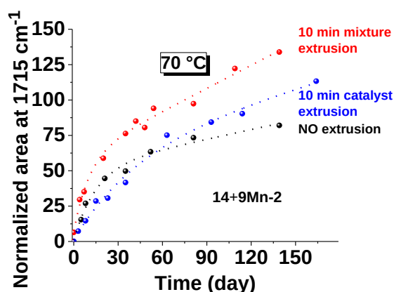
Figure IV-33: Normalized area at 1715\text{ cm}^{-1} representing the oxidation of 14 with 9Mn-2 at 70\text{ }^{\circ}\text{C} after 0 or 10 minutes of “extrusion” of the catalyst/ 14 additive and 10 minutes of “extrusion” of only the catalyst.
