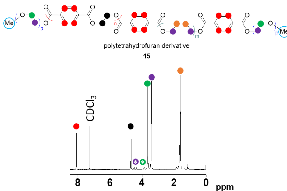
Figure IV-68: ^1\text{H} NMR spectrum of non-oxidized 15 measured in \text{CDCl}_3 at 500 MHz. * indicated terminal residues of the polymer.
