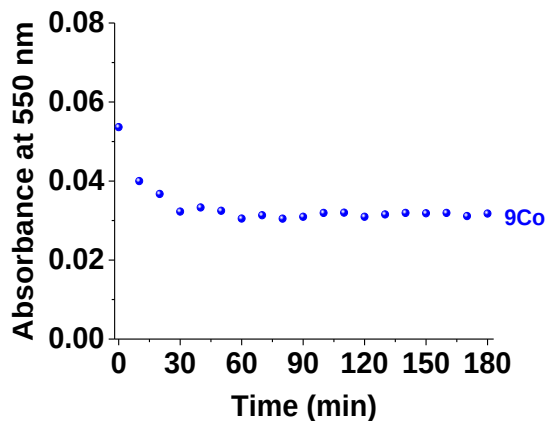
Figure II-35: Absorbance at 550 nm of 9Co over time; [ 9Co ] = 9.52 \times 10^{-4} M, solvent: iso -butanol, l = 1 cm.
