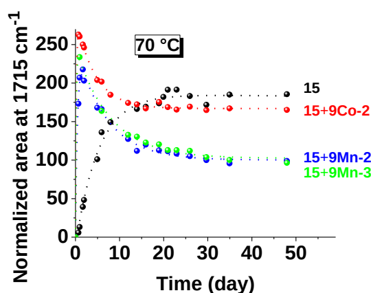
Figure IV-62: Normalized area at 1715\text{ cm}^{-1} representing the oxidation of 15 either alone or with 9Co-2 , 9Mn-2 or 9Mn-3 at 70\text{ }^{\circ}\text{C} .
