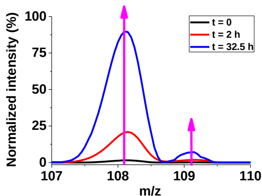
Figure II-4: Stability of a L^1 solution over time (zoom on the [benzylamine+H]^+ peak centred at m/z = 108.1 ); [L^1] = 1.0 \times 10^{-4} M; solvent: CH_3CN:H_2O (1:1 v/v); + 100 V.
