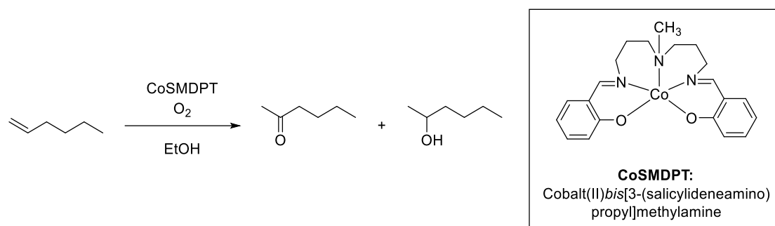
Scheme III-7: Oxidation of hex-1-ene into hexan-2-one and hexan-2-ol catalysed by cobalt(II)SMDPT and described by the group of Drago.
