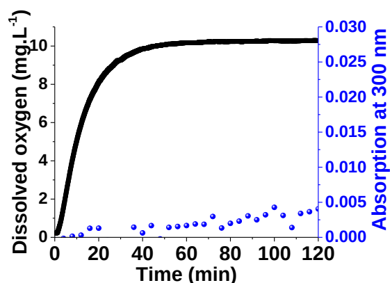
Figure II-48: Dioxygen concentration and absorbance variation at 300 nm recorded as a function of time for the second oxygenation stage with 1Co ; [1Co] = 4.79 \times 10^{-4} M , solvent: EtOH, l = 1 cm.
