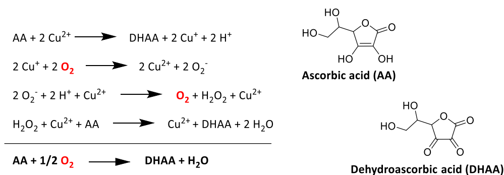
Scheme I-2: Ascorbic acid-based oxygen scavenger principle.
