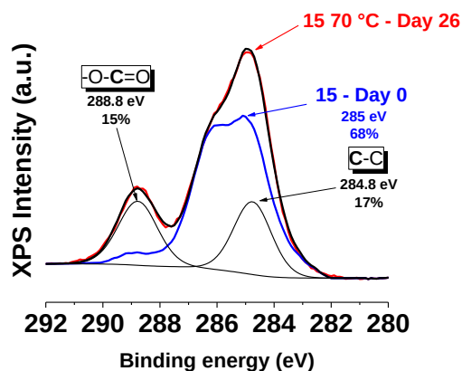
Figure IV-65: XPS – deconvolution of C 1s scans of 15 .
