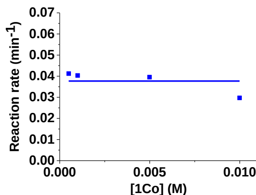
Figure II-38: Variation of the rate constants associated to the oxygenation of 1Co as a function of metal catalyst concentrations; solvent: dioxane:H 2 O (1:1 v/v), l = 1 \text{ cm} .
