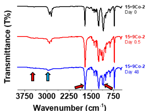
Figure IV-61: FTIR spectra of 15 at day 0 and after 0.5 and 48 days of aerobic oxidation with 9Co-2 at 70\text{ }^{\circ}\text{C} .
