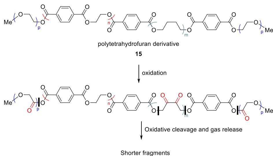
Scheme IV-5: Putative oxidation sites and products formed from oxidative cleavage of 15 . The bold black lines indicate the potential cleavage points.
