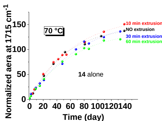
Figure IV-27: Normalized area at 1715 cm -1 representing the oxidation reaction of 14 at 70 °C after 0, 10, 30 and 60 minutes of “extrusion”.
