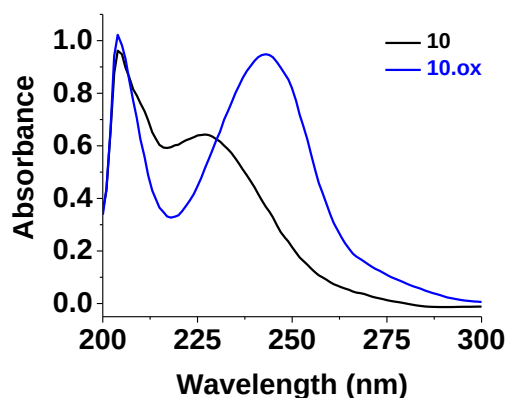
Figure III-7: UV-visible absorption spectra of 10 and 10.ox ; [10] = [10.ox] = 2.0 \times 10^{-5} M, solvent: MeOH, l = 1 cm.
