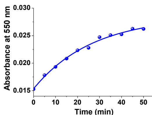
Figure II-37: Variation of the absorbance at 550 nm of 1Co as a function of time; [1\text{Co}] = 5 \times 10^{-4} \text{ M} , solvent: dioxane:H 2 O (1:1 v/v), l = 1 \text{ cm} .
