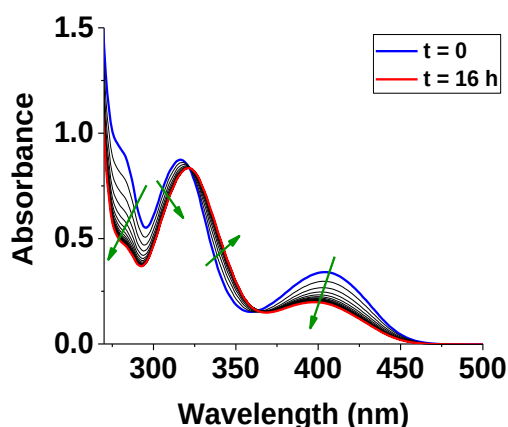
Figure II-5: Stability of a L^1 solution monitored by UV-visible absorption over 16 hours; [L^1] = 2.50 \times 10^{-4} M, solvent: dioxane: H_2O (1:1 v/v), l = 1 cm.
