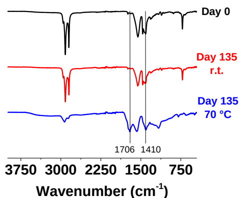
Figure IV-34: FTIR spectra of 14:9Co-2 (1:2 w/w).
