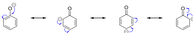
Scheme II-4: Resonance forms of the phenolate anion
