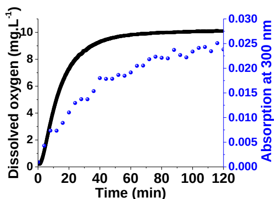
Figure II-47: Dioxygen concentration and absorbance at 300 nm recorded as a function of time for the first oxygenation stage with 1Co ; [1Co] = 4.79 \times 10^{-4} M , solvent: EtOH, l = 1 cm.
