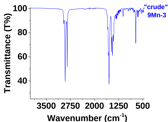
Figure II-25: FTIR spectrum of the 9Mn-3 complex that was not subjected to any purification step.
