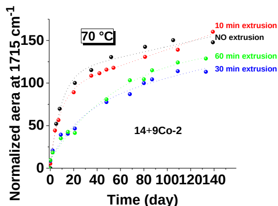
Figure IV-28: Normalized area at 1715 cm -1 illustrating the oxidation of 14 with 9Co-2 at 70 °C after 0, 10, 30 and 60 minutes of “extrusion”.
