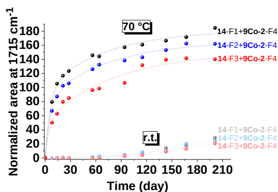
Figure IV-17: Normalized area at 1715 cm -1 illustrating the oxidation process of the three different particle size distributions of 14 with 9Co-2-F4 at r.t. and at 70 °C.
