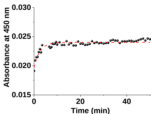
Figure III-12: Absorbance variation at 450 nm of 11 with m -CPBA (5 equiv.) as a function of time; [11] = 7.71 \times 10^{-3} M , solvent: EtOH, l = 1 cm.
