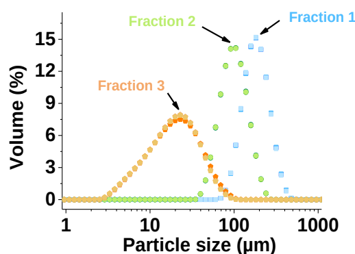
Figure IV-13: Laser diffraction granulometric analysis of 14 after sieving.
