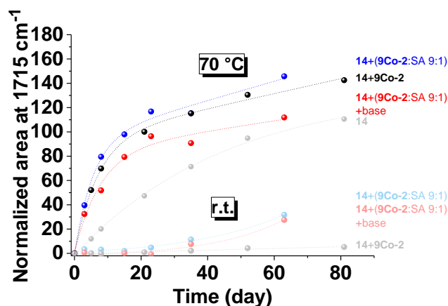
Figure IV-41: Normalized area at 1715 cm -1 illustrating the oxidation of 14 with 9Co-2 at r.t. and at 70 °C in the presence of stearic acid (SA) and calcium oxide (base).
