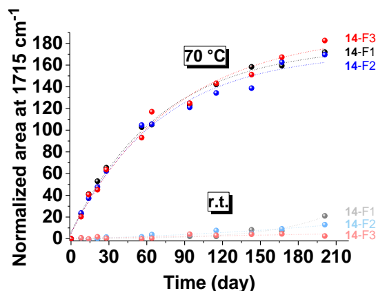
Figure IV-16: Normalized area at 1715 \text{cm}^{-1} illustrating the oxidation reaction of the three-different particle size distributions of 14 alone at r.t. and at 70 °C.
