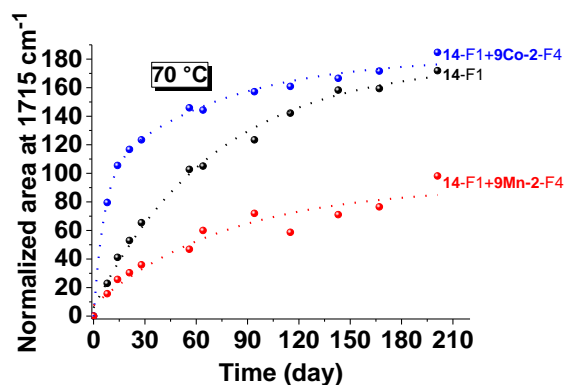
Figure IV-19: Normalized area at 1715\text{ cm}^{-1} describing the oxidation process of 14 alone, with 9Co-2-F4 and with 9Mn-2-F4 as a function of time at 70\text{ }^{\circ}\text{C} .
