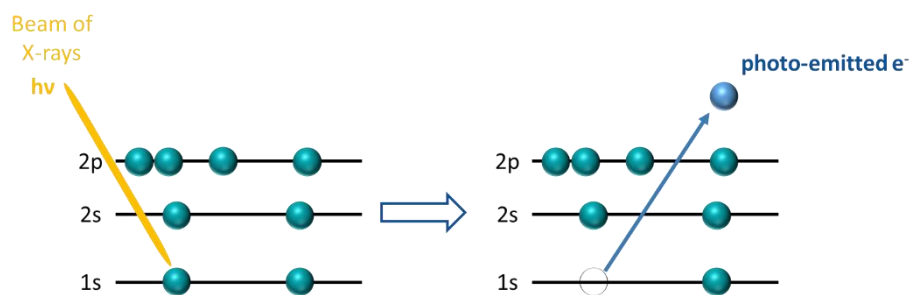
Figure IV-74: XPS principle.
