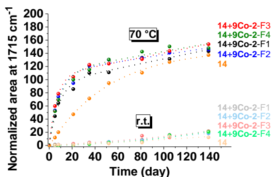
Figure IV-21: Normalized area at 1715\text{ cm}^{-1} illustrating the oxidation process of 14 with the four different particle size distributions of 9Co-2 at r.t. and at 70\text{ }^{\circ}\text{C} .
