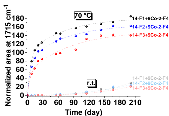
Figure IV-17: Normalized area at 1715\text{ cm}^{-1} illustrating the oxidation process of the three different particle size distributions of 14 with 9Co-2-F4 at r.t. and at 70\text{ }^{\circ}\text{C} .
