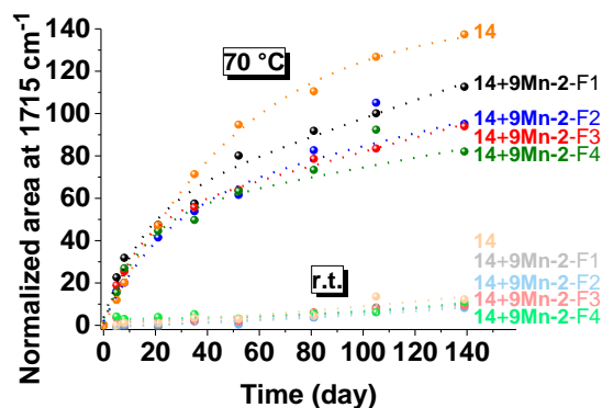
Figure IV-22: Normalized area at 1715\text{ cm}^{-1} describing the oxidation process of 14 with the four different particle size distributions of 9Mn-2 at r.t. and at 70\text{ }^{\circ}\text{C} .
