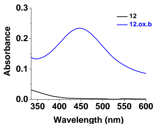
Figure III-9: UV-visible absorption spectra of 12 and 12.ox.b ; [12] = [12.ox.b] = 2.0 \times 10^{-2} \text{ M} , solvent: MeOH, l = 1 \text{ cm} .
