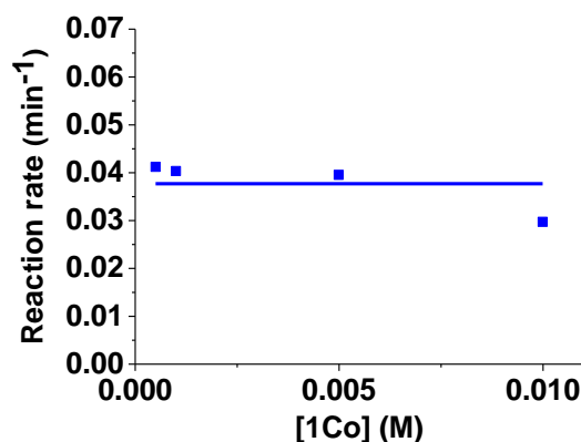
Figure II-38: Variation of the rate constants associated to the oxygenation of 1Co as a function of metal catalyst concentrations; solvent: dioxane:H 2 O (1:1 v/v), l = 1 cm .
