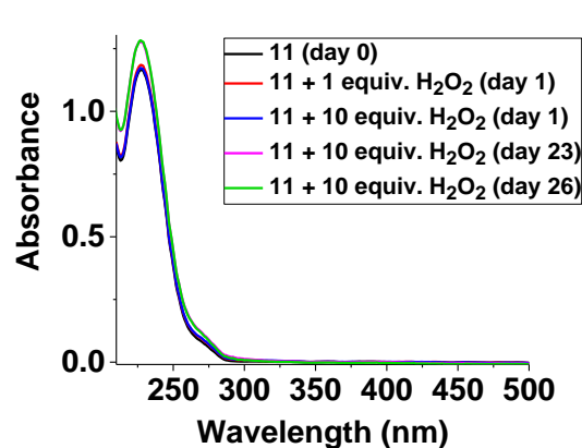
Figure III-3: Oxidation of 11 with \text{H}_2\text{O}_2 (1 and 10 equiv.) monitored by UV-visible absorption spectrophotometry; [11] = 1.05 \times 10^{-4} \text{ M} , solvent: \text{CH}_3\text{CN}:\text{H}_2\text{O} (1:1 v/v), l = 1 \text{ cm} .
