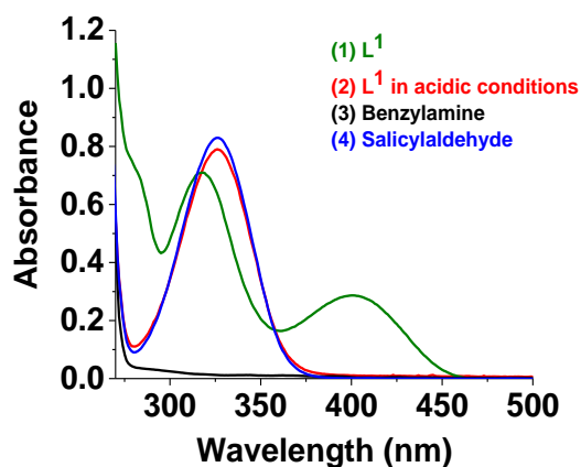
Figure II-11: UV-visible absorption spectra of L^1 in neutral and acidic conditions, benzylamine and salicylaldehyde; (1) [L^1] = 2.26 \times 10^{-4} \text{ M} (pH = 8.6), (2) [L^1] = 2.20 \times 10^{-4} \text{ M} (pH = 3.9), (3) [\text{benzylamine}] = 4.94 \times 10^{-2} \text{ M} , (4) [\text{salicylaldehyde}] = 4.94 \times 10^{-4} \text{ M} , solvent: dioxane: \text{H}_2\text{O} (1:1 v/v), l = 1 \text{ cm} .
