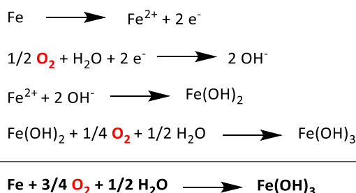
Scheme I-1: Iron-based oxygen scavenger principle.
