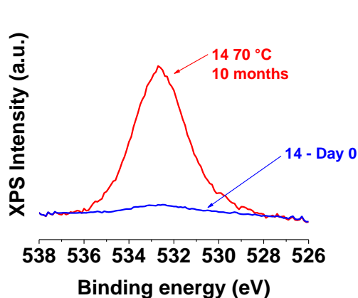
Figure IV-46: XPS O 1s scans of 14 .
