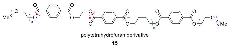
Scheme IV-1: Polymeric additives investigated in this Ph.D. work.
