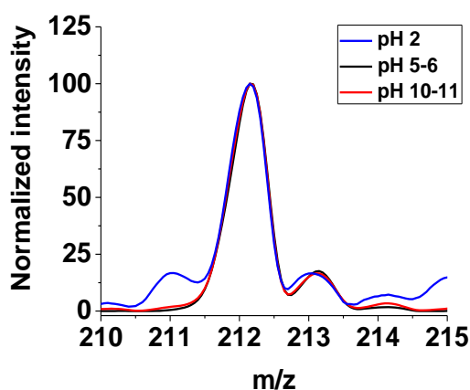
Figure II-12: Stability of a L^1 solution over time (zoom on the [L^1+H]^+ peak centred at m/z = 212.1 ); [L^1] = 9.0 \times 10^{-5} \text{ M} ; solvent: \text{CH}_3\text{CN}:\text{H}_2\text{O} (1:1 v/v); + 100 V.
