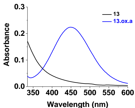
Figure III-10: UV-visible absorption spectra of 13 and 13.ox.a ; [13] = [13.ox.a] = 2.0 \times 10^{-2} \text{ M} , solvent: MeOH, l = 1 \text{ cm} .
