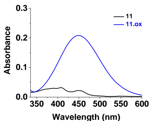
Figure III-8: UV-visible absorption spectra of 11 and 11.ox ; [11] = [11.ox] = 2.0 \times 10^{-2} \text{ M} , solvent: MeOH, l = 1 \text{ cm} .
