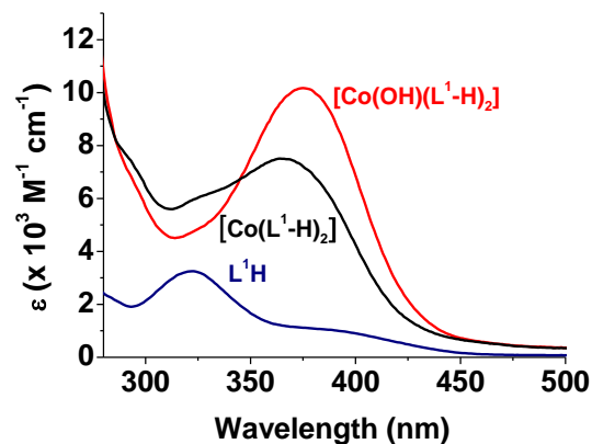
Figure II-29: Electronic spectra of the protonated cobalt(II) L 1 species; solvent: dioxane:H 2 O (1:1 v/v); T = 25.0(2) °C; I = 0.1 M (NaClO 4 .H 2 O).
