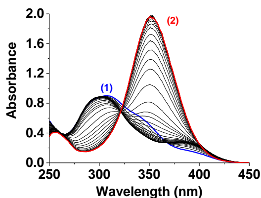
Figure II-16: UV-visible absorption spectrophotometric titration of the free L^2 ligand as a function of pH; (1) pH: 4.00, (2) pH: 12.54, [L^2] = 7.31 \times 10^{-5} M, solvent: dioxane:H 2 O (1:1 v/v), T = 25.0(2) °C, I = 0.1 M (NaClO 4 .H 2 O), l = 1 cm.
