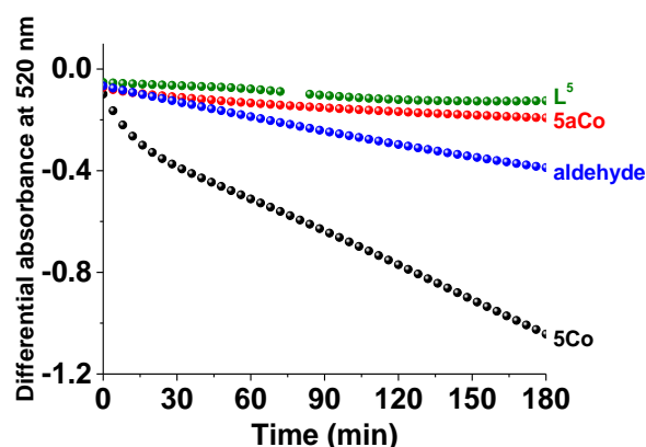
Figure II-70: Oxygenation/activation kinetics of the compound 5\text{Co} series probed by DPPH; [\text{Compounds}] \sim 3 \times 10^{-4}\text{M} , [\text{Compounds}]/[\text{DPPH}] = 1.0 , solvent: dioxane, l = 1\text{cm} , T = 25.0(2)^\circ\text{C} .
