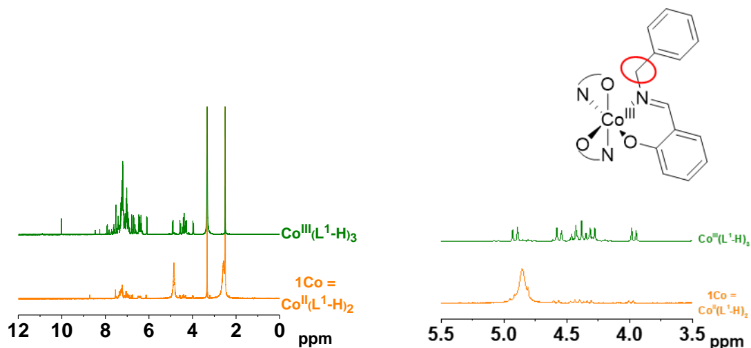
Figure II-60: ^1\text{H} NMR spectra of the cobalt(II) bischelate 1Co and its corresponding cobalt(III) trischelate analogue; solvent: (\text{CD}_3)_2\text{SO} .
