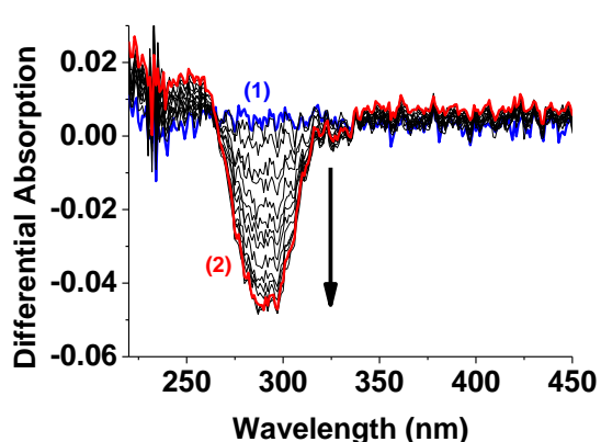
Figure II-39: Differential absorption spectra measured at regular intervals during the first oxygenation stage of 8Co ; (1) t = 0 , (2) t = 2 h, [\mathbf{8Co}] = 2 \times 10^{-4} M, solvent: dioxane:H 2 O (1:1 v/v), l = 1 cm.
