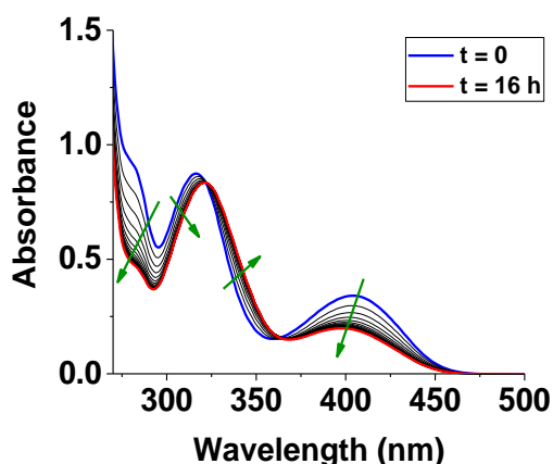
Figure II-5: Stability of a L^1 solution monitored by UV-visible absorption over 16 hours; [L^1] = 2.50 \times 10^{-4} M , solvent: dioxane: H_2O (1:1 v/v), l = 1 cm.
