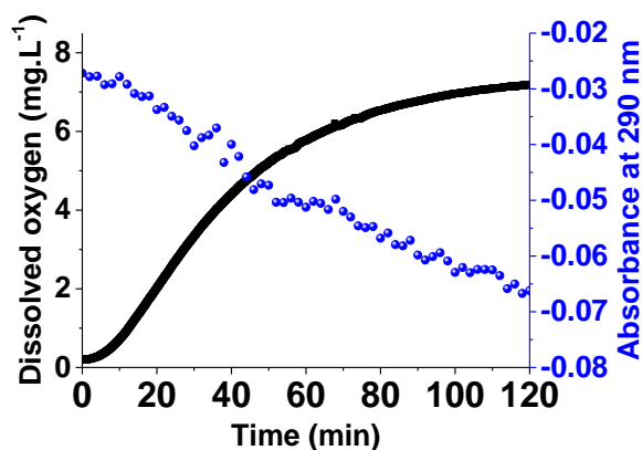
Figure II-42: Dissolved oxygen concentration and absorbance variation at 290 nm as a function of time for the second oxygenation stage of 8Co ; [\mathbf{8Co}] = 2 \times 10^{-4} M, solvent: dioxane:H 2 O (1:1 v/v), l = 1 cm.
