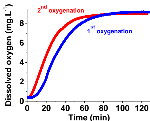
Figure II-46: Superimposition of the two oxygenation curves of 1Co during the oxygenation stages; [1Co] = 6 \times 10^{-4} M , solvent: dioxane:H 2 O (1:1 v/v).
