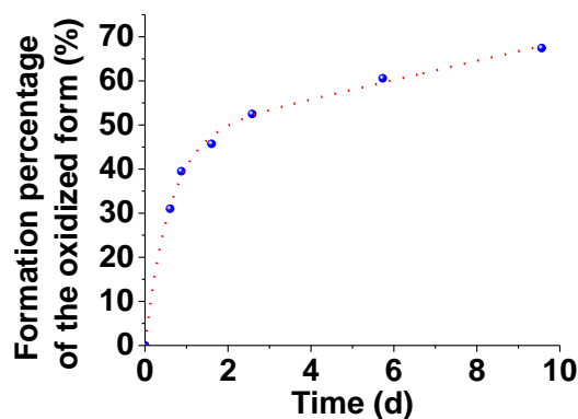
Figure II-56: Formation percentage of the oxidized form of 1Co over 10 days.
