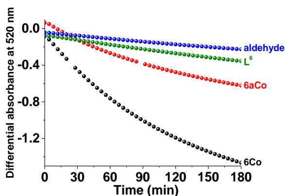
Figure II-71: Oxygenation/activation kinetics of the compound 6\text{Co} series probed by DPPH; [\text{Compounds}] \sim 3 \times 10^{-4}\text{M} , [\text{Compounds}]/[\text{DPPH}] = 1.0 , solvent: dioxane, l = 1\text{cm} , T = 25.0(2)^\circ\text{C} .
