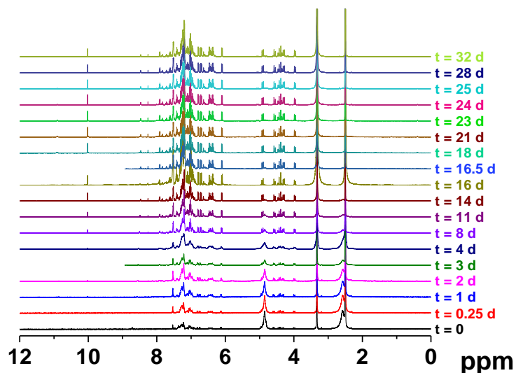
Figure II-62: ^1\text{H} NMR spectra of 1Co recorded over time; solvent: (\text{CD}_3)_2\text{SO} .
