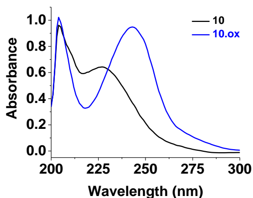
Figure III-7: UV-visible absorption spectra of 10 and 10.ox ; [10] = [10.ox] = 2.0 \times 10^{-5} \text{ M} , solvent: MeOH, l = 1 \text{ cm} .
