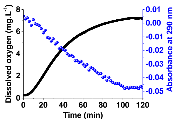
Figure II-40: Dissolved oxygen concentration and absorbance variation at 290 nm as a function of time for the first oxygenation stage of 8Co ; [\mathbf{8Co}] = 2 \times 10^{-4} M, solvent: dioxane:H 2 O (1:1 v/v), l = 1 cm.
