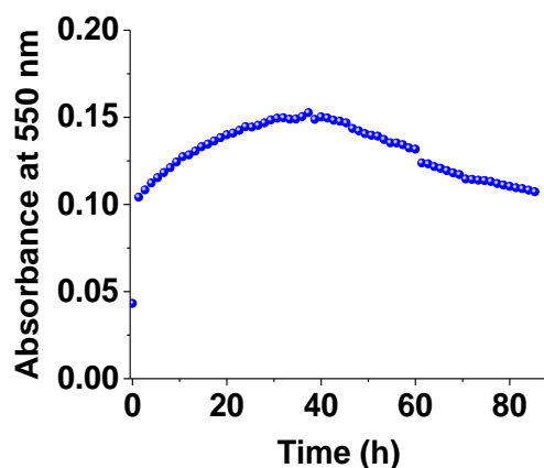
Figure II-36: Variation of the absorbance at 550 nm of 1Co as a function of time; [1Co] = 2.51 \times 10^{-3} M , solvent: dioxane:H 2 O (1:1 v/v), l = 1 cm .
