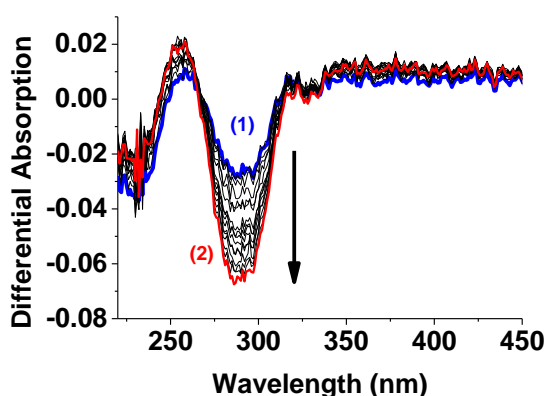
Figure II-41: Differential absorption spectra recorded during the second oxygenation stage of 8Co ; (1) t = 0 , (2) t = 2 h, [\mathbf{8Co}] = 2 \times 10^{-4} M, solvent: dioxane:H 2 O (1:1 v/v), l = 1 cm.
