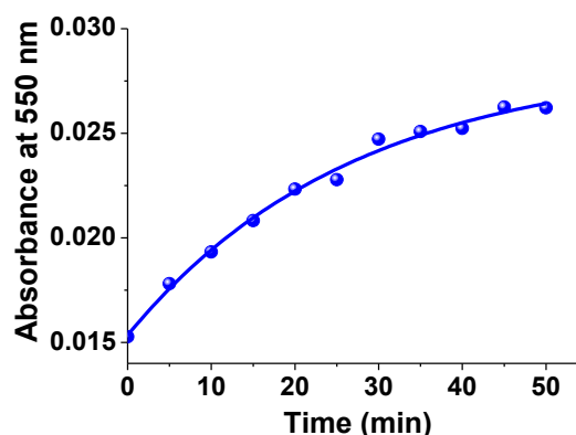
Figure II-37: Variation of the absorbance at 550 nm of 1Co as a function of time; [1Co] = 5 \times 10^{-4} M , solvent: dioxane:H 2 O (1:1 v/v), l = 1 cm .
