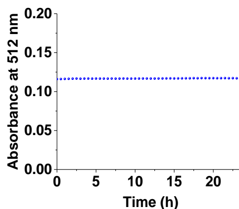
Figure II-33: Absorbance at 512 nm as a function of time; [\text{Co}(\text{ClO}_4)_2 \cdot 6\text{H}_2\text{O}] = 2.51 \times 10^{-3} M, solvent: dioxane: \text{H}_2\text{O} (1:1 v/v); l = 1 cm.
