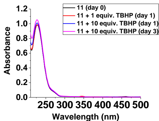
Figure III-2: Oxidation of 11 with TBHP (1 and 10 equiv.) monitored by UV-visible absorption spectrophotometry; [11] = 1.05 \times 10^{-4} \text{ M} , solvent: \text{CH}_3\text{CN}:\text{H}_2\text{O} (1:1 v/v), l = 1 \text{ cm} .
