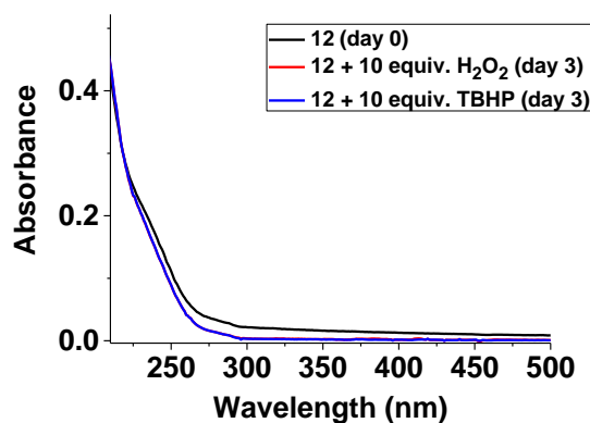
Figure III-4: Oxidation of 12 with \text{H}_2\text{O}_2 (10 equiv.) and TBHP (10 equiv.) followed by UV-visible absorption spectrophotometry; [12] = 1.06 \times 10^{-5} \text{ M} , solvent: \text{EtOH} , l = 1 \text{ cm} .
