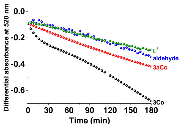
Figure II-69: Oxygenation/activation kinetics of the compound 3\text{Co} series probed by DPPH; [\text{Compounds}] \sim 3 \times 10^{-4}\text{M} , [\text{Compounds}]/[\text{DPPH}] = 1.0 , solvent: dioxane, l = 1\text{cm} , T = 25.0(2)^\circ\text{C} .
