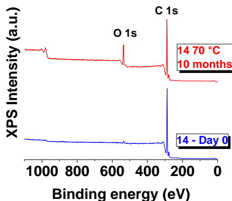
Figure IV-43: XPS survey scans of 14 .
