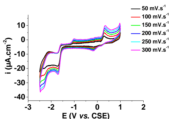
Figure II-74: CV voltammograms of complex 1Co measured at different scan rates; [\mathbf{1Co}] = 9.74 \times 10^{-4} \text{ M} , solvent: DMSO, I = 0.1 \text{ M} ( n\text{-NBu}_4\text{PF}_6 ).
