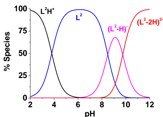
Figure II-19: Distribution diagrams of the protonated L^2 species; [L^2] = 7.31 \times 10^{-5} M, solvent: dioxane:H 2 O (1:1 v/v), T = 25.0(2) °C, I = 0.1 M (NaClO 4 .H 2 O), l = 1 cm.
