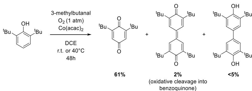
Scheme III-3: Oxidation of 2,6-di- tert -butylphenol catalysed by cobalt(II)(acac) 2 and described by the group of Mastrorilli.
