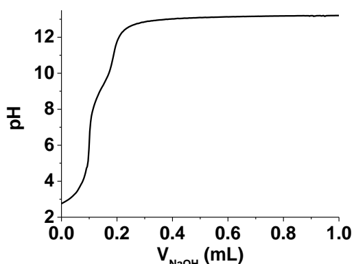
Figure II-18: Potentiometric titration curve of L^2 ; [L^2] = 1.05 \times 10^{-3} M, solvent: dioxane:H 2 O (1:1 v/v), T = 25.0(2) °C, I = 0.1 M (NaClO 4 .H 2 O).
