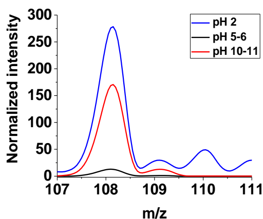
Figure II-13: ESI-MS spectra of L^1 at different pH conditions (zoom on the [\text{benzylamine}+H]^+ peak centred at m/z = 108.1 ); [L^1] = 9.0 \times 10^{-5} \text{ M} , solvent: \text{CH}_3\text{CN}:\text{H}_2\text{O} (1:1 v/v), + 100 V.
