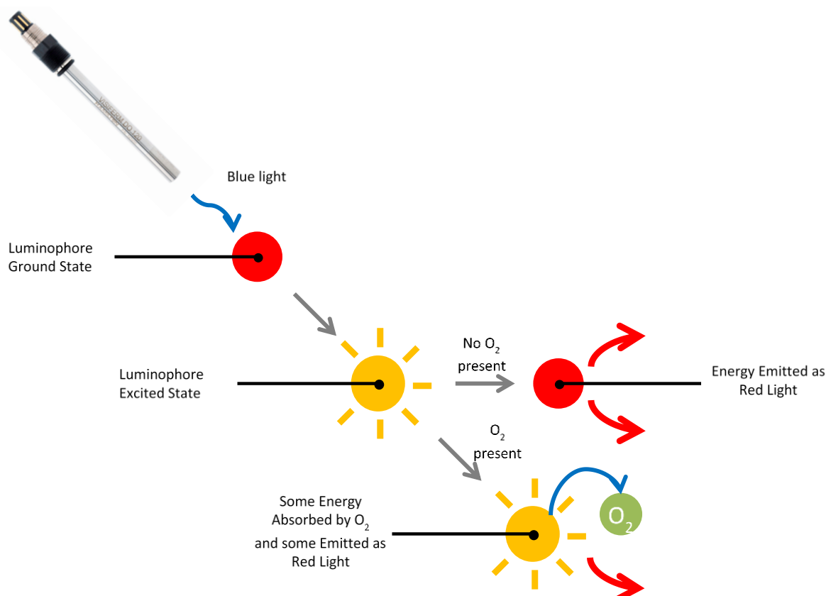
Figure II-78: Principle of the Visiferm™ DO Arc 120 (Hamilton).
