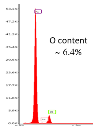
Figure IV-9: SEM-EDS analysis of 14 after oxidation at 70 °C.
