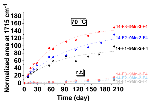
Figure IV-18: Normalized area at 1715\text{ cm}^{-1} illustrating the oxidation process of the three different particle size distributions of 14 with 9Mn-2-F4 at r.t. and at 70\text{ }^{\circ}\text{C} .
