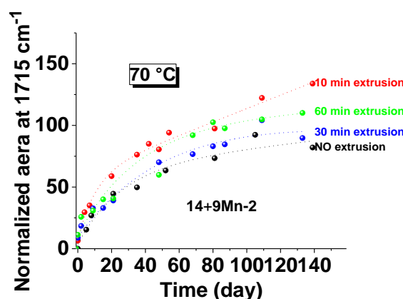
Figure IV-29: Normalized area at 1715\text{ cm}^{-1} representing the oxidation of 14 with 9Mn-2 at 70\text{ °C} after 0, 10, 30 and 60 minutes of “extrusion”.
