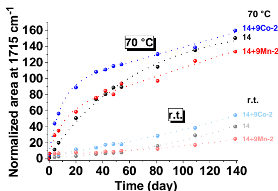
Figure IV-24: Normalized area at 1715 \text{cm}^{-1} representing the oxidation of 14 , with 9Co-2 and 9Mn-2 at r.t. and at 70 °C after 10 minutes of “extrusion”.
