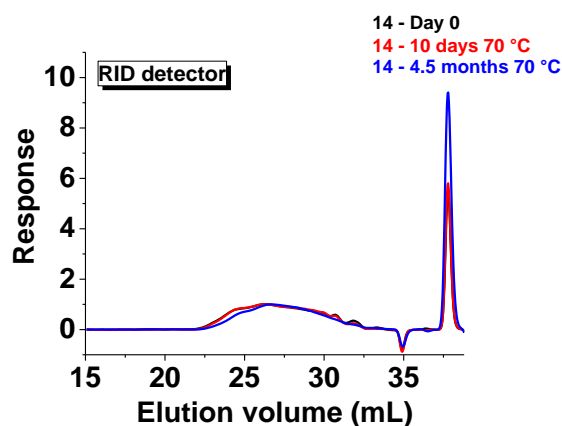
Figure IV-49: SEC measurements of non-oxidized 14 before (black) and after 10 days (red) and 4.5 months (blue) of oxidation at 70 °C - refractive index detector (RID).
