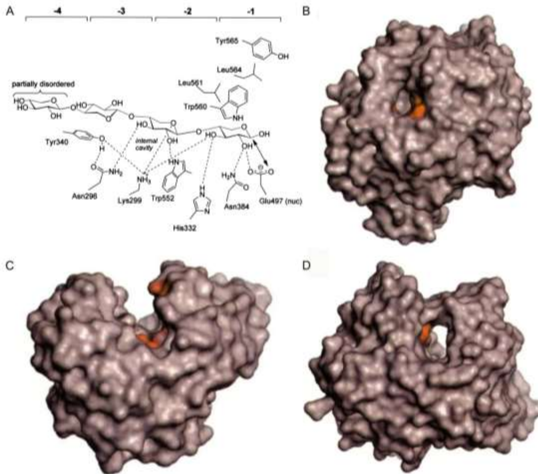
Fig B-2. Sugar binding subsite topologies in glycosyl hydrolases.
