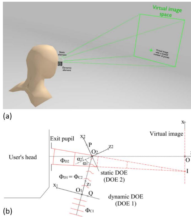
Fig. 2.21. (a) An illustration of the setup and (b) Top view of the optical system (not to scale). Q is a point of the plane of DOE 1, P is point of the plane of DOE 2 and I is a point of the plane of the virtual image. \alpha_1 is the angle between the normal to DOE 2 and the direction (O_1O_2) . \alpha_2 is the angle between the normal to DOE 2 and the direction (OO_2) [51].
