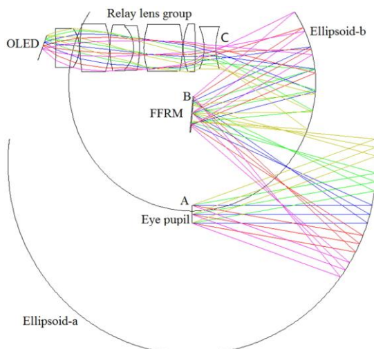
Fig. 2.15. Structure of the HMD with freeform reflective mirror (FFRM) based on the two similar ellipsoids. It consists of two ellipsoid surfaces, an FFRM, a 7-pieces co-axis relay lens group, and an OLED [44].
