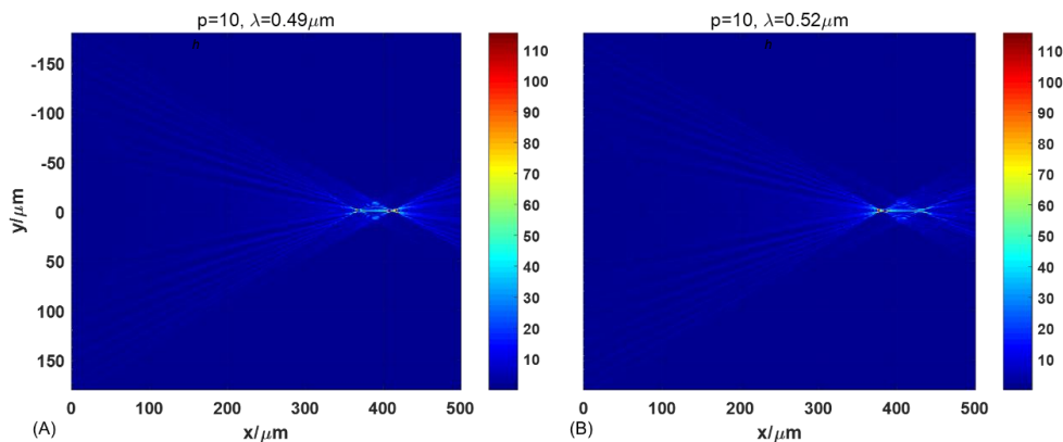
Fig. 6.6. Electric field intensity distribution of a harmonic lens with p_h=10 . (a) \lambda=0.49 \mu\text{m} and (b) \lambda=0.52 \mu\text{m} .
