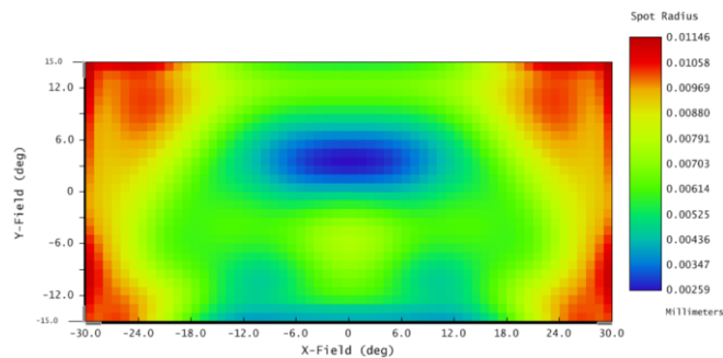
Fig. 3.18. RMS spot radius field map.
