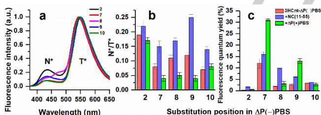
Figure 2. Spectroscopic properties of the \Delta P(-) PBS sequences labeled by 3HCnt at different positions. (a) Fluorescence spectra were recorded for 2 \mu\text{M} \Delta P(-) PBS labeled by 3HCnt at position 2 (black line), 7 (red), 8 (magenta), 9 (blue) and 10 (green). All spectra were normalized at the T^* band. (b) N^*/T^* ratio and (c) fluorescence quantum yield of the 3HCnt-labeled \Delta P(-) PBS sequences. The 3HCnt-labeled sequences at 2 \mu\text{M} were either in the form of stem-loops in the absence (red bars) or the presence of 8 \mu\text{M} NC(11–55) (blue bars) or in the form of duplexes with the complementary \Delta P(+) PBS sequence (green bars). Buffer: 10 mM phosphate buffer, 30 mM NaCl, pH = 6.5. Excitation was at 360 nm.
