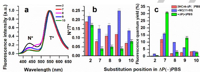
Figure 2. Spectroscopic properties of the \Delta P(-) PBS sequences labeled by 3HCnt at different positions. (a) Fluorescence spectra were recorded for 2\ \mu\text{M} \Delta P(-) PBS labeled by 3HCnt at position 2 (black line), 7 (red), 8 (magenta), 9 (blue) and 10 (green). All spectra were normalized at the T^* band. (b) N^*/T^* ratio and (c) fluorescence quantum yield of the 3HCnt-labeled \Delta P(-) PBS sequences. The 3HCnt-labeled sequences at 2\ \mu\text{M} were either in the form of stem-loops in the absence (red bars) or the presence of 8\ \mu\text{M} NC(11–55) (blue bars) or in the form of duplexes with the complementary \Delta P(+) PBS sequence (green bars). Buffer: 10 mM phosphate buffer, 30 mM NaCl, pH = 6.5. Excitation was at 360 nm.
