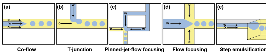
Figure 2. Main geometries used for droplet generation. (a) Droplet generation by co-flowing an aqueous phase (in blue) arriving from a capillary immersed in an oil stream (yellow). (b–d) Droplet generators with planar geometries. Channels in which oil (shaded in yellow) and aqueous phase (shaded in blue) flow are respectively labeled “o” and “w”. Arrows indicate flow directions. (e) Schematic of a step emulsification process.
