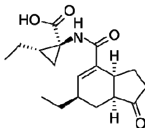
Figure 1.42 : Coronatine
