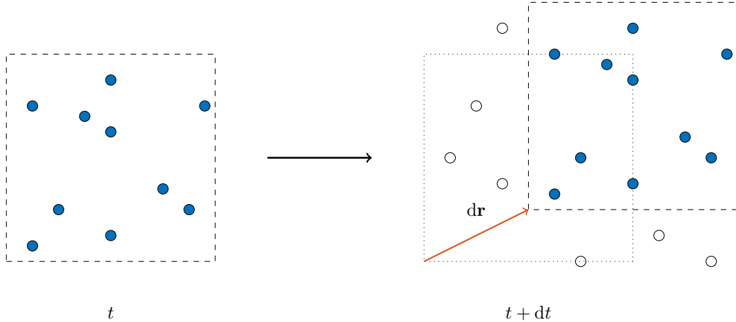
Figure 2.8: Schematic illustration of the PIV technique, with a displaced field of seeding particles \mathbf{dr} (in blue) during dt in a box contained in the observation plane. Adapted from [104].
