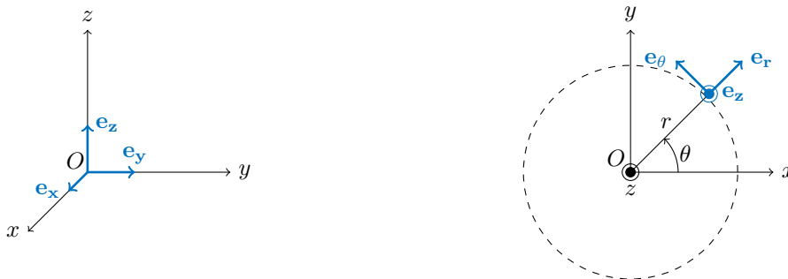
Figure A.1: Left: Cartesian coordinates (x, y, z) . Right: Cylindrical (polar) coordinates (r, \theta, z) .
