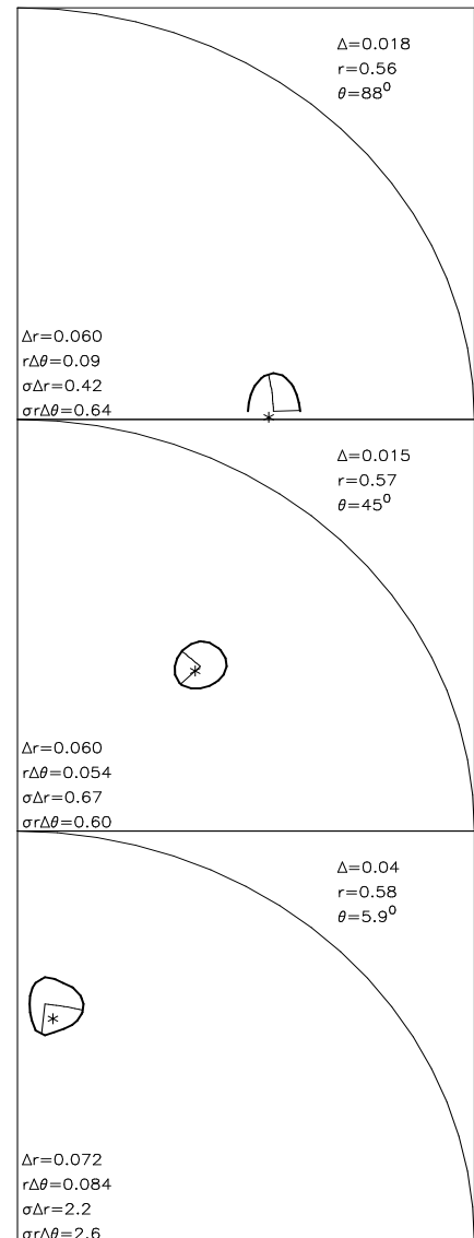
Figure 4: Contour plot curve C of the averaging kernels for the target radius r_0=0.55 (indicated by a * point) and three latitudes (equator, mid-latitude and pole) corresponding to half height of the maximum value.
