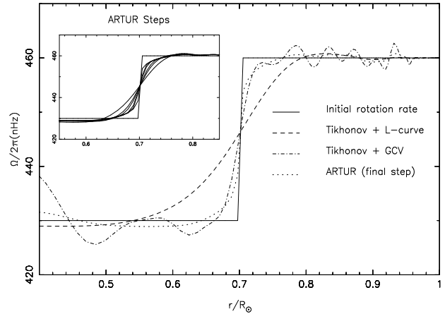
Fig. 1. Solutions obtained by inverting splittings computed from a discontinuous one dimension rotation profile (full line) for the same model as in LOWL data and by adding some 'realistic' noise (see text). The standard Tikhonov solution is given for two different automatic choices of the regularizing parameter. The successive steps of ARTUR algorithm are given in the upper left window whereas the final step is shown on the main plot. The choice of the regularizing function and parameters for ARTUR algorithm are those discussed in Sect. 5. The solutions are plotted without error bars for clarity.
