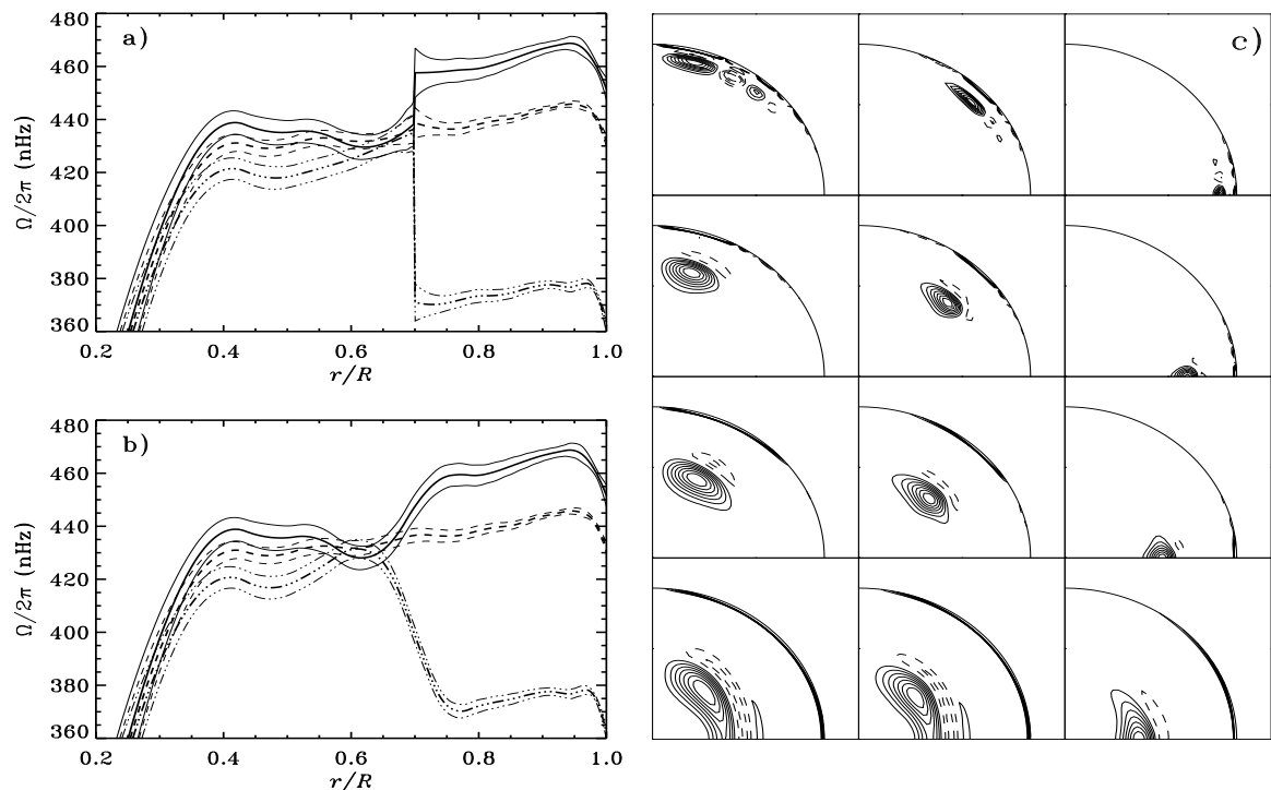
Figure 5. (a) Solution at latitudes 0^\circ (solid), 30^\circ (dashed) and 60^\circ (triple-dot dashed) for a 2D RLS of GONG data, allowing the solution to adopt a discontinuity at the base of the convection zone. Adjacent curves indicate \pm 1\sigma error limits. (b) As (a) but not allowing a discontinuity ('standard' 2D RLS). (c) Averaging kernels corresponding to the solution in panel b, at target latitudes (left to right) 90^\circ , 45^\circ and 0^\circ and radii (top to bottom) 0.9R , 0.7R , 0.55R , 0.4R . (Nice group)
