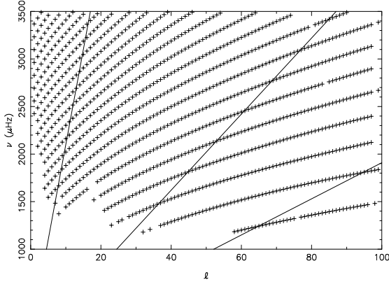
Fig. 1. l - \nu diagram showing the modes included in the LOWL 2 year dataset. Solid lines indicate the values of \nu/L that correspond to modes with turning points r_t=0.4, 0.85, 0.95R_\odot from the left to the right.
