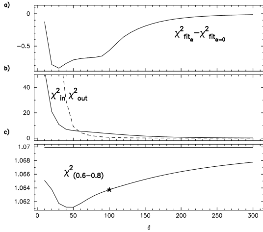
Fig. 7a-c. Variation of various \chi^2 indicators with \delta . a Difference between the goodness of the fits of ARTUR solutions by an erf function with or without a linear part (cf. Eq. (22)). b Difference between T-GCV and ARTUR solutions in and out of the zones where high gradients are expected (cf. Eq. (21)). c The normalized \chi^2 value of ARTUR inversions for modes which have their turning points between 0.6R_\odot and 0.8R_\odot . The horizontal line shows the value (1.07) obtained from T-GCV solution. The star symbol indicate the \chi^2 value reached for the choice \delta = 100 retained for ARTUR algorithm.
