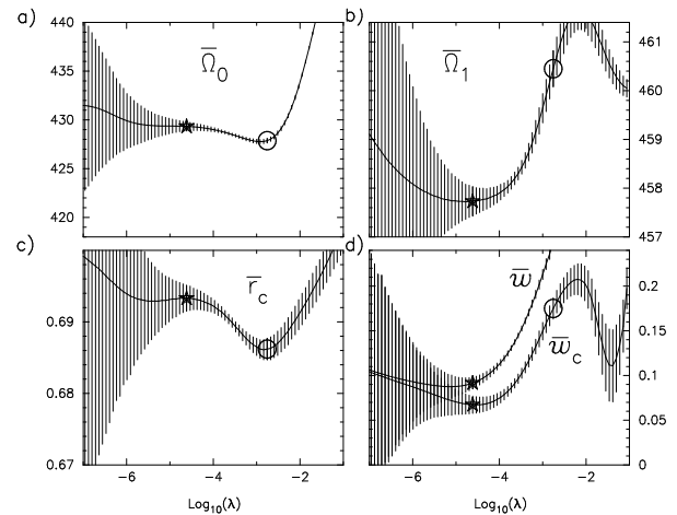
Fig. 10a-d. Variation of the inferred parameters \bar{\Omega}_0 , \bar{\Omega}_1 , \bar{r}_c , \bar{w} and \bar{w}_c as a function of the logarithm of the regularization parameter for the Tikhonov inversion of LOWL data. Graph markers have the same meaning as in Fig. 1. The L-curve choice of \bar{w} is outside the plot on panel d .
