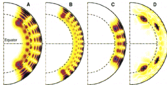
Fig. 1. (A–C) Meridional cuts through three rotation kernels for modes with frequencies \nu \approx 1500 \mu\text{Hz} , for (A) \ell = 15, m = 8 ; (B) \ell = 28, m = 14 ; and (C) \ell = 28, m = 24 . The color scale indicates the absolute magnitude of the kernel; dark colors (black and blue) represent the largest values, and light colors (yellow and white) represent values close to zero. The latitudinal extent of the kernels varies with m/L , and the radial extent varies with w/L . Except close to the deepest point where it has appreciable amplitude, each kernel is nearly a product of a function of radius and a function of latitude. (D) Meridional cut through averaging kernels for a RLS inversion (as in Fig. 3B), for target radii and latitudes r = 0.70R, 60^\circ and r = 0.82R, 30^\circ . The averaging kernels are symmetric about the equatorial plane, so that they are also peaked at latitudes -60^\circ and -30^\circ . The four crosses indicate target locations.
