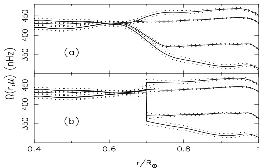
Figure 2: Rotation rate versus solar radius for latitudes 0, 30, 60, 90^{\circ} obtained with dataset I. (a) Without discontinuous basis (b) With a basis discontinuous at 0.7R_{\odot}
