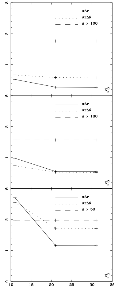
Figure 5: Sensitivity of the radial and latitudinal resolution multiplied by the error on the solution \sigma\Delta r and \sigma r\Delta\theta relatively to the number of piecewise polynomials N_r^\Omega . They are given for three values N_r^\Omega = 10, 20, 30 at the same location ( r_0 = 0.55 ) and ( \mu_0 = 0.01, 0.707, 0.99 ) than Figure 4. The position of the maximum value of the averaging kernel, characterized by \Delta , is not modified within the grid of r and \mu we use to compute these kernels.
