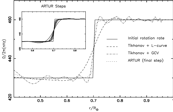
Figure 2. The same as Figure 1 but computed for a lower level of noise (standard deviations divided by \sqrt{10} ). Comparison between Figures 1 and 2 shows the smoothing effect of the data noise level for the three methods.
