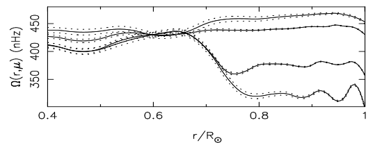
Figure 1: Rotation rate versus solar radius for latitudes 0, 30, 60, 90^\circ obtained with dataset I
