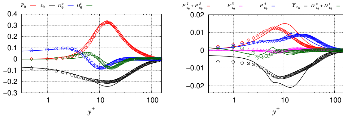
FIGURE 24. Temperature variance \overline{\theta'^2} budgets (left) and the dissipation rate \varepsilon_\theta budgets (right) for Conjugate Heat Transfer (CHT) . The symbols stand for DNS data and the solid lines represent the present model.
