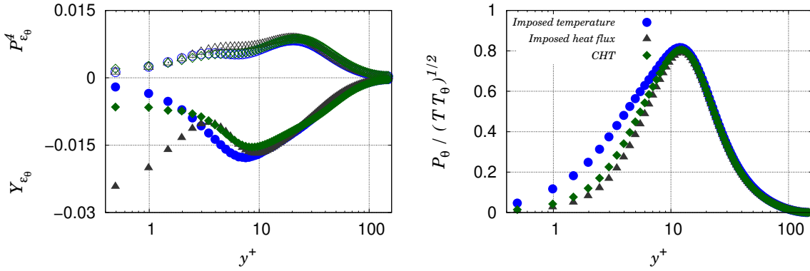
FIGURE 14. The turbulent production P_{\varepsilon_\theta}^4 and the dissipation rate Y_{\varepsilon_\theta} (left) and the thermal production P_\theta divided by the mixed time-scale \sqrt{\mathcal{T}\mathcal{T}_\theta} from the DNS Data of Flageul et al. (2015, 2017) for different kinds of temperature boundary conditions.
