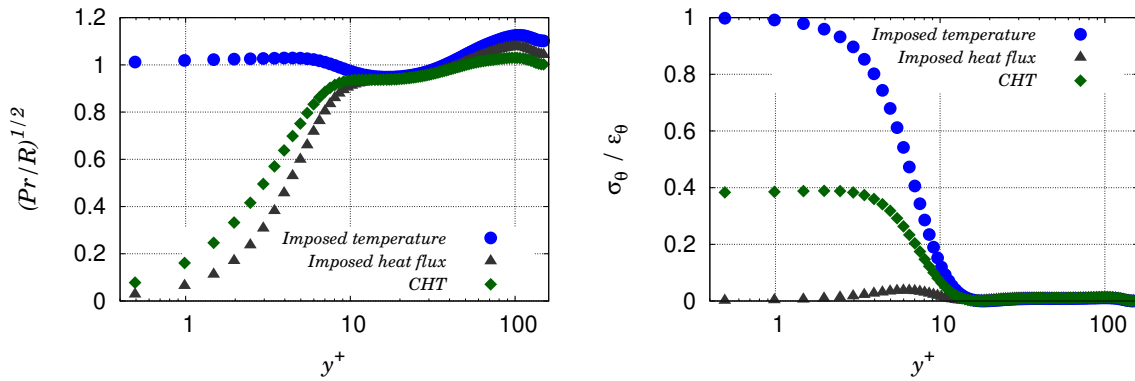
FIGURE 17. The two parameters \sqrt{Pr/R} (left) and \sigma_\theta/\varepsilon_\theta used to distinguish between the different kinds of temperature boundary condition, from DNS Data of Flageul et al. (2015, 2017).
