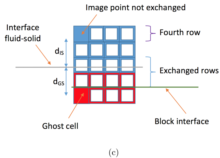
Figure 3.8: Example of cases where the image point is not exchanged between processors. Blue: fluid cells; red: solid cells.
