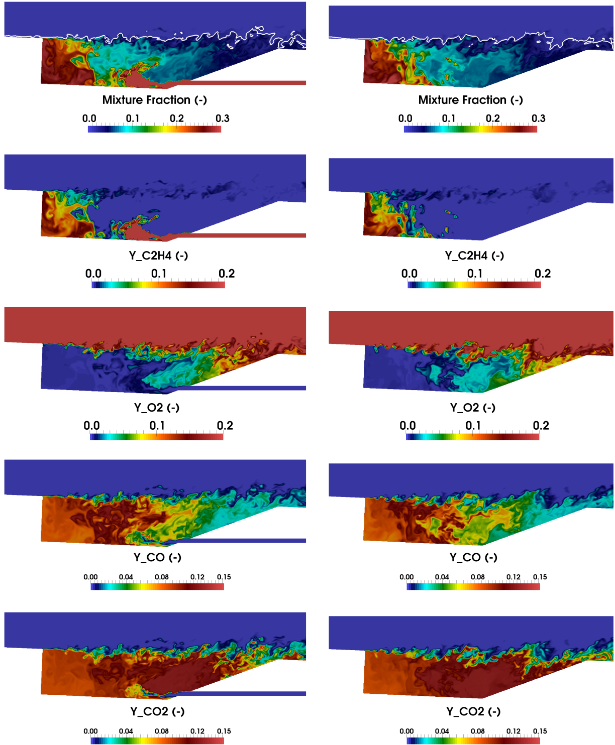
Figure 5.19: Instantaneous fields of mixture fraction and mass fractions of C_2H_4 , O_2 , CO and CO_2 at the injector centerplane (left) and the centerplane between two injectors (right). The isoline Mach = 1 is displayed with a white line. Fine mesh.
