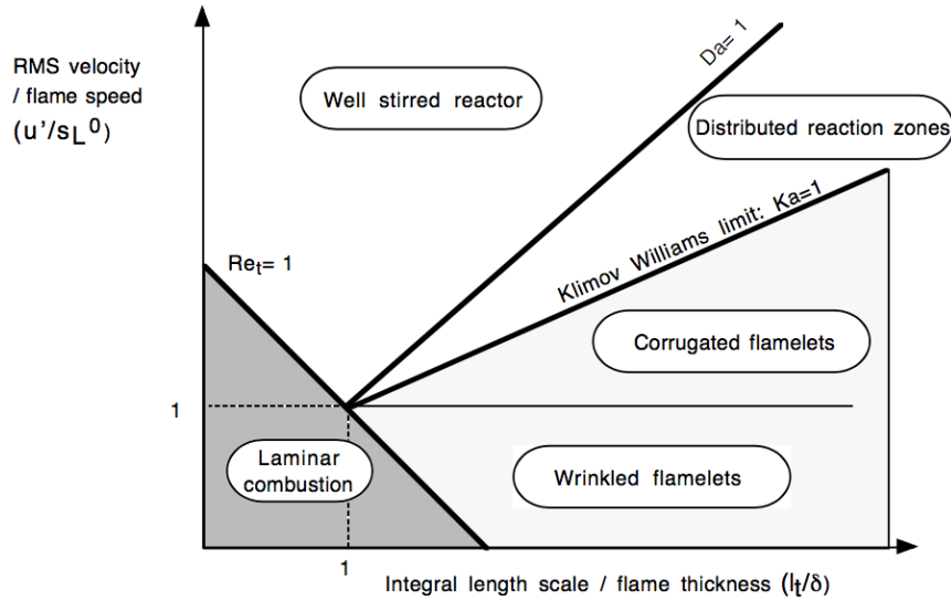
Figure 2.4: Turbulent combustion diagram by Peters [127]
