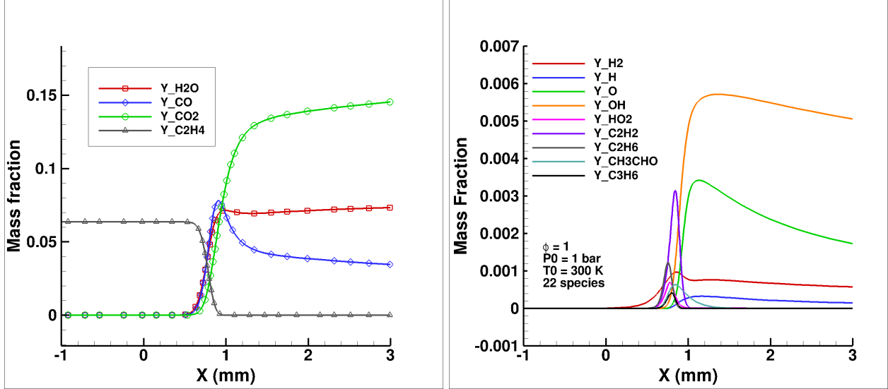
Figure 5.11: Ethylene-air combustion products at P = 1 bar, T = 300 K and \phi = 1 for S22.
