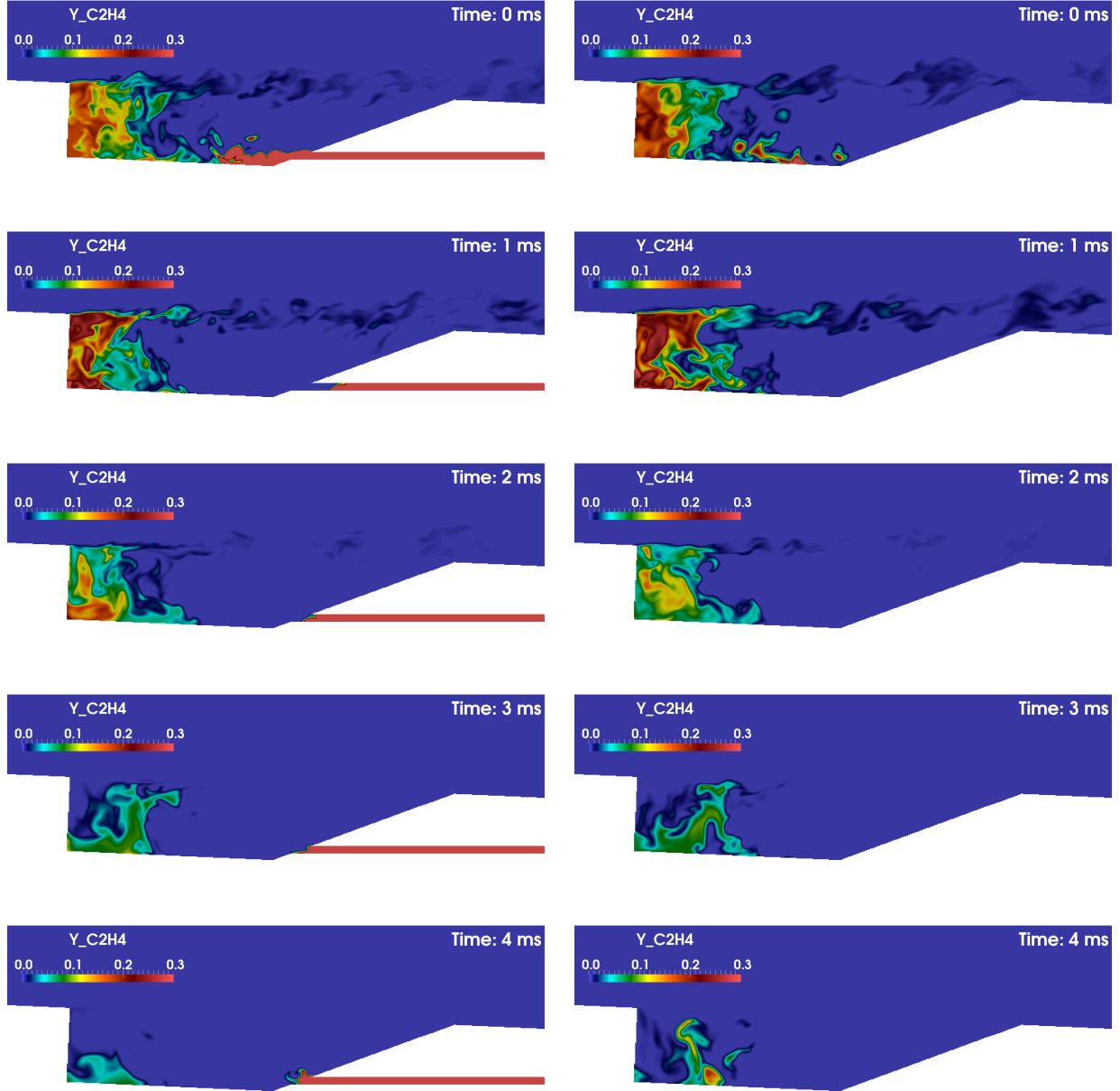
Figure 5.34: Snapshots of ethylene mass fraction at injector centerplane (left) and centerplane between two injectors (right) for a lean fuel loading (RCA1L), presented every ms from t = 0 to 4 ms. Coarse mesh.
