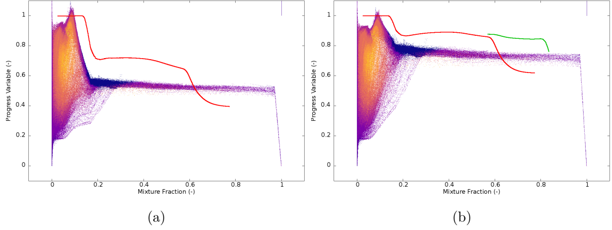
Figure 6.34: Scatter plot of progress variables C_1 (a) and C_2 (b) vs. mixture fraction: blue color refers to negative heat release rate, the shading from purple to yellow represents cells with low to high heat release rate. The curves show the maximum value of tabulated progress variable for a given composition C_{max}(Z) with a 1D computational domain of 10 m for red color and 1 km for green color.
