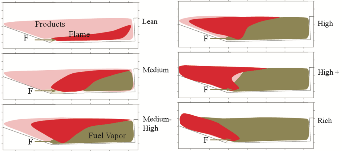
Figure 4.6: Fuel flow regimes [164].
