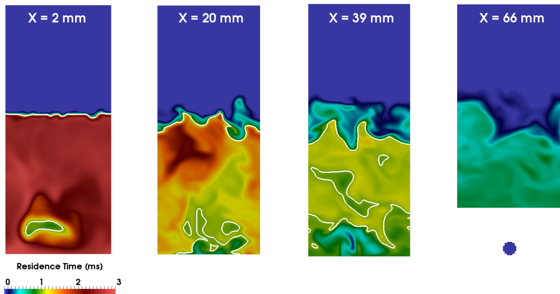
Figure 6.17: Residence time inside the cavity in planes with constant x for RCA1. The isoline \tau_r = 1 \text{ ms} is displayed with a white line.
