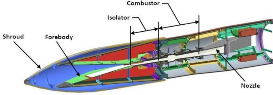
Figure 1.11: Schematic of HIFiRE Flight 2 [17].
