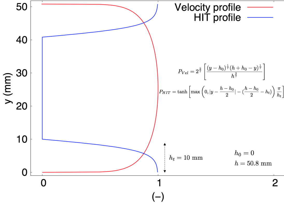
Figure 4.23: Velocity and HIT profiles.
