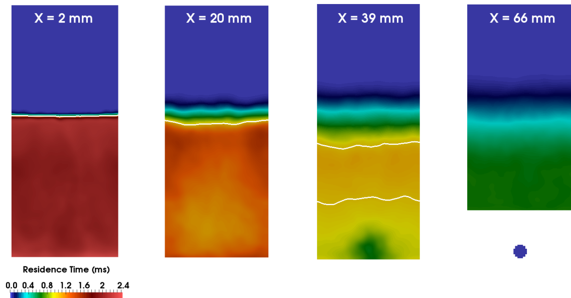
Figure 6.19: Averaged residence time inside the cavity in planes with constant x for RCA1. The isoline \tau_r = 1 \text{ ms} is displayed with a white line.
