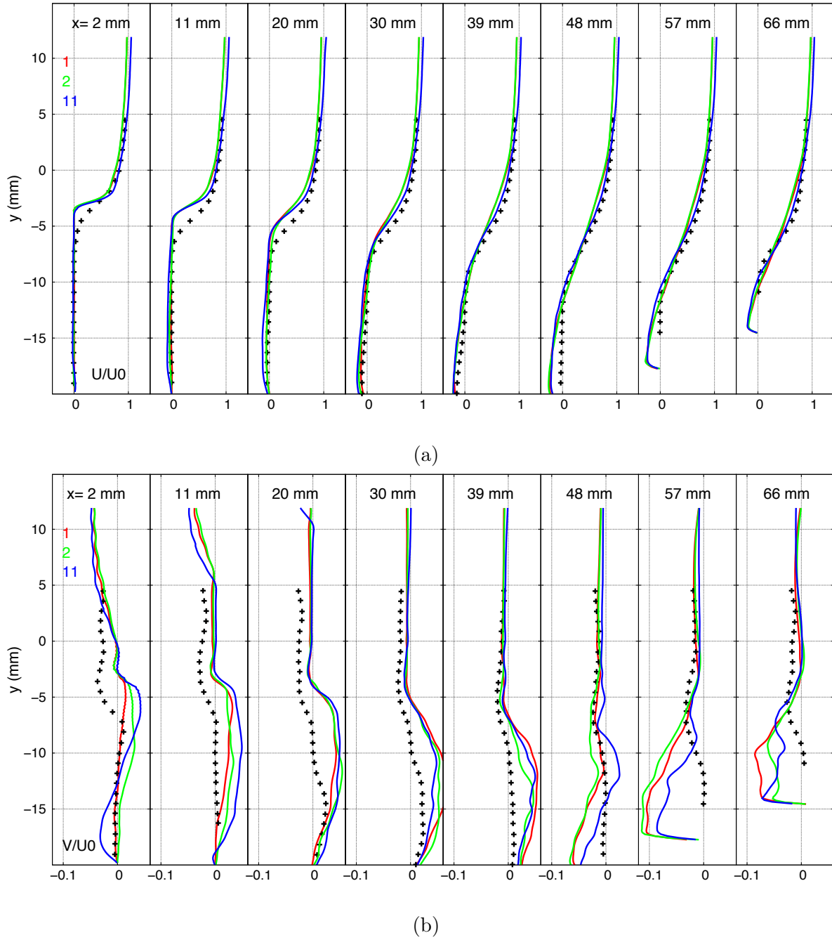
Figure 5.48: Averaged streamwise (a) and transverse (b) velocity profiles inside the cavity, comparison between the numerical and the experimental data for coarse mesh at the centerplane between two injectors: experiment (pattern), numerical data of one (red line), two (green line) and eleven (blue line) injectors (between 6-th and 7-th).
