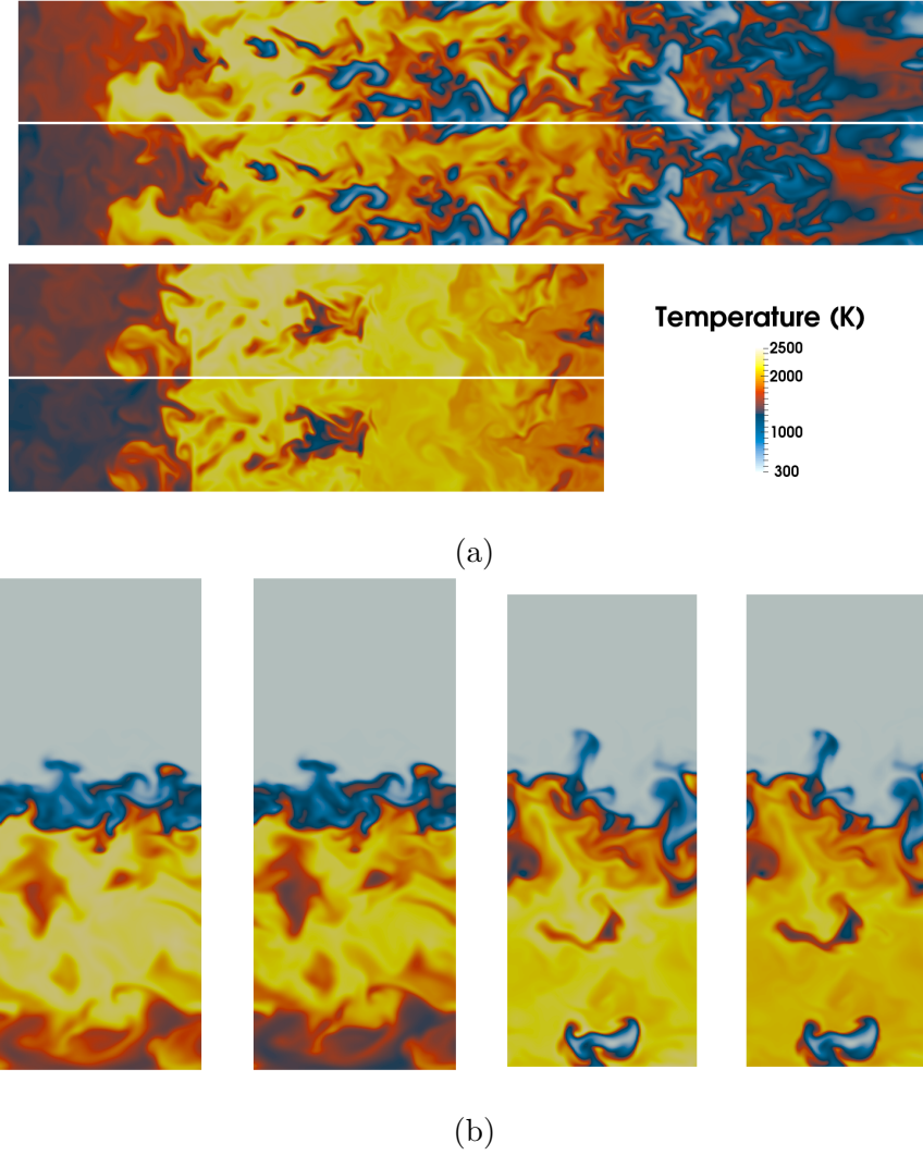
Figure 6.39: Temperature comparison with (a) constant y cuts at mixing layer ( y = -7 mm) and middle line of the cavity ( y = -14 mm): from top to bottom, LES, TAB2 at y = -7 mm, then LES, TAB2 at y = -14 mm; and (b) constant x cuts at the interface of the recirculation zones ( x = 20 mm from the cavity front) and the middle of the large recirculation area ( x = 39 mm): from left to right LES, TAB2 at x = 20 mm, then LES, TAB2 at x = 39 mm.
