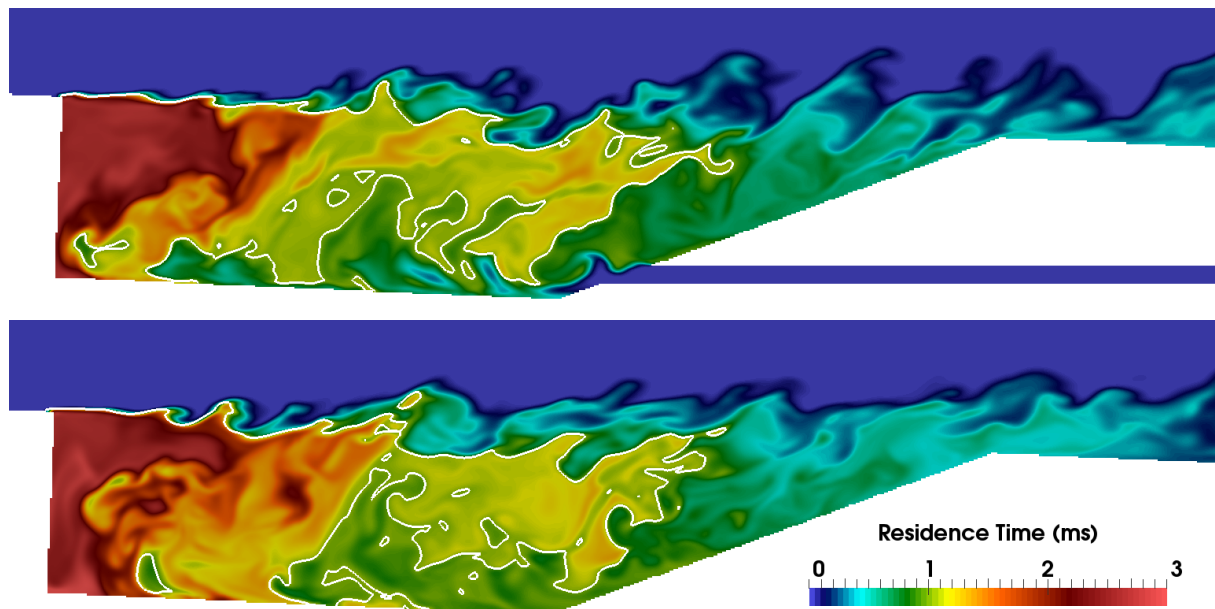
Figure 6.16: Residence time inside the cavity in the injector centerplane (top) and the centerplane between two injectors (bottom) for RCA1. The isoline \tau_r = 1 ms is displayed with a white line.
