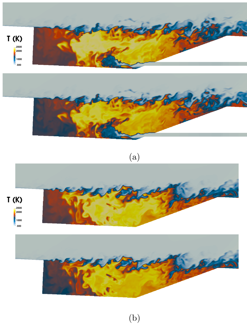
Figure 6.38: Temperature comparison with LES results at injector centerplane (a) and centerplane between two injectors (b): LES (top), TAB2 (bottom)
