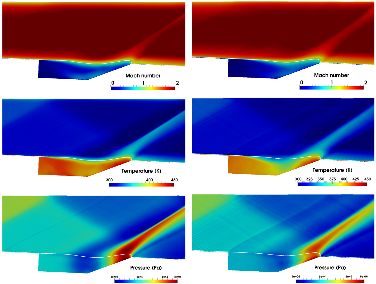
Figure 4.16: Various averaged properties of the flow for fine (left) and coarse (right) meshes: Mach number (top), temperature (middle) and pressure (bottom). The isoline Mach = 1 is displayed with a white line.
