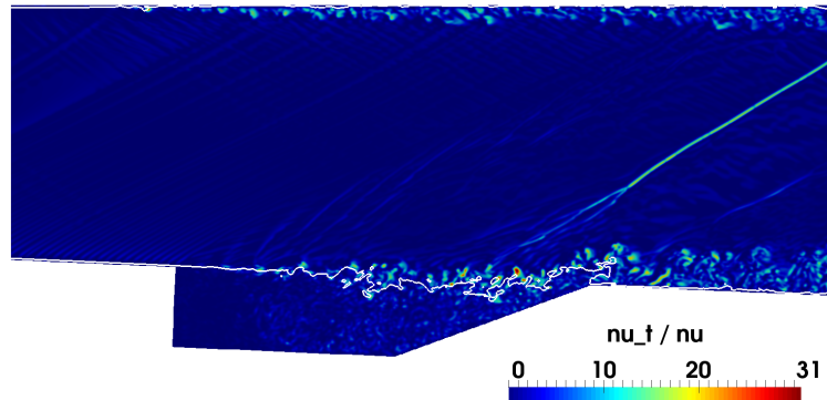
Figure 4.17: Instantaneous field subgrid viscosity adimensionalized by laminar viscosity \nu_t/\nu for fine mesh. The isoline Mach = 1 is displayed with a white line.
