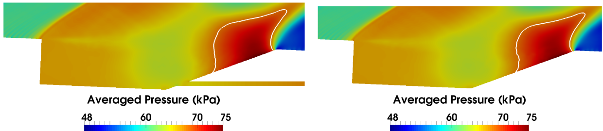
Figure 5.29: Averaged pressure fields in the injector centerplane (left) and the centerplane between two injectors (right). The isoline P = 68 kPa is displayed with a white line. Fine mesh.
