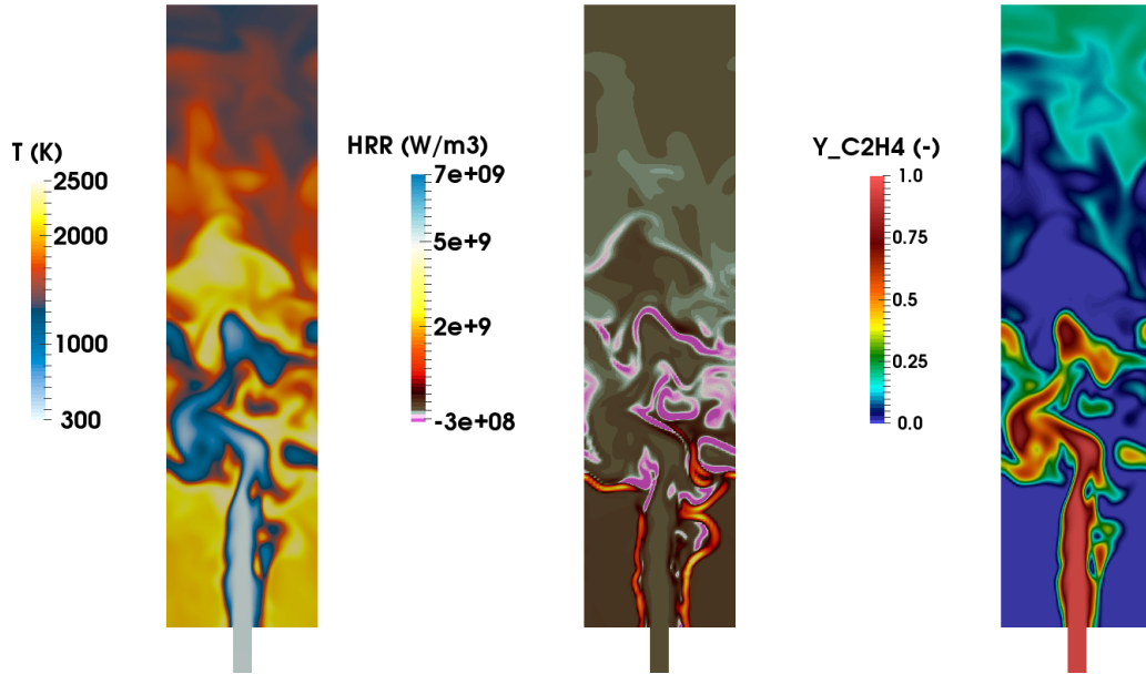
Figure 1: Instantaneous temperature, heat release rate and fuel mass fraction at y = -19.57 mm (injector center) for RCA1. Coarse mesh.
