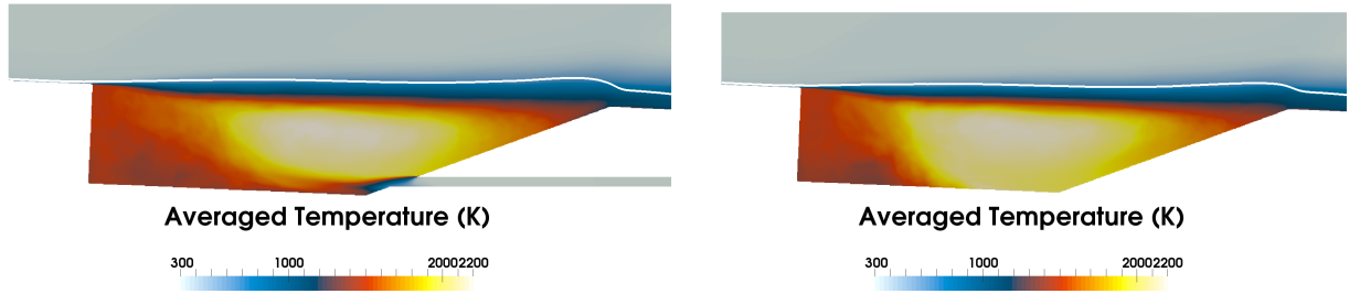
Figure 5.28: Averaged temperature fields in the injector centerplane (left) and the centerplane between two injectors (right). The isoline Mach = 1 is displayed with a white line. Fine mesh.
