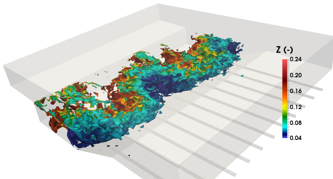
Figure 5.52: Instantaneous isosurface of temperature at 2000 K for RCA11, colored by the values of mixture fraction.
