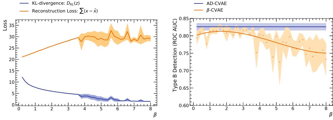
FIGURE 6.9: The final loss function values for a \beta -CVAE (left) and results of the type B detection problem for the synthetic data set as a function of varying \beta (right). The experiment was run five times for each of the chosen \beta values. The orange bands correspond to the standard deviation of the results. The dots correspond to the mean and the solid line to a polynomial fit of the means. The AD-CVAE ROC AUC stays constant as the training procedure does not depend on \beta hyper-parameter (see the loss in equation 6.4).
