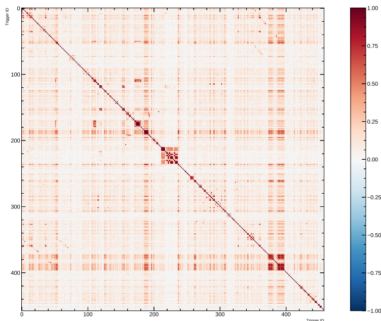
FIGURE 6.1: Correlations between 458 HLT rates of LHC fill 6291 of Run 2. The calculation is performed after correction for down-trend of all trigger rates using first differences.
