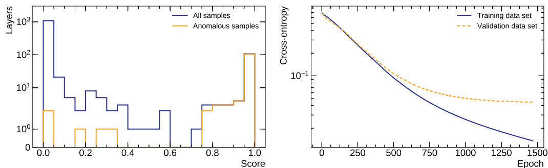
FIGURE 4.5: The distribution of scores (left), and the loss function as a function of the number of training epochs (right) for the CNN model used in the local approach.
