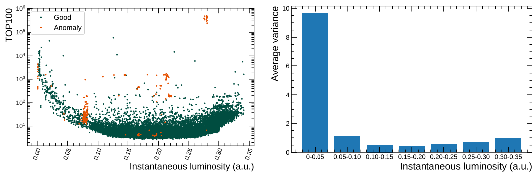
FIGURE 5.4: Anomaly score w.r.t. instantaneous luminosity (left) of sparse autoencoder and the average feature spread in different instantaneous luminosity regions (right).
