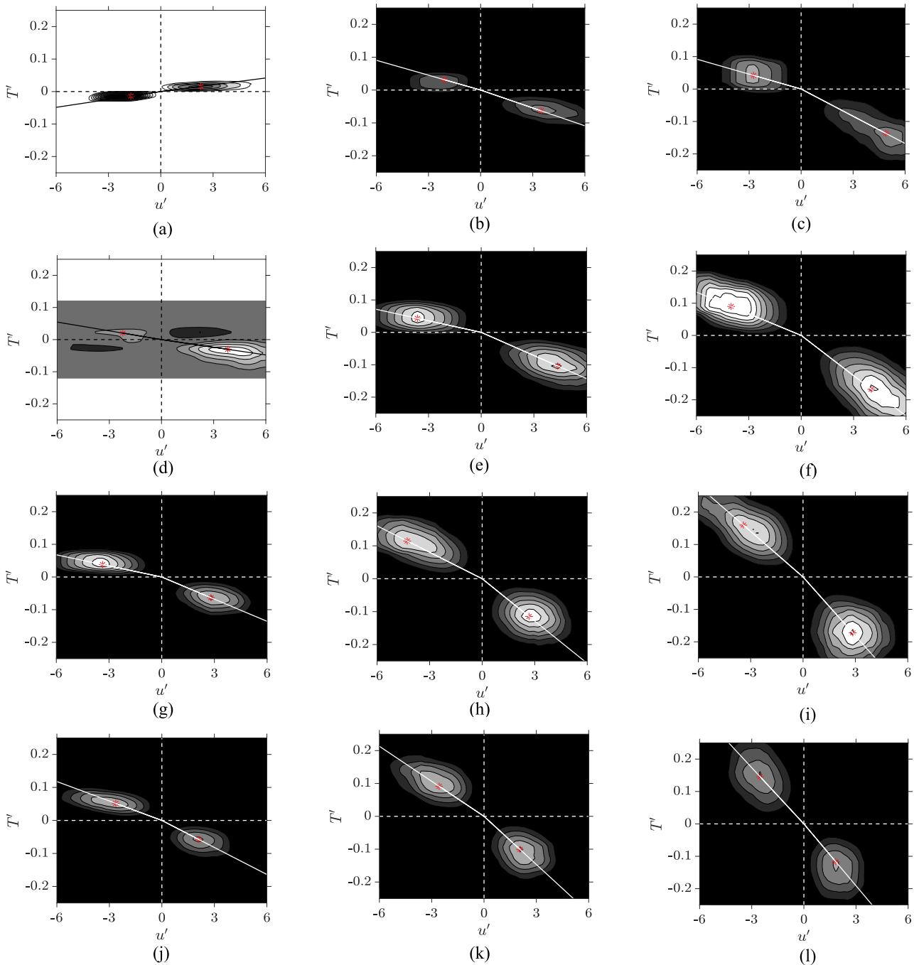
Fig. 12. Contours of the covariance integrands of the u' and T' for y^+ = 5 ((a)–(c)), 10 ((d)–(f)), 35 ((g)–(i)) and 90 ((j)–(l)). Here the first, second and third columns represent the cooled, adiabatic and heated walls, respectively. The colors of the contour levels vary from 2 to 9 (light to dark) for (a), from -5 to 2, excluding the zero level for (d) and from -16 to -4 for the rest. (For interpretation of the references to color in this figure legend, the reader is referred to the web version of this article.)
