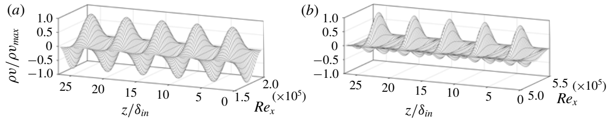
FIGURE 13. 3-D representation of control strip functions at (a) FSC, and (b) SCS for C52Cn and C52Ch.
