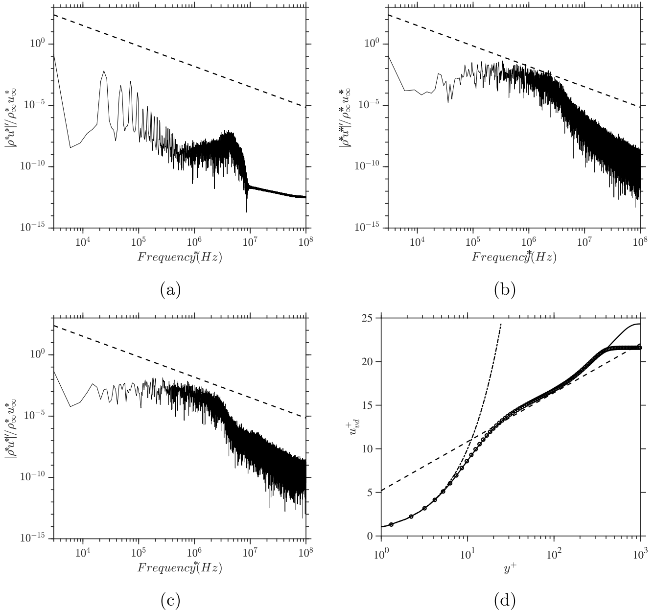
Fig. 4. Frequency spectra of |\rho^* u^{*'}| / \rho_{\infty}^* u_{\infty}^{*} for the adiabatic wall at (a) Re_x = 3.02 \times 10^6 , (b) Re_x = 3.94 \times 10^6 , (c) Re_x = 5.40 \times 10^6 ; where (—) represents the (-5/3) law of turbulence decay, and (d) Van-Driest transformed mean velocity profile for the adiabatic case compared with (Shadloo et al., 2015) (symbols) at Re_x = 5.40 \times 10^6 , where (—) is (1/0.41 \log y^+ + 5.2) and (— · —) is u_{vd}^+ = y^+ .
