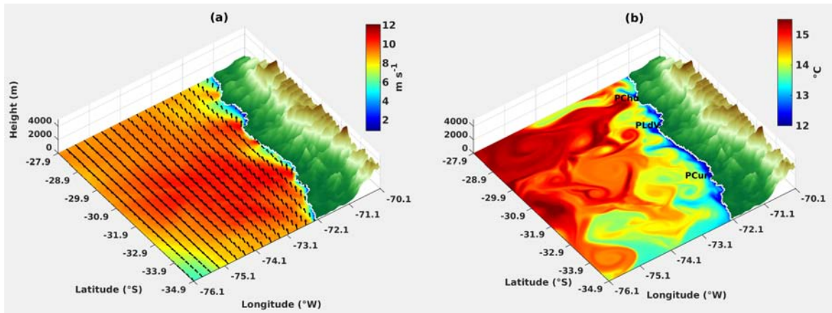
Figure 1.16. Map illustrating the main features of the surface circulation off central Chile (spring 2008), as simulated by the regional atmospheric (WRF) and oceanic (ROMS) models: (a) Surface wind magnitude/direction ( \text{m s}^{-1} ) and (b) Sea surface temperature ( ^{\circ}\text{C} ). In addition, acronyms indicate upwelling centers( PCho: Punta de Choros, PLdv: Punta Lengua de Vaca and PCur: Punta Curaumilla. From Astudillo et al. (2018), submitted, see Chapter 4.
