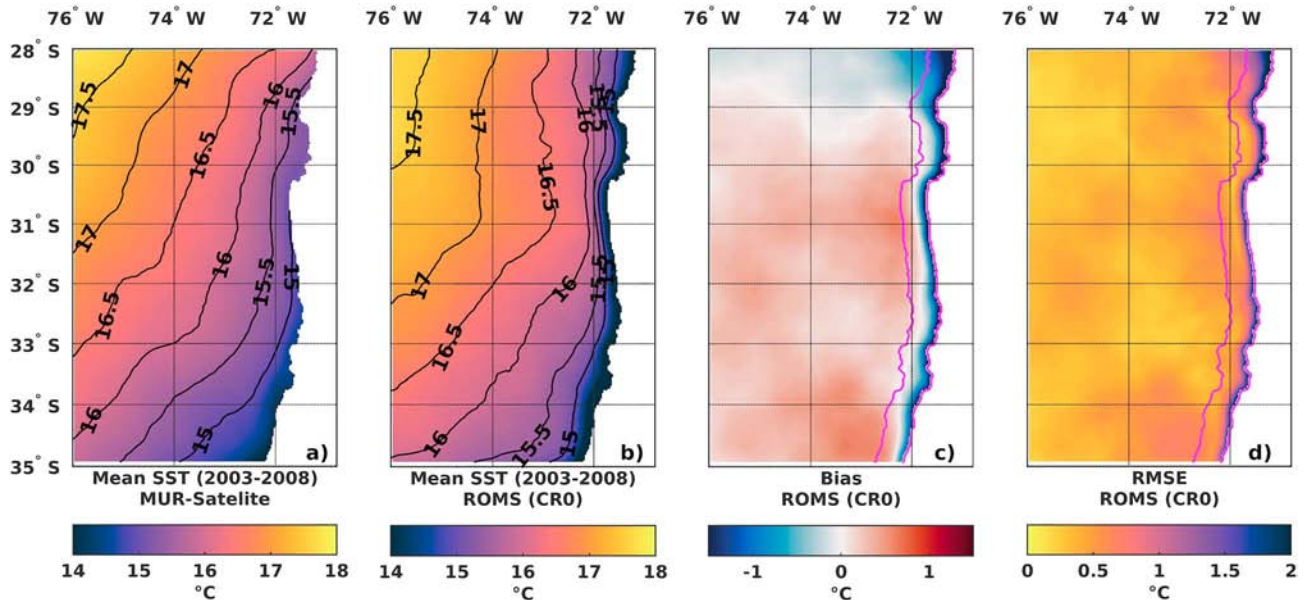
Figure A3. Spatial maps of the temporal mean of the SST ( ^{\circ}\text{C} ) over the period 2003–2008 from (a) MUR data and simulated by (b) ROMS CR0. (c) mean bias ( ^{\circ}\text{C} ), and (d) RMSE ( ^{\circ}\text{C} ) for the monthly seasonal differences between CR and MUR data. The lines in magenta indicate the limit of the 50-km coastal band and the shoreline. SST = Sea Surface Temperature; MUR = Multi-scale Ultra-high Resolution; ROMS = Regional Ocean Modeling System; RMSE = Root Mean Square Error.
