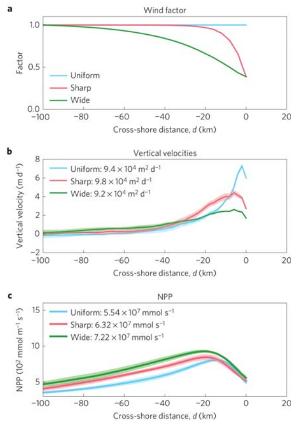
Figure 1.22. Impact of wind drop-off on total upwelling and NPP in the CalCS between 38° N and 43° N during spring (April-June). (a), Coastal wind profile factor applied to the wind product. (b), Mean vertical velocity at 70 m depth. (c), NPP integrated over the photic zone (0–70 m depth). The shaded areas represent the standard deviations. The means and standard deviations are estimated using 8 years of simulations. From Renault et al. (2016a).
